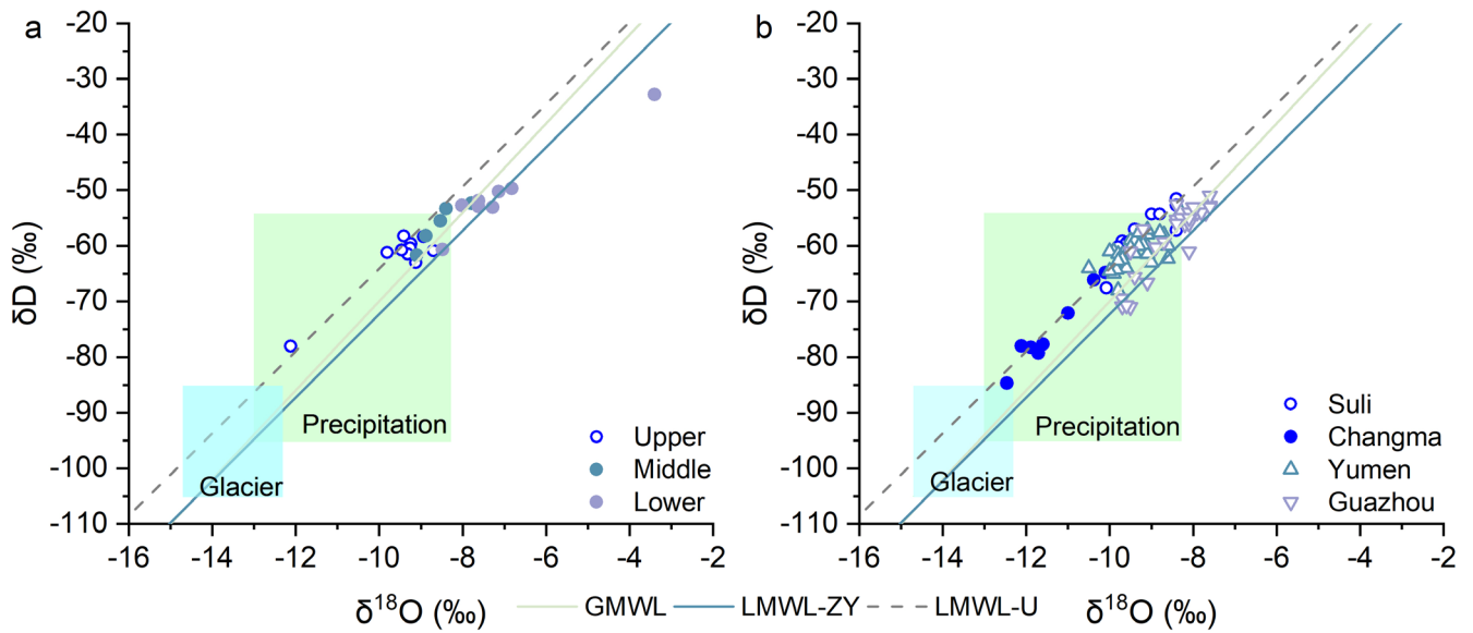
330 Figure 8: \delta D and \delta^{18}O relationships of river water (a) and groundwater (b) in the Shule River Basin, including previously published groundwater data (Xie et al., 2022; Wang et al., 2015; He et al., 2015), plotted against the Global Meteoric Water Line (GMWL), the local meteoric water line in the upper reaches (LMWL-U), and that in the middle and lower reaches (LMWL-ZY). The pale green rectangle denotes the \delta D and \delta^{18}O range of precipitation in the upper basin, while the pale blue rectangle denotes the \delta D and \delta^{18}O range of glacier meltwater (Guo et al., 2022).
