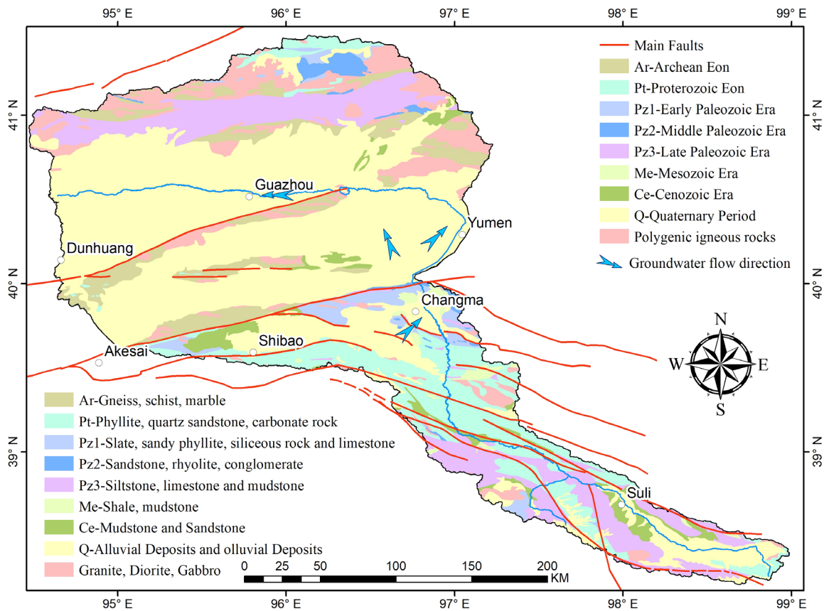
135 Figure 2: Geological-stratigraphic distribution, structural framework, and hydrogeological sketch map of the study area (modified 140 from the 1:1,000,000 Geological Map of Gansu Province, Gansu Geology Survey 1978~1980).
