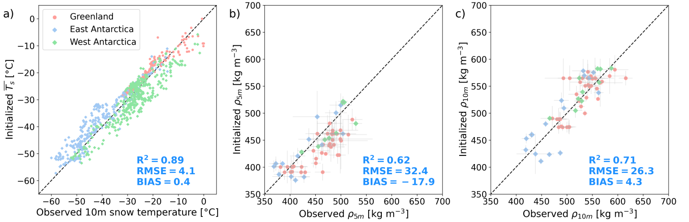
Figure 2. (a) Mean surface temperature \overline{T}_s obtained from the initialization procedure represented as a function of the observed 10 m snow temperature. (b, c) Initialized snow density at 5 m (b) and 10 m (c) depth versus observed densities at 5 m (b) and 10 m (c) across Greenland, East Antarctica, and West Antarctica. Statistical indicators (correlation coefficient R^2 , RMSE, and bias) are reported in blue. Locations in Greenland, East Antarctica, and West Antarctica are marked in red, cyan, and green respectively. Error bars represent observational uncertainties (see Supplementary).
