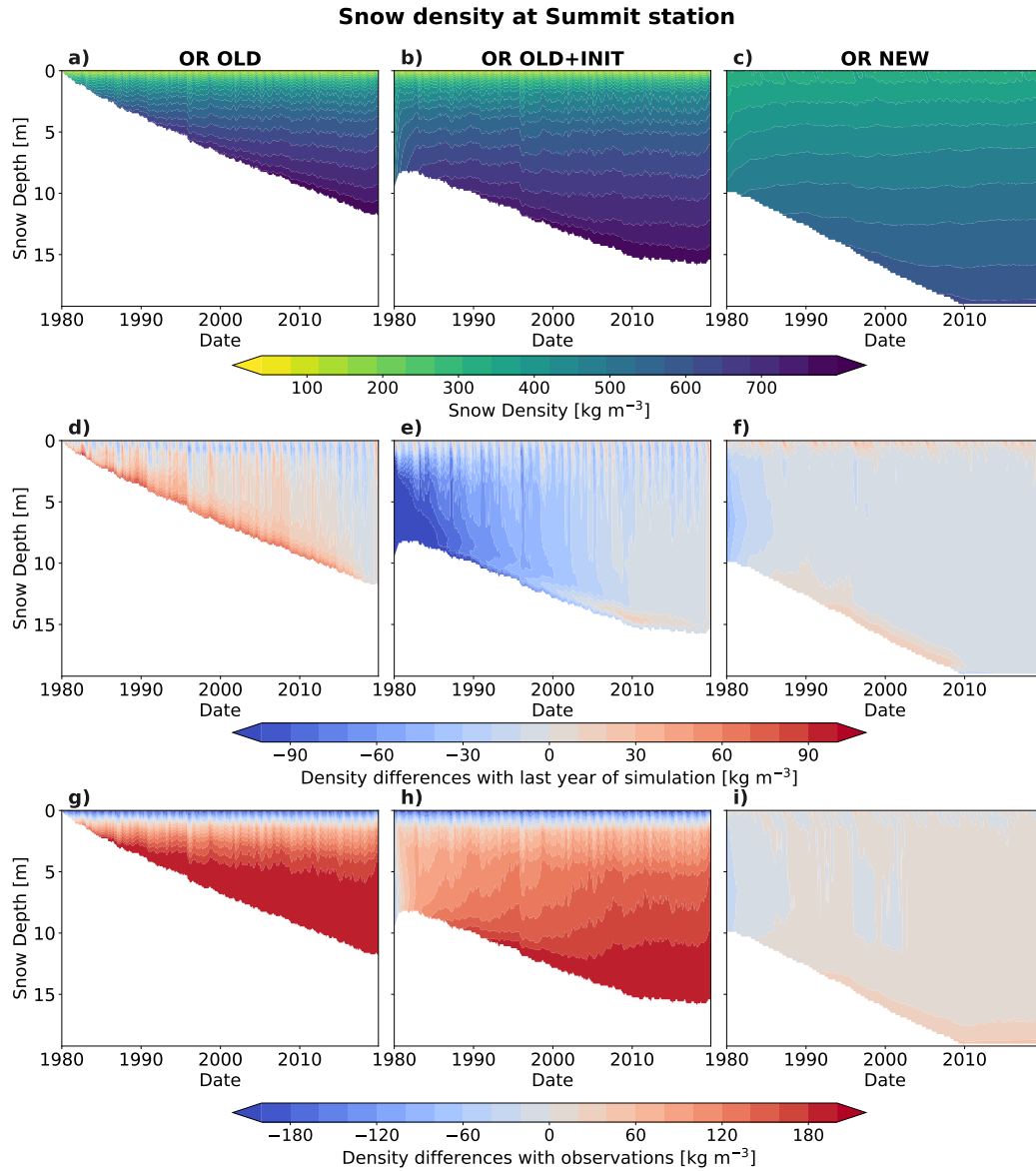
Figure 8. Monthly evolution of (a, b, c) the modeled snow density at Summit; (d, e, f) the density differences between modeled snow density and the final year averaged (2019) simulated profile, interpolated over the model snow depth at Summit for each month; and (g, h, i) the density differences between monthly simulated profiles and an observed density profile derived from a third-degree polynomial fit. The results are shown for three model configurations: (left) OR OLD, the previous version of ORCHIDEE, (middle) OR OLD+INIT with the initialization procedure activated, and (right) OR NEW, the final configuration with the initialization combined with the densification developments.
