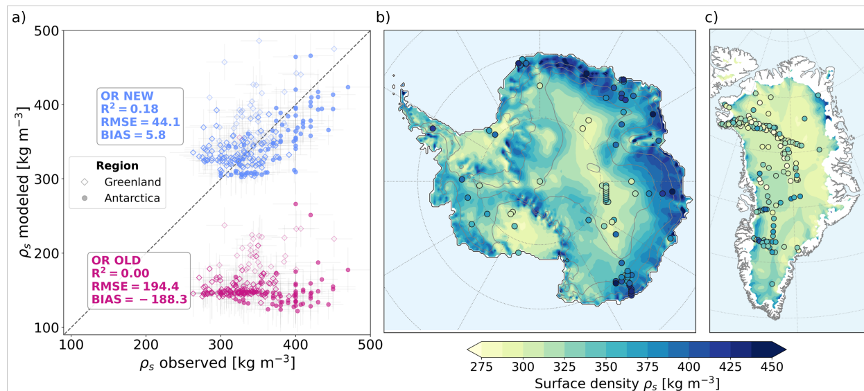
Figure 5. (a) Comparison of 40 years averaged (1980-2019) modeled surface snow density (computed as the average density of the top 20cm of the snowpack) with observed surface snow density from Greenland (open diamond) and Antarctica (solid circle). Model results are shown for the previous ORCHIDEE formulation (OR OLD, purple; Pahaut, 1976) and the new formulation (OR NEW, blue). Error bars represent observational uncertainties (see Supplementary). (b, c) Spatial comparison of 40 years averaged modeled surface snow density with observations (in dots) in Antarctica (b) and Greenland (c).
