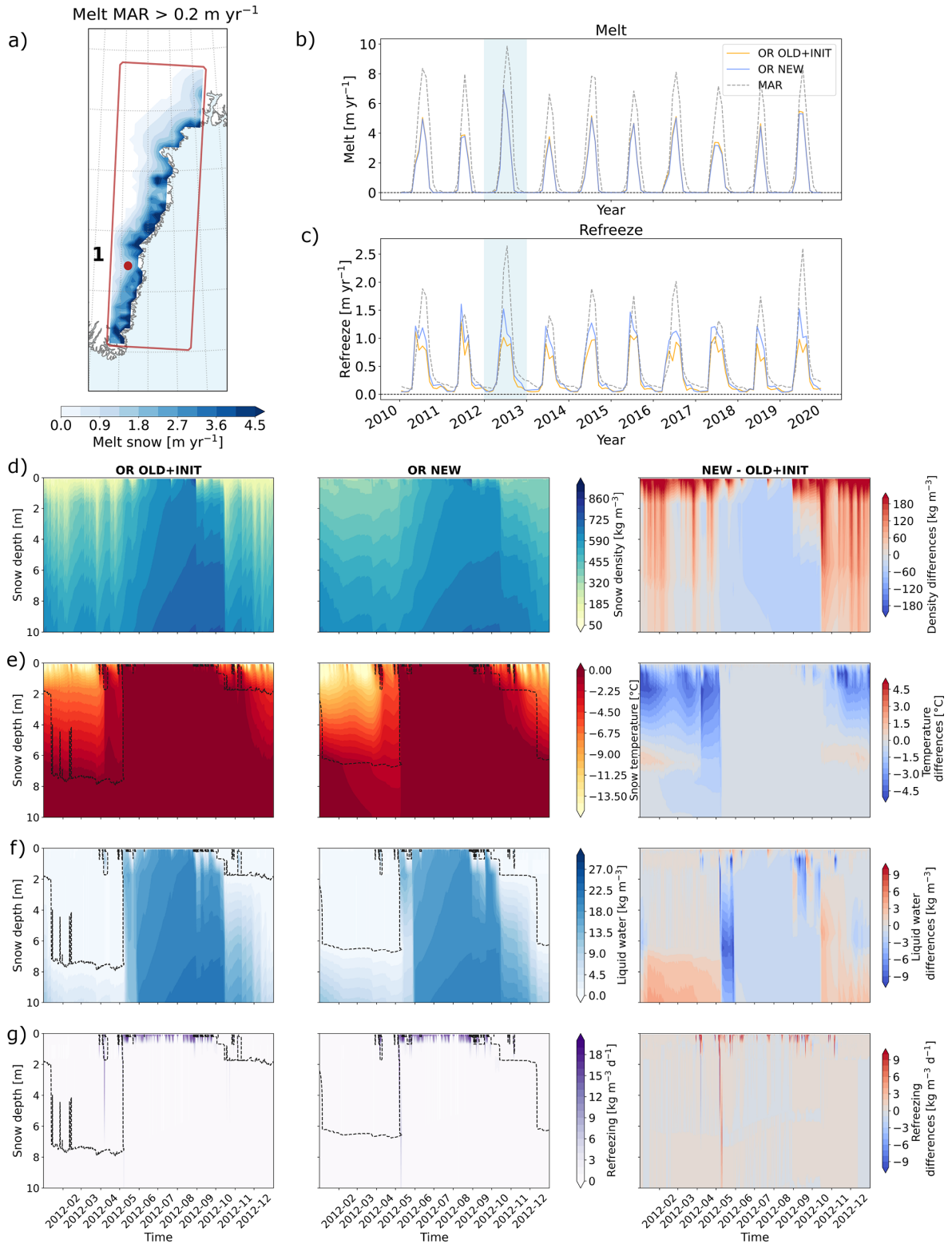
Figure 10. (a) Average melt from the MAR model over the southeast coast of the GrIS, where melt exceeds a threshold of 0.2 \text{ m yr}^{-1} . (b, c) Mean seasonal melt and refreezing rates ( \text{m yr}^{-1} ), averaged over the region shown in (a). Results are presented for OR OLD + INIT (orange), OR NEW (blue), and MAR (dashed lines). The ORCHIDEE simulations were run using the OPT12L albedo parameters. The year 2012 is highlighted in light blue. (d–g) Simulated snow density (d), snow temperature (e), liquid water content (f), and refreezing (g), modelled with ORCHIDEE OLD + INIT (left), ORCHIDEE NEW (centre), and their differences (OR NEW – OR OLD + INIT, right). In panel (e–g), the black dotted line represent the threshold where liquid water is present or not in the snowpack.
