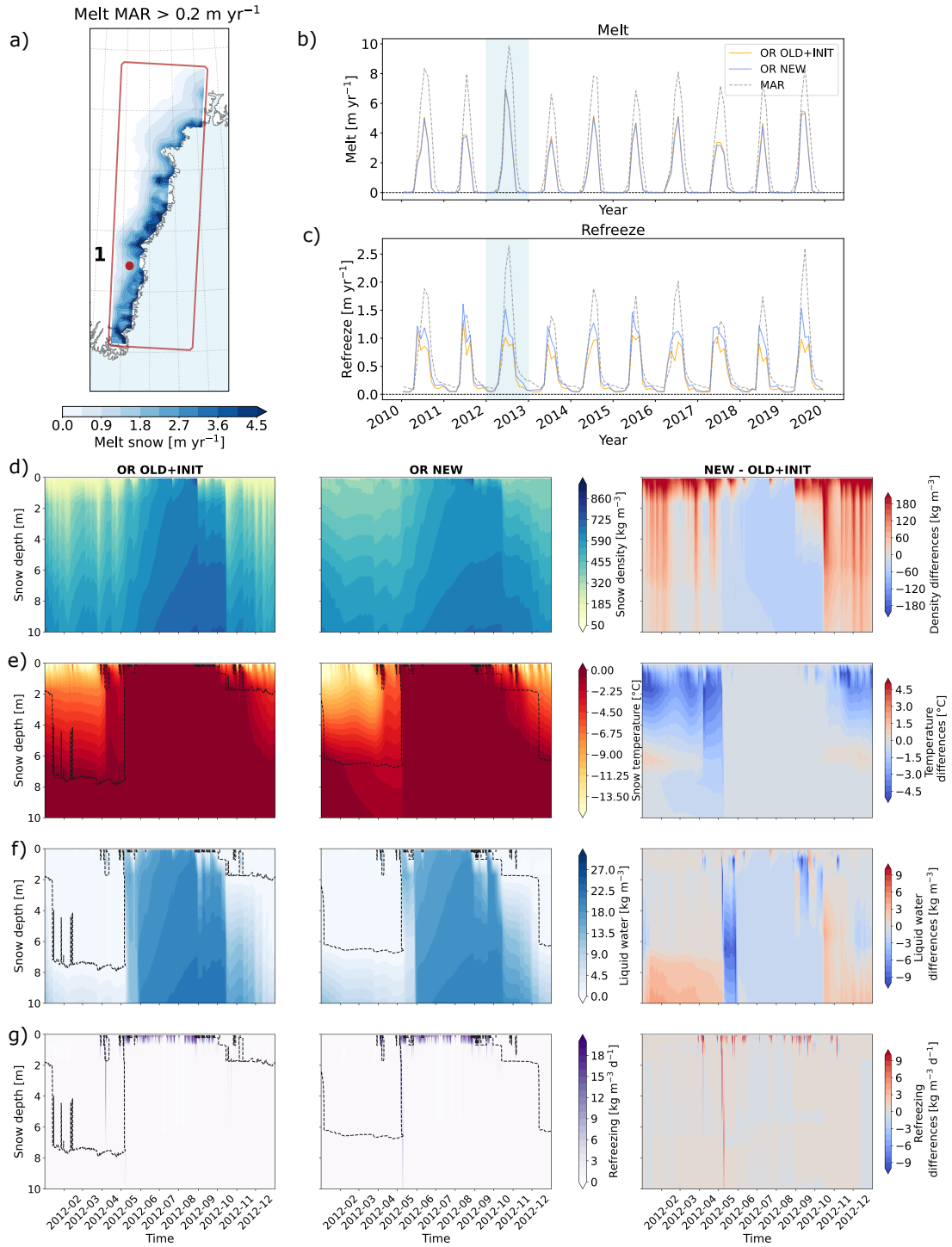
Figure 10. (a) Average melt from the MAR model over the southeast coast of the GrIS, where melt exceeds a threshold of 0.2 \text{ m yr}^{-1} . (b–c) Mean seasonal melt and refreezing rates ( \text{m yr}^{-1} ), averaged over the region shown in (a). Results are presented for OR OLD+INIT (orange), OR NEW (blue), and MAR (dashed lines). The ORCHIDEE simulations were run using the OPT12L albedo parameters. The year 2012 is
