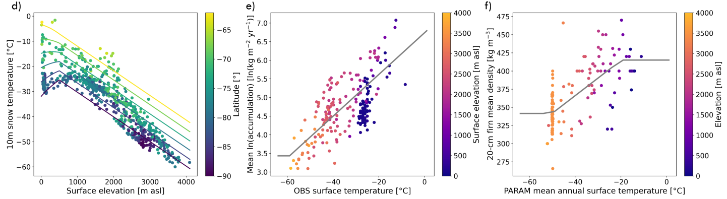
Figure A2. Observed 10 m snow temperature in function of surface elevation and latitude in Greenland (a) and Antarctica (d). Colored lines represent the parameterization of mean annual surface temperature in function of latitude and elevation. Logarithm accumulation observations in function of the parameterized mean annual surface temperature and surface elevation in Greenland (b) and Antarctica (e). Grey line show the final parameterization in function of the parameterized mean annual surface temperature. Surface density observations in function of the parameterized mean surface temperature and surface elevation in Greenland (c) and Antarctica (f). Grey line shows the parameterized surface density in function of the parameterized mean annual surface temperature.
