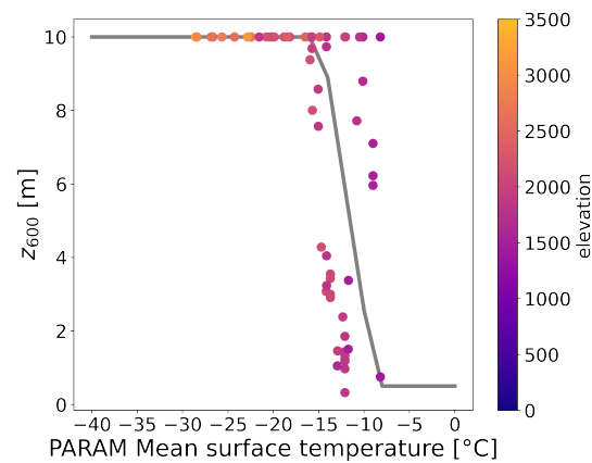
Figure A1. Observed snowpack thickness at which 600\text{ kg m}^{-3} is reached ( z_{600} ) as a function of the parameterized mean surface temperature and surface elevation, in Greenland. The grey line represents the parameterization of mean snowpack thickness as a function of the parameterized mean surface temperature.
