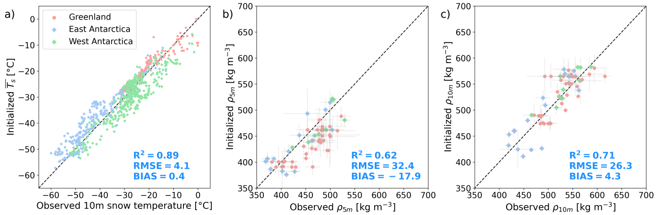
Figure 2. (a) Mean surface temperature \overline{T}_s obtained from the initialization procedure represented as a function of the observed 10 m snow temperature. (b, c) Initialized snow density at 5 m (b) and 10 m (c) depth versus observed densities at 5 m (b) and 10 m (c) across Greenland, East Antarctica, and West Antarctica. Statistical indicators (correlation coefficient R^2 , RMSE, and bias) are reported in blue. Locations in Greenland, East Antarctica, and West Antarctica are marked in red, cyan, and green respectively. Error bars represent observational uncertainties (see Supplementary).
