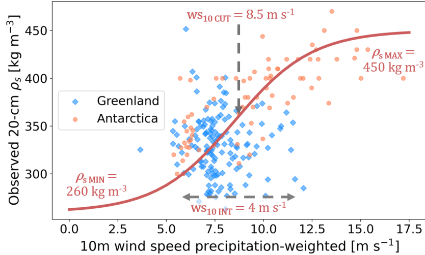
370 Figure 3. Observed mean surface snow densities in the upper 20 cm of the snowpack represented as a function of the climatological average (1980-2019) of the 10 m wind speed simulated by MAR and weighted by the amount of snowfall during the same period. Observations are presented in blue for Greenland and orange for Antarctica. The red line represents the wind speed parameterization of surface snow density presented in this study.
