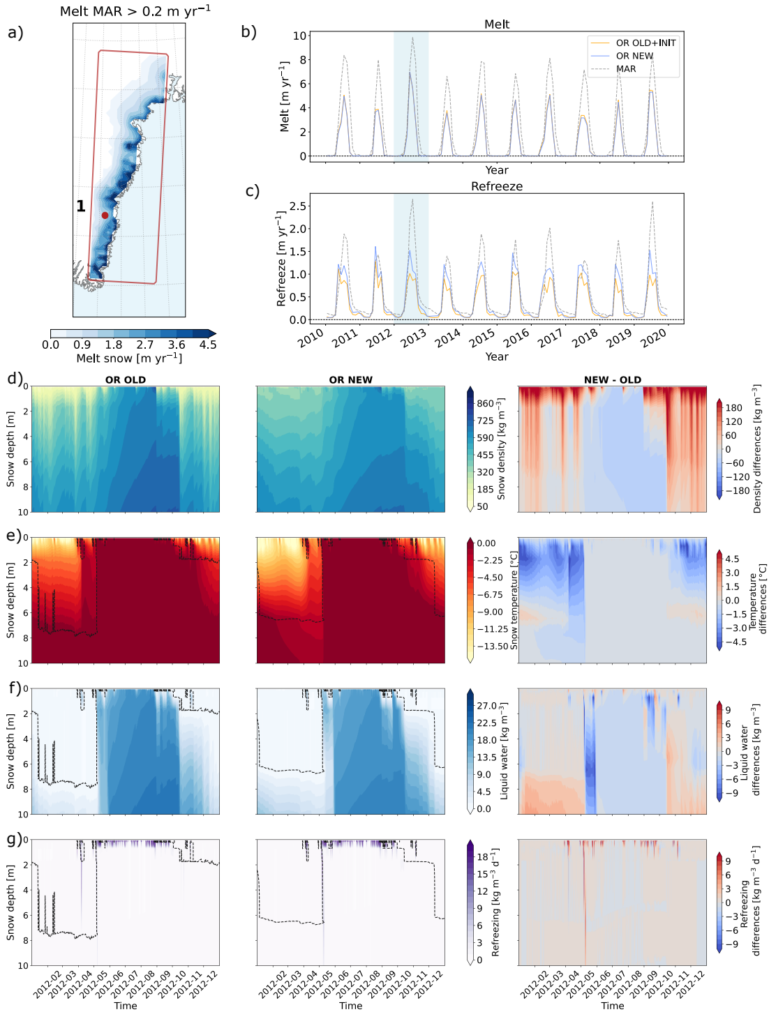
Figure 10. (a) Average melt from the MAR model over the southeast coast of the GrIS, where melt exceeds a threshold of 0.2 \text{ m yr}^{-1} . (b–c) Mean seasonal melt and refreezing rates ( \text{m yr}^{-1} ), averaged over the region shown in (a). Results are presented for OR OLD+INIT (orange), OR NEW (blue), and MAR (dashed lines). The year 2012 is highlighted in light blue. (d–g) Simulated snow density (d), snow
