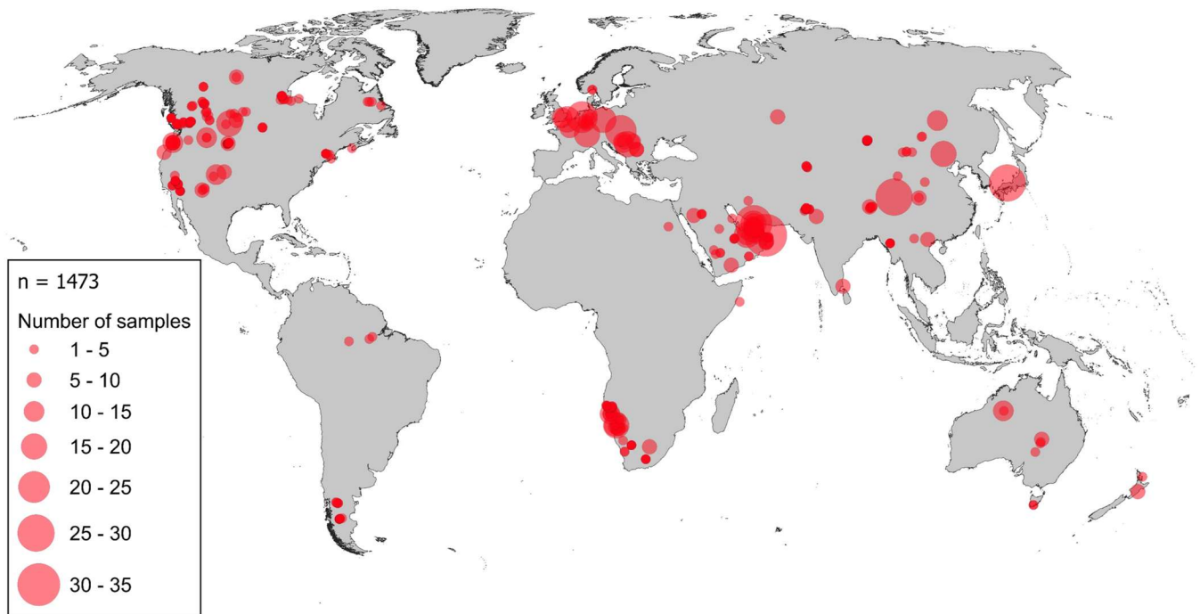
Figure 2: Map of the sedimentary radionuclide samples compiled within the training dataset used in this study.
