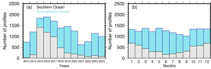
1120 Figure S1: Time distribution of the selected set of BGC-Argo profiles over (a) years and (b) months.
