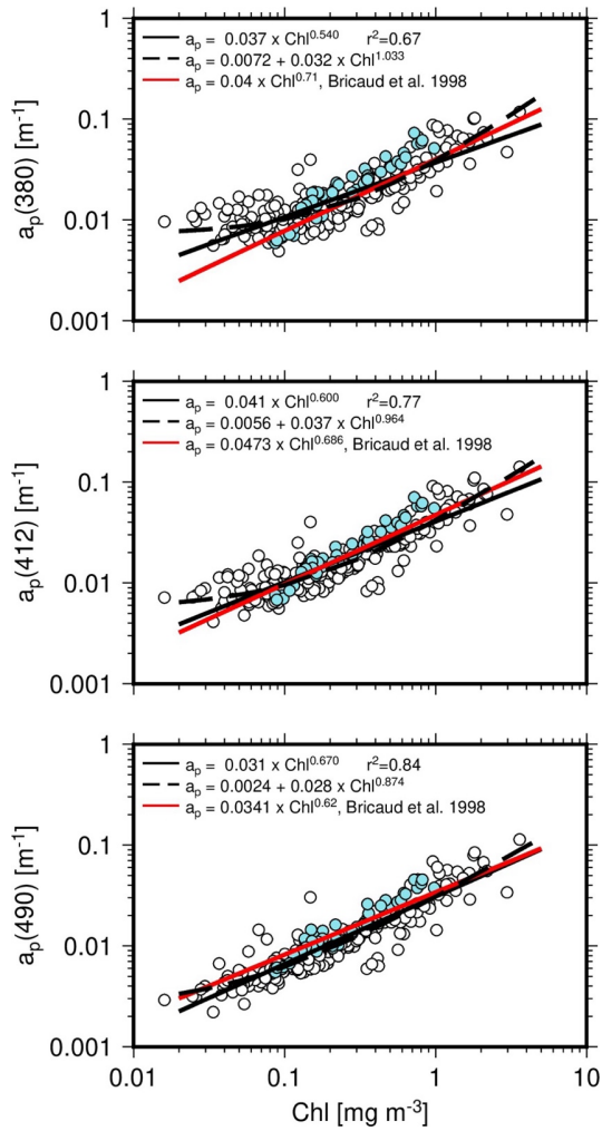
1150 Figure S4: Particulate absorption coefficient at the three wavelengths indicated as a function of Chl. The data are from the ACE (open dots) and SOLACE (turquoise) research voyages. The solid black lines are linear fits on the log-transformed data. The dashed black lines are non-linear fits (Eq. 5) on the same data. The red lines are the parameterization from Bricaud et al., (1998).
