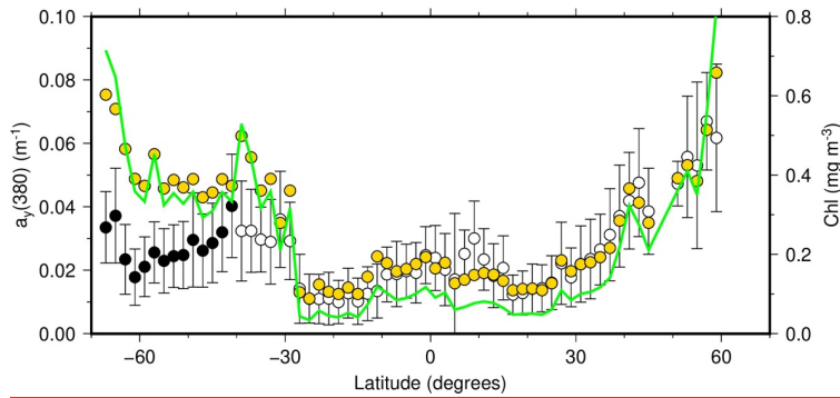
Figure 3: Zonal averages and standard deviation of a_y(380) for 2-degree latitude bands, calculated across our entire data set (black symbols for latitudes < 40° S). The gold symbols are the a_y(380) estimated from the MG09 relationship for the average Chl values (green curve, with no standard deviation plotted for clarity of the plot).
