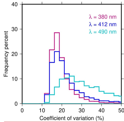
605 Figure 9: Distribution of the coefficient of variation of a_y(\lambda) values obtained by running the Monte Carlo analysis on each of the individual estimates of K_d(\lambda) .
