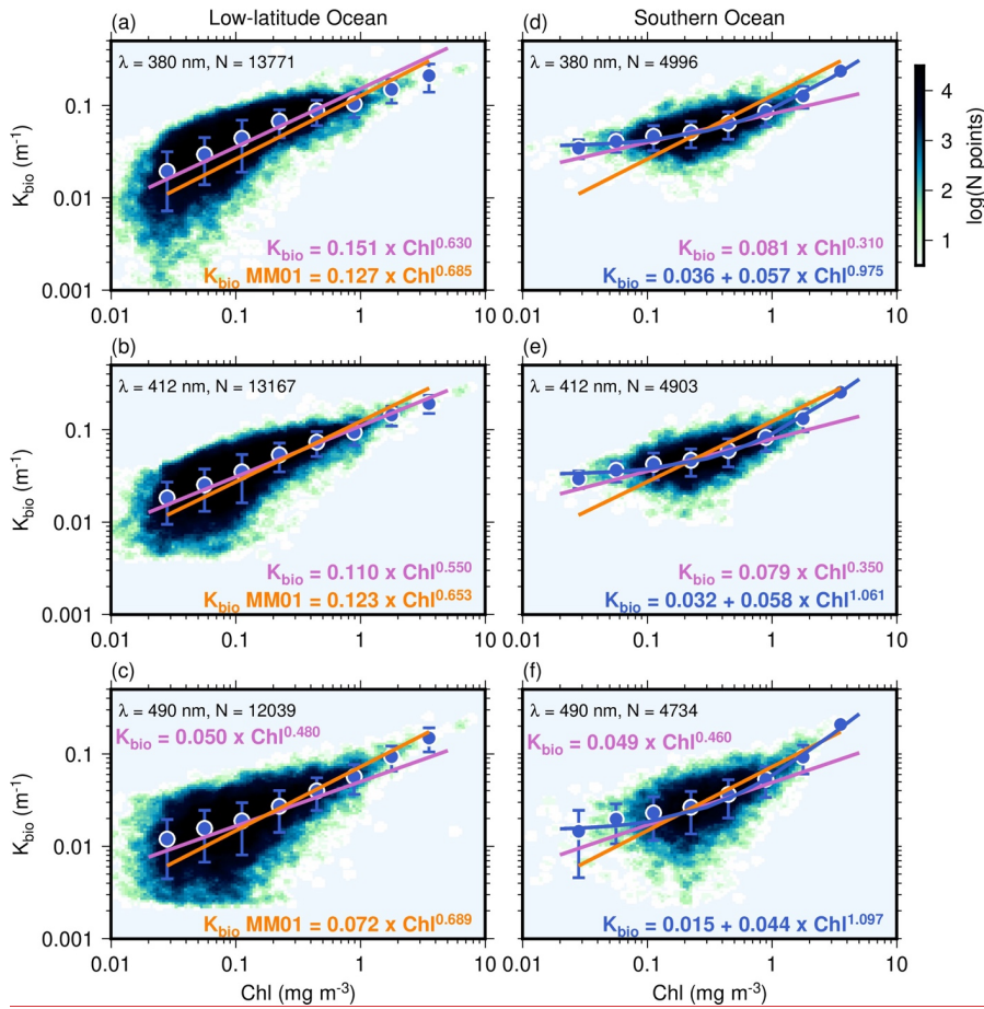
Figure 4: Non-water diffuse attenuation coefficient for downward irradiance ( K_{bio} ) for the three wavelengths indicated in the panels for the low-latitude oceans (left) and the SO (right) data sets. The blue-coloured density plots (scale on the top right) are built from all data obtained from individual float profiles. The large blue dots circled in white and vertical bars are average values and their standard deviation calculated over logarithmically equal Chl intervals. The purple and dark blue solid lines are a linear and a non-linear fits to all data points (log-transformed data; equations provided on each panel). The orange line for both the low-latitude oceans and the SO are for the Morel and Maritorena (2001) model (reported on the left panels as the " K_{bio\_MM01} " equation).
