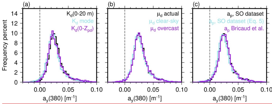
Figure 8: Distribution of a_y(380) resulting from (a) three approaches to obtain K_d from E_d(z, 380) , (b) whether the distinction between clear and cloudy sky is applied when calculating \mu_d , or ignored and then \mu_d being forced to either its clear sky or overcast sky value, and (c) using the three different a_p vs. chl relationships displayed in Fig. S4. Data for the SO only.
