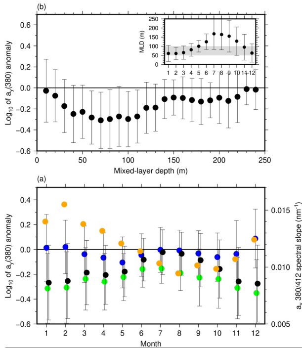
525 Figure 6: (a) monthly average values (dots) and standard deviations (vertical bars) of a_y anomalies as a function of month of year (left scale). The anomalies are expressed as the decimal logarithm of the ratio of observed to modelled a_y , where the modelled values are from Morel and Gentili (2009). The blue dots are for Chl < 0.2 mg m -3 , the green dots for Chl above that threshold, and the black dots for all data. The orange dots are the monthly average values of the spectral slopes calculated between 380 and 412 nm (right scale). (b) The same anomalies as in (a) plotted as a function of the mixed-layer depth (MLD), with the insert showing the seasonal course of the MLD in our data set. The greved area shows MLD values between 50 and 100 m, corresponding to the largest negative anomalies. 530
