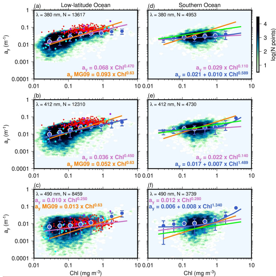
470 Figure 5: CDOM absorption ( a_y ) for the three wavelengths indicated and for the low-latitude waters (left) and the SO (right) data sets. The blue-coloured density plots (scale on the top right) are built from all data obtained from individual float profiles. The large blue dots circled in white and vertical bars are average values and their standard deviation calculated over logarithmically equal Chl intervals. The purple and dark blue curves are a linear and non-linear fits to all data points (log-transformed data), the orange lines are from the Morel and Gentili (2009) model, whose equations are also
