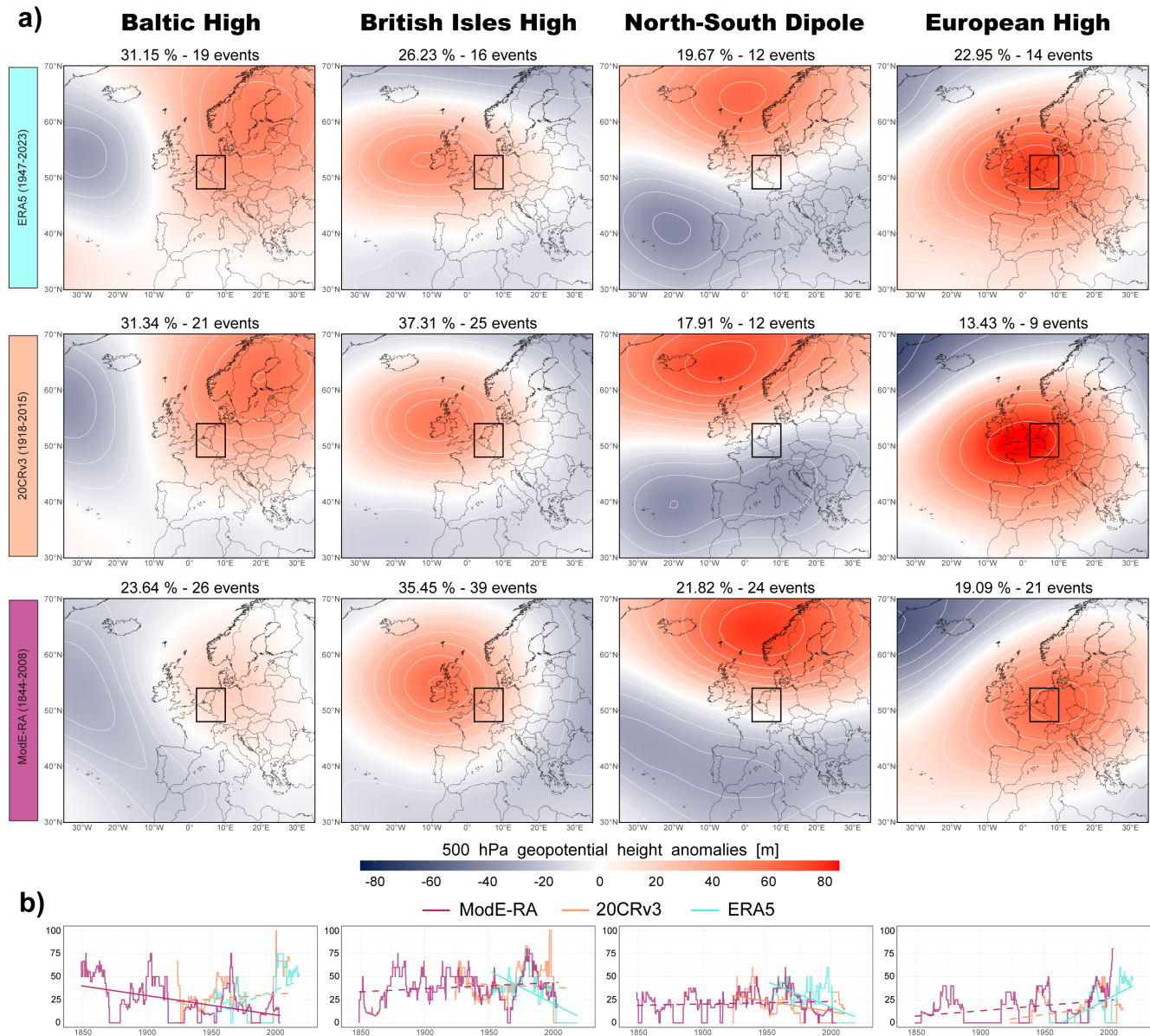
Figure 5: Atmospheric circulation patterns associated with SPEI-3 drought events and their temporal changes. (a) Cluster centroids of 500 hPa geopotential height anomalies (reference period: 1947–2008) for each period–reanalysis combination. Values above each map indicate the percentage and absolute number of drought events assigned to the corresponding cluster within each
