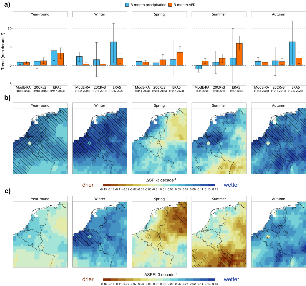
Figure 4: (a) Trends in 3-month precipitation and AED for each period–reanalysis combination, estimated using Sen’s slope and expressed per decade. Trends were assessed both year-round, considering all monthly values, and seasonally. Error bars indicate the 95% confidence intervals of Sen’s slope, accounting for the variance correction approach of Hamed and Rao (1998). (b–c) Sen’s slope maps of year-round and seasonal SPI-3 (b) and SPEI-3 (c) trends over 1947–2023 (ERA5), expressed per decade. Discs
