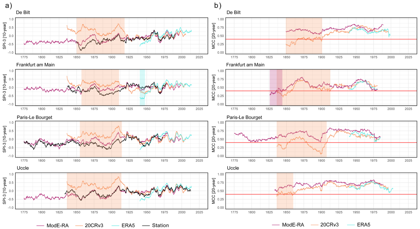
Figure 1: Data evaluation: time series of (a) the 10-year left-moving average of SPI-3, for the four reference stations (De Bilt, Frankfurt am Main, Paris-Le Bourget, Uccle) and the reanalyses, and (b) the 20-year left-moving Matthews correlation coefficient (MCC) for drought classification between each reference station and the reanalyses. For each reanalysis–station pair in (a), the shaded period begins when the 10-year left-moving mean absolute error exceeds 0.5 and extends until it subsequently decreases below 0.5 and remains below this threshold. In (b), the shaded period begins when the 20-year left-moving MCC falls below 0.4 and extends until it subsequently rises above 0.4 and remains above this threshold. In both panels, shaded areas are coloured according to the dataset considered unreliable during the corresponding periods.
