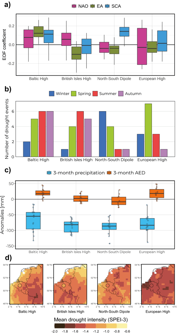
Figure 6: Characteristics of the atmospheric circulation patterns identified from SPEI-3 drought-based clustering over 1947–2023 (ERA5), pooling all drought events across seasons and years. (a) Boxplots of EOF coefficients from seasonal EOF analyses of the
