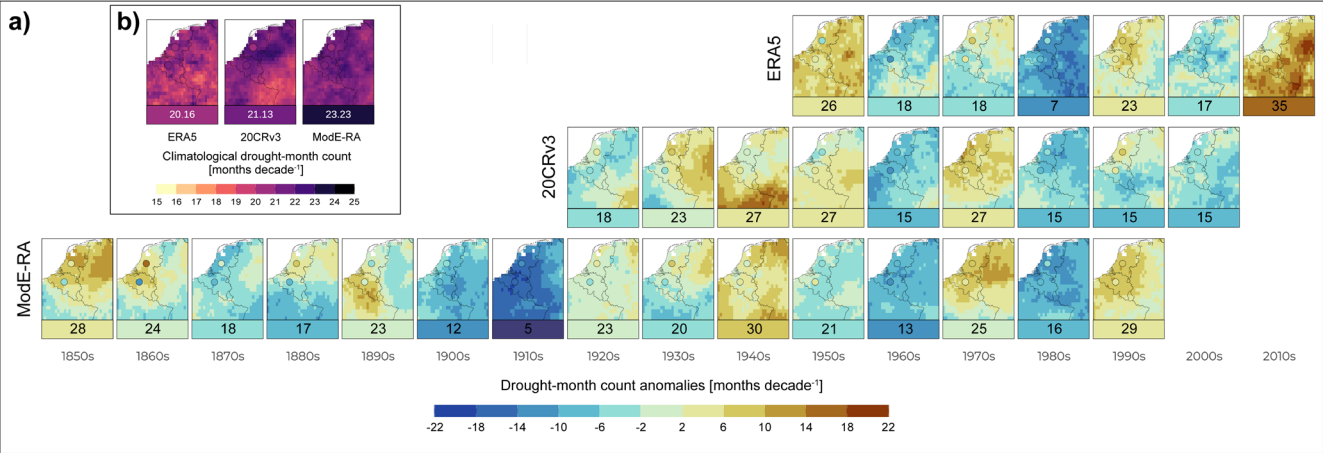
Figure 3: (a) Anomalies in the number of SPEI-3 drought months per decade for each dataset (rows), shown for decades fully covered by the corresponding datasets (columns), relative to (b) the mean number of SPEI-3 drought months per decade over the 1947–2008 reference period. In both (a) and (b), the absolute number of drought months at the regional scale is shown below each map. Discs represent values at weather stations that fully cover both the corresponding decade and the reference period.
