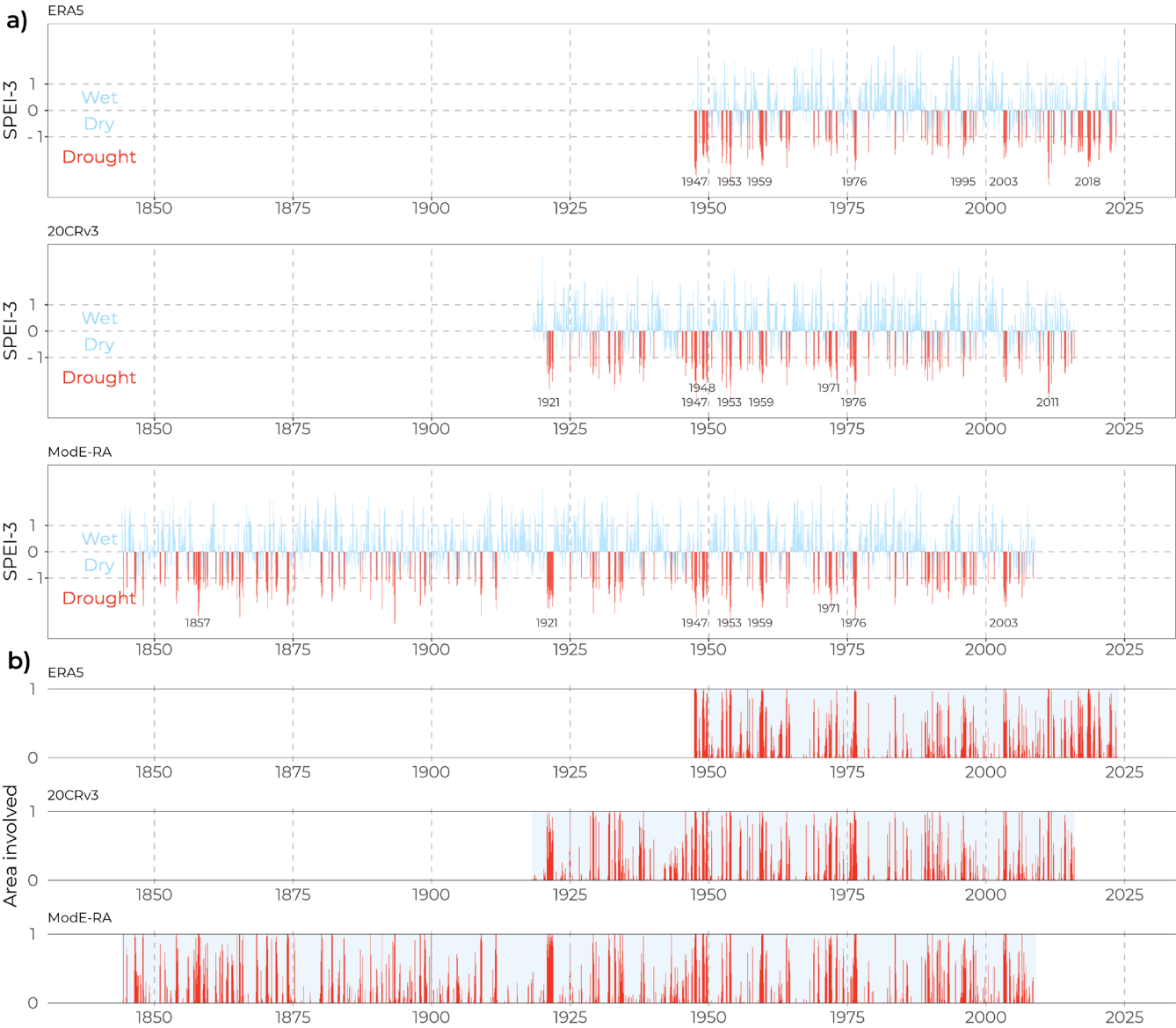
200 Figure 2: (a) 3-month Standardized Precipitation Evapotranspiration Index time series for the aggregate western Central Europe region for each reanalysis dataset (each row) (reference period: 1947–2008). The red bars indicate drought months (SPEI-3 < -1), and the most severe drought events are highlighted. (b) Time series of the proportion of the western Central Europe region under drought (illustrated in red) according to the SPEI-3 values of the grid cells.
