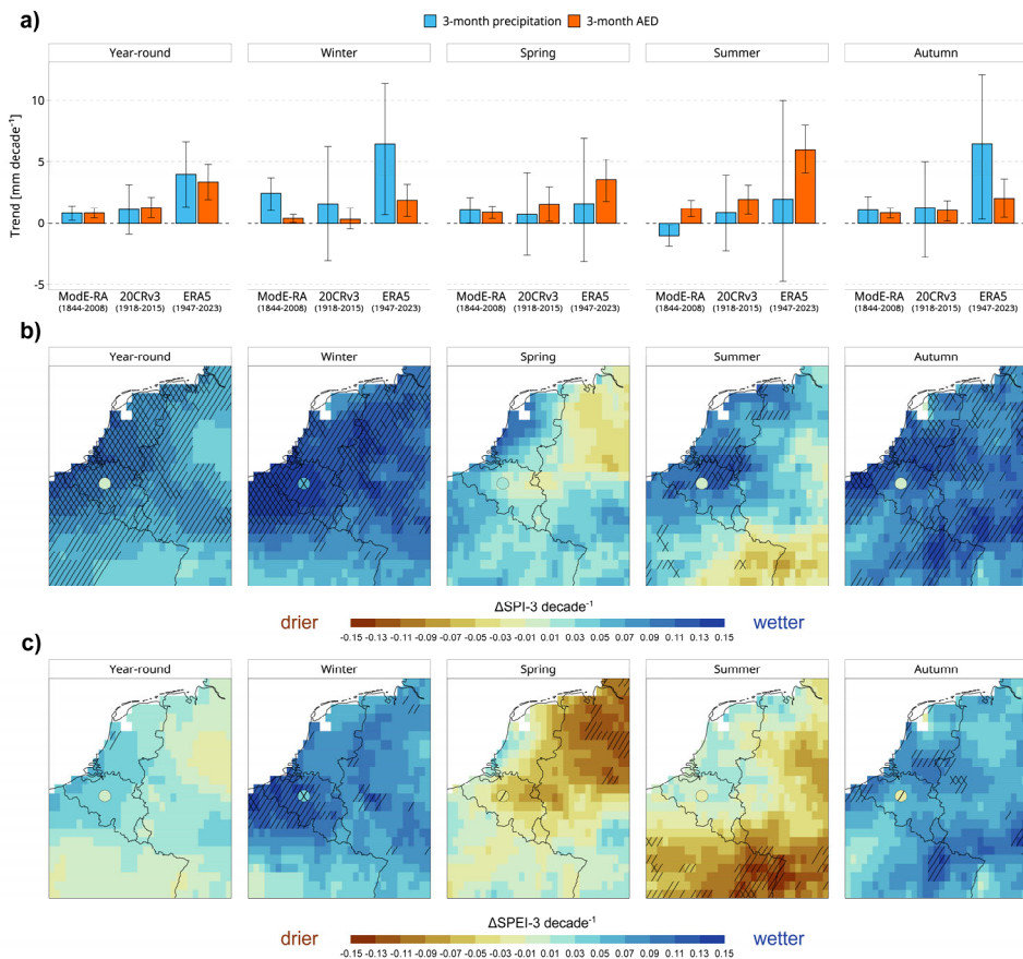
Figure 4: (a) Year-round and seasonal trends per decade in 3-month precipitation and AED for each period–reanalysis combination, estimated using Sen’s slope, and expressed per decade. Trends were assessed both year-round, considering all monthly values, and seasonally. Error bars indicate the 95% confidence interval of Sen’s slope, accounting for the variance correction proposed by approach of Hamed and Rao (2008), (1998). (b–c) Sen’s slope maps of year-round and seasonal SPI-3 (b) and SPEI-3 (c) per decade trends over 1947–2023 (ERA5), expressed per decade. Discs represent the Sen’s slope of SPEI-3 at the Uccle weather station over the same period, the only station in the datasets used in this study with a continuous record spanning 1947–
