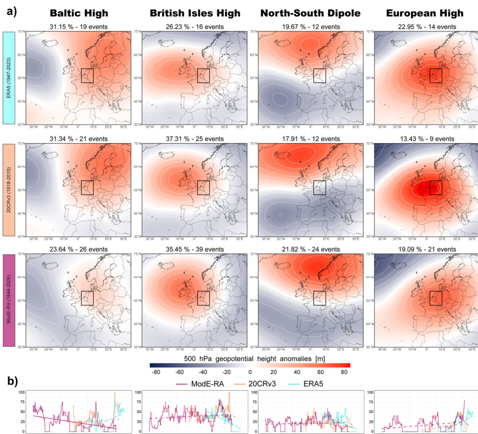
Figure 5: Atmospheric circulation patterns identified from associated with SPEI-3 drought-based clustering (a) and associated drought occurrence trends (b), events and their temporal changes. (a) Cluster centroids of 500 hPa geopotential height anomalies (reference period: 1947–2008) for each period–reanalysis combination. The numbers above each map indicate the percentage and absolute number of drought events assigned to the corresponding cluster within each period–reanalysis combination. The western Central Europe region is delineated by the black box. (b) Ten-year moving fraction (%) of drought events associated with each cluster, using the same colours as in (a). Straight lines represent linear regressions fitted to the moving fractions. Solid lines indicate statistically significant trends according to the modified Mann–Kendall test ( p < 0.05 ), whereas dashed lines indicate non-significant trends ( p \geq 0.05 ).
