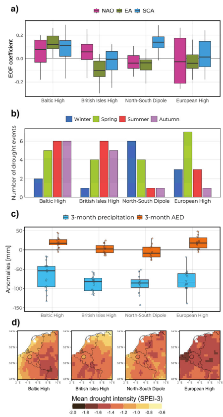
385 Figure 6: Atmospheric characteristics of the atmospheric circulation pattern characteristics associated with patterns identified from SPEI-3 drought-based clustering over 1947–2023 (ERA5); pooling all drought events across seasons and years. (a) Boxplots of EOF 390 coefficients from seasonal EOF analyses of the full Euro-Atlantic record for drought events associated with each circulation pattern (all seasons-pooled). (b) Seasonal distribution of drought events for each circulation pattern. (c) Boxplots of 3-month atmospheric evaporative demand (AED) and precipitation anomalies for each cluster drought events associated with each circulation pattern, with individual events shown as jittered points. For (a) and (c), the black line indicates the median, the box boundaries represent the first and third quartiles, and the whiskers extend to the most extreme values within 1.5 times the interquartile range (IQR). Values beyond the whiskers are shown as individual outliers. (d) Maps of the mean Mean SPEI-3 during drought intensity-for events
