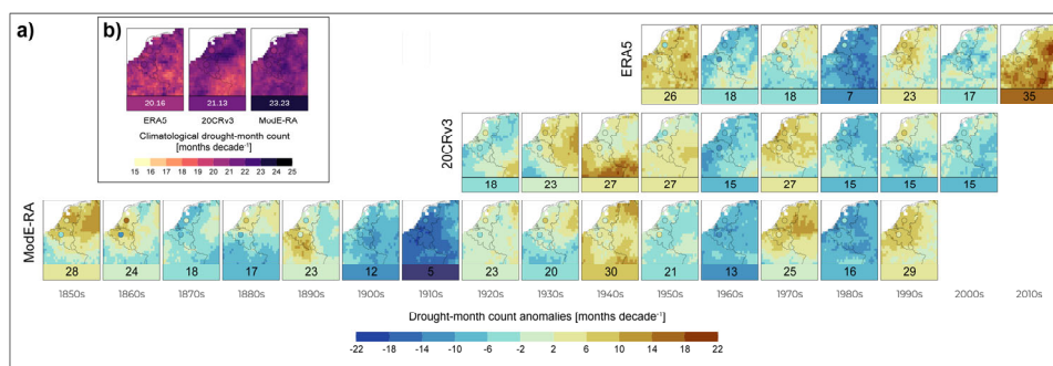
Figure 3: (a) Anomalies in decadal the number of SPEI-3 drought-month counts months per decade for each dataset (rows) and complete-decade, shown for decades fully covered by the corresponding datasets (columns), relative to (b) the mean number of SPEI-3 drought months per decade over the 1947–2008 reference period. Positive values in in both (a) indicate more drought months than and (b), the climatological decadal-mean, whereas negative values indicate fewer. The absolute number of drought months computed at the regional scale is shown below each corresponding map. Discs represent anomalies values at weather stations that fully cover both the corresponding decade and the reference period.
