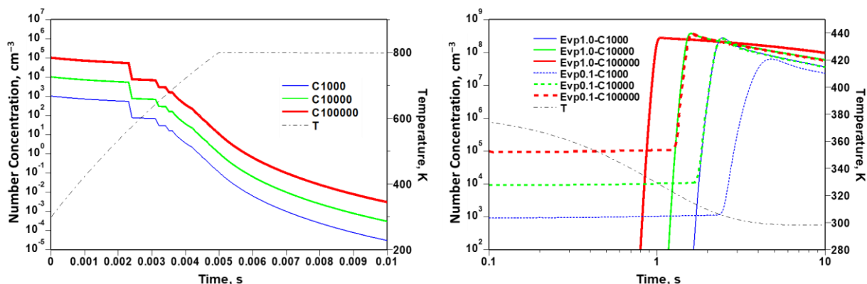
Figure 4: Simulated time evolution of particle concentration. (a) Heating: rapid evaporation; (b) Cooling: burst nucleation with 240 sensitivity to the assumed evaporation fraction. Blue, green, and red curves correspond to initial aerosol number concentrations C = 10^3 , 10^4 , and 10^5 \text{cm}^{-3} , respectively. Solid and dashed lines denote 100% (Evp1.0) and 10% (Evp0.1) evaporation during the heating phase. The black dash-dot curve shows the parcel temperature (right-hand axis). The small zigzag pattern in panel (a) arises from numerical discretization of mass bins and is not a physical signal.
