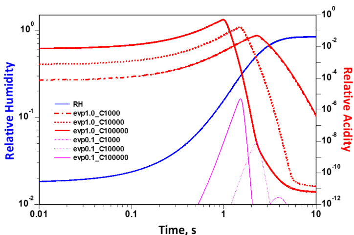
260 Figure 5: Time evolution of relative humidity (defined with respect to \text{H}_2\text{O} ) and relative acidity (defined with respect to \text{H}_2\text{SO}_4 vapor) during the cooling stage (corresponding to the PNC evolution in Fig. 4b). Relative acidity (RA) is categorized by evaporation fraction (thick red curves: 100%; thin magenta curves: 10%) and by initial PNC (dash-dotted, dotted, and solid curves correspond to C=10^3 , 10^4 , and 10^5\text{ cm}^{-3} , respectively). The initial mole fraction of \text{H}_2\text{SO}_4 vapor corresponding to C=10^3 , 10^4 , and 10^5\text{ cm}^{-3} are 2.5\times 10^{-9} , 2.5\times 10^{-8} , and 2.5\times 10^{-7} , respectively, assuming 100% evaporation.
