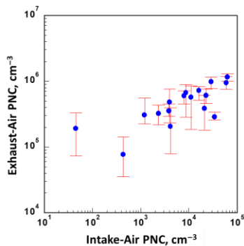
Figure 3: Exhaust PNC increases with intake aerosol loading.
