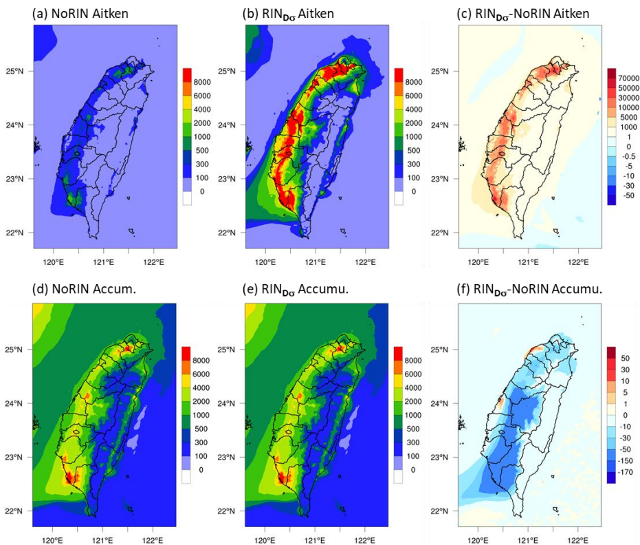
470 Figure 10: Daily Aitken- and Accumulation-mode PNC (in \text{cm}^{-3} ) from the November 20 simulation. Panels (a)–(c) show results from the NoRIN, \text{RIN}_{\text{D}\sigma} , and \text{RIN}_{\text{D}\sigma} -NoRIN cases, respectively. For visual consistency, an upper limit of 10,000 \text{ cm}^{-3} is applied to the color scale in the PNC plots. However, the Aitken-mode PNC in the \text{RIN}_{\text{D}\sigma} simulation (panel b) frequently exceeds this limit. Panel (c) therefore provides a clearer depiction of regions with elevated PNC concentrations.
