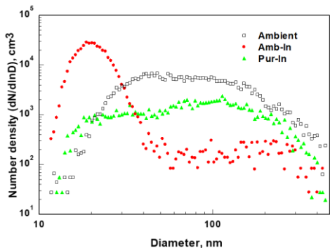
Figure 2: Comparison of PSD for Amb-In (red dots), Pur-In (green triangles), and ambient intake-air (black squares) treatments. Amb-In shows distinct <30 nm nucleation mode and reduced accumulation number.
