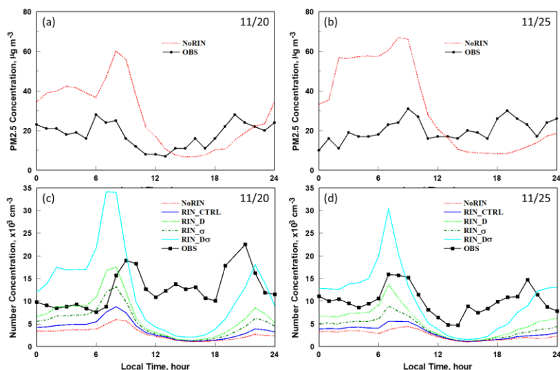
450 Figure 9: Comparison of simulated and observed hourly variations of PM 2.5 (top) and PNC (bottom) on the two selected days. The simulated PM 2.5 values are from the RIN CTRL experiment, as results from other RIN cases are nearly identical. Observed values (OBS) are shown as black solid lines, while simulations from NoRIN, RIN CTRL , RIN D , RIN σ , and RIN Dσ are represented by red dotted, blue solid, light green dotted, dark green dash-dotted, and cyan solid lines, respectively.
