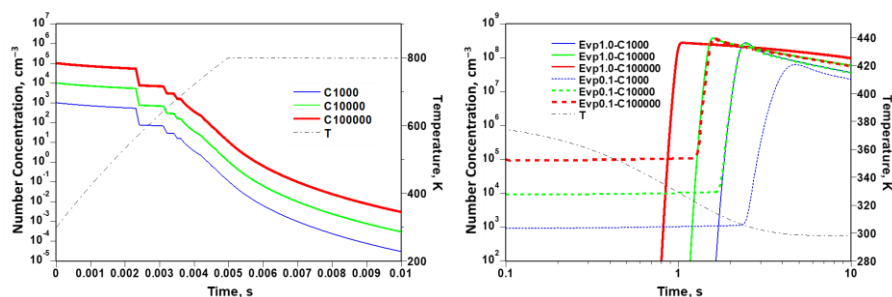
240 Figure 4: Simulated time evolution of particle concentration. (a) Heating: rapid evaporation; (b) Cooling: burst nucleation with sensitivity to the assumed evaporation fraction. Blue, green, and red curves correspond to initial aerosol number concentrations C = 10^3 , 10^4 , and 10^5 \text{cm}^{-3} , respectively. Solid and dashed lines denote 100% (Evp1.0) and 10% (Evp0.1) evaporation during the heating phase. The black dash-dot curve shows the parcel temperature (right-hand axis). The small zigzag pattern in panel (a) arises from numerical discretization of mass bins and is not a physical signal.
