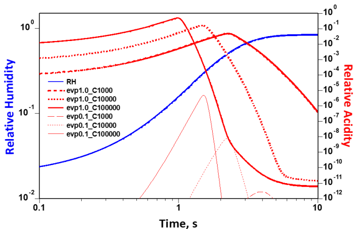
Figure 5: Time evolution of relative humidity (defined with respect to H 2 O) and relative acidity (defined with respect to H 2 SO 4 vapor) during the cooling stage (corresponding to the PNC evolution in Fig. 4b). Relative acidity (RA) is categorized by evaporation fraction (thick red curves: 100%; thin red curves: 10%) and by initial PNC (dashed, dotted, and solid curves correspond to C= 10 3 , 10 4 , and 10 5 cm -3 , respectively). The initial mole fraction of H 2 SO 4 vapor corresponding to C= 10 3 , 10 4 , and 10 5 cm -3 are 2.5x10 -9 , 2.5x10 -8 , and 2.5x10 -7 , respectively, assuming 100% evaporation.
