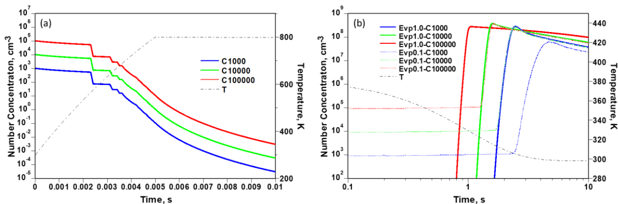
250 Figure 4: Simulated time evolution of particle concentration. (a) Heating: rapid evaporation; (b) Cooling: burst nucleation with sensitivity to the assumed evaporation fraction. Blue, green, and red curves correspond to initial aerosol number concentrations C = 10^3 , 10^4 , and 10^5 \text{cm}^{-3} , respectively. Solid and dotted lines denote 100% (Evp1.0) and 10% (Evp0.1) evaporation during the heating phase. The black dash-dot curve shows the parcel temperature (right-hand axis). The small zigzag pattern in panel (a) arises from numerical discretization of mass bins and is not a physical signal.
