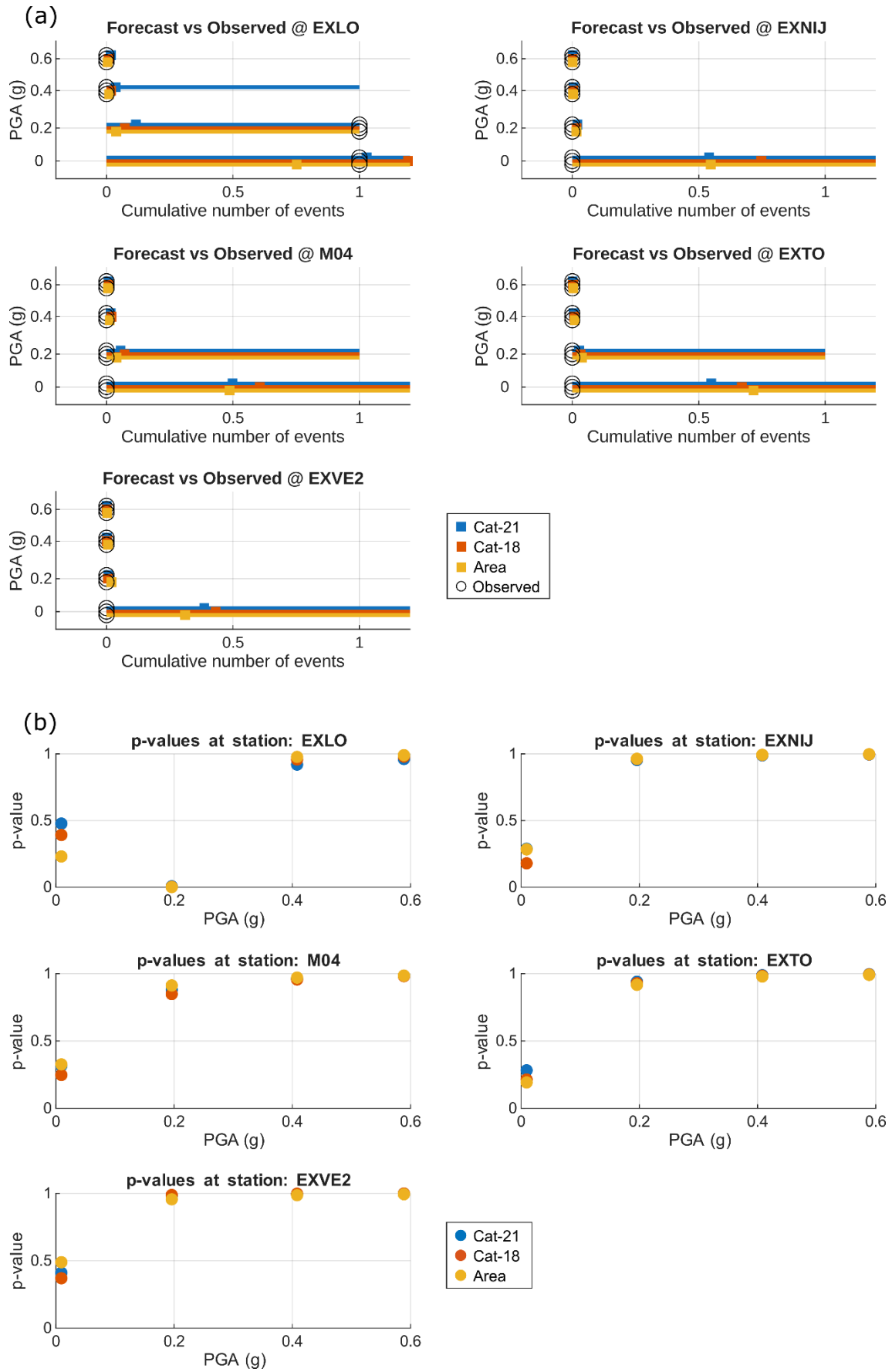
Figure S5. Same as figure 9 of the article but considering observations and forecast for magnitudes equal or above Mw 5 at the different accelerometric stations of the study.
