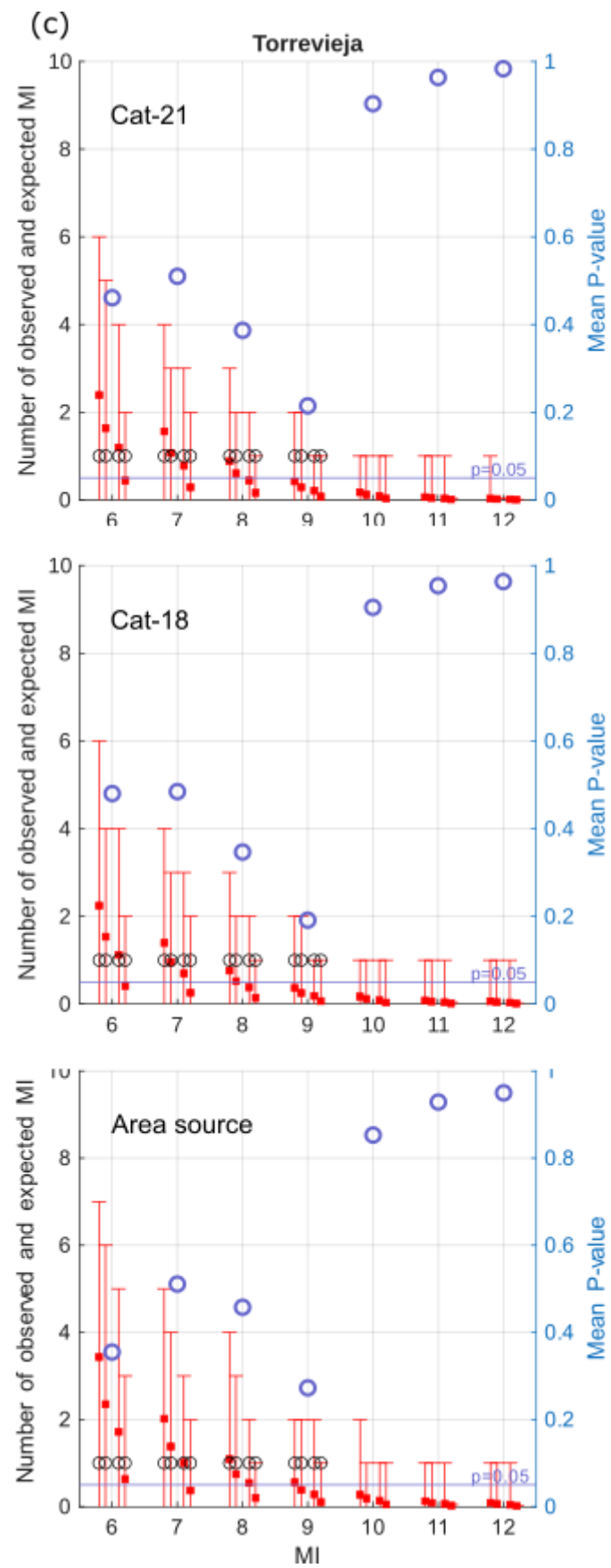
Figure S2. Same as figure 8 of the paper but for the rest of the city locations (Murcia, Vera and Torre Vieja).
