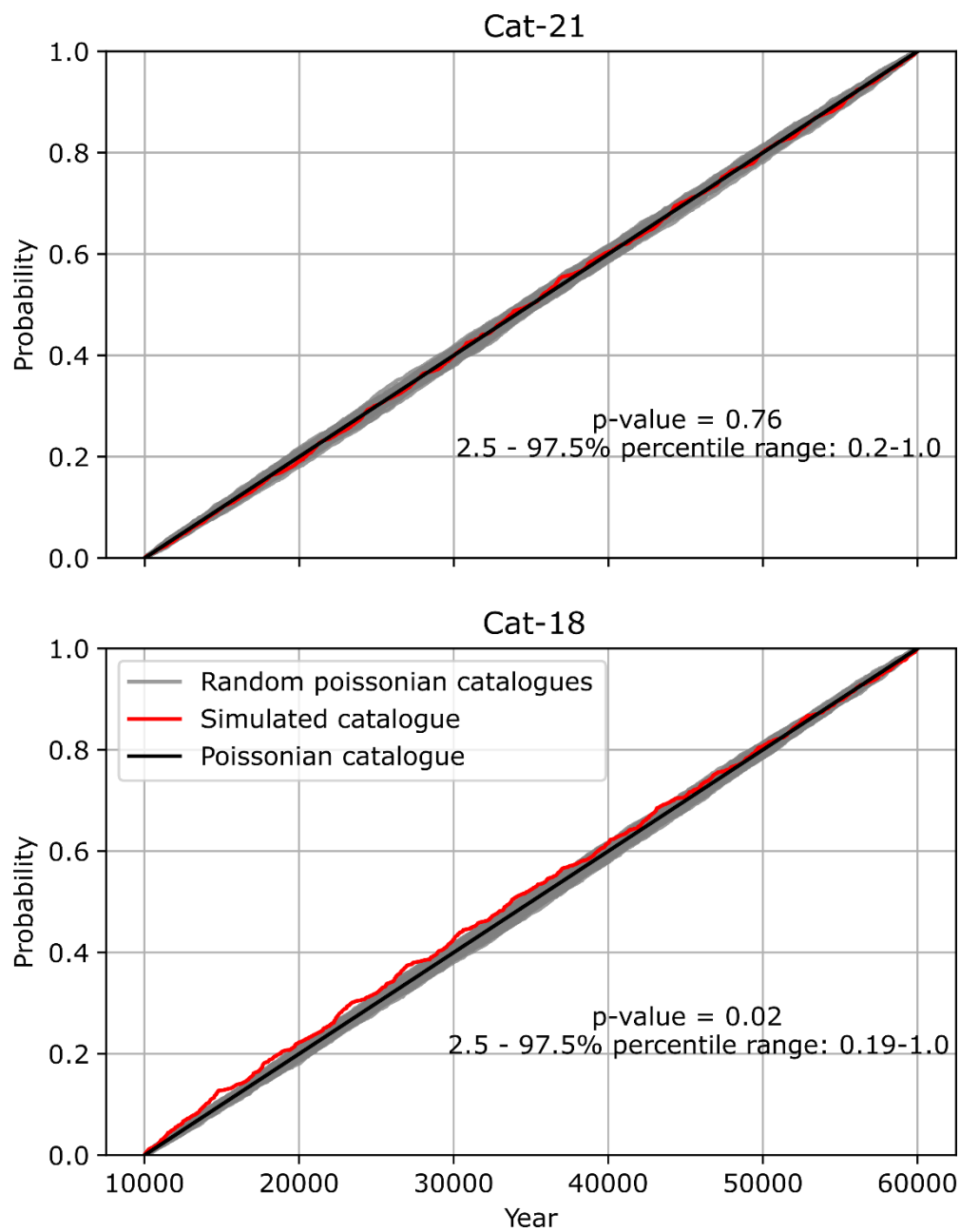
Figure S3. Kolmogorov–Smirnov (KS) test results for the temporal distribution of simulated ruptures in the Cat-21 (top) and Cat-18 (bottom) catalogues considering all ruptures of magnitude equal or above Mw 5.
