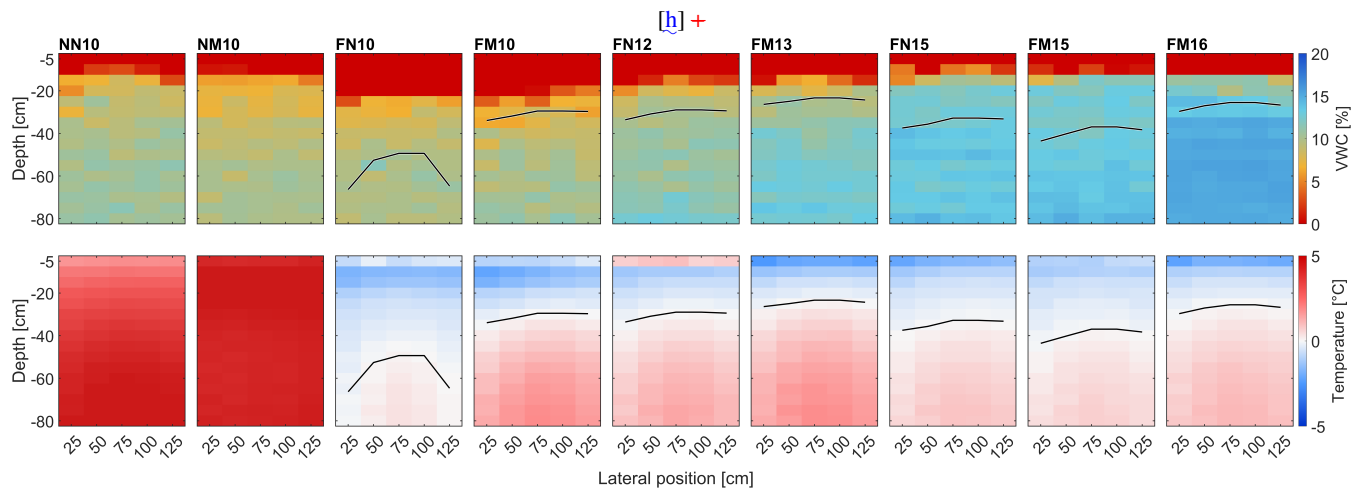
Figure 5. Profiles of volumetric water content (VWC) and temperature for all nine experiments directly after the freezing period and before the start of precipitation ( t = 0 h). The first row shows the total VWC, while the second row depicts the corresponding temperature distribution. The first two profiles represent the unfrozen reference experiments. The black line denotes the 0\text{ }^{\circ}\text{C} isotherm. The slope extends from 0\text{ cm} at the lower end to 150\text{ cm} at the upper end.
