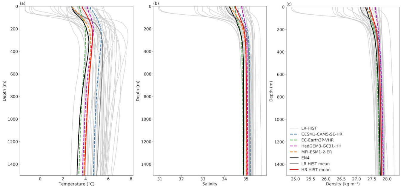
308 Figure 5. Vertical profiles of (a) temperature (in °C), (b) salinity, and (c) density (in kg/m 3 ), averaged over (35°–60° W, 50°–65° N), the 309 Labrador/Irminger Sea (LIS) box shown in Figs. 7 and 8. 310 311
