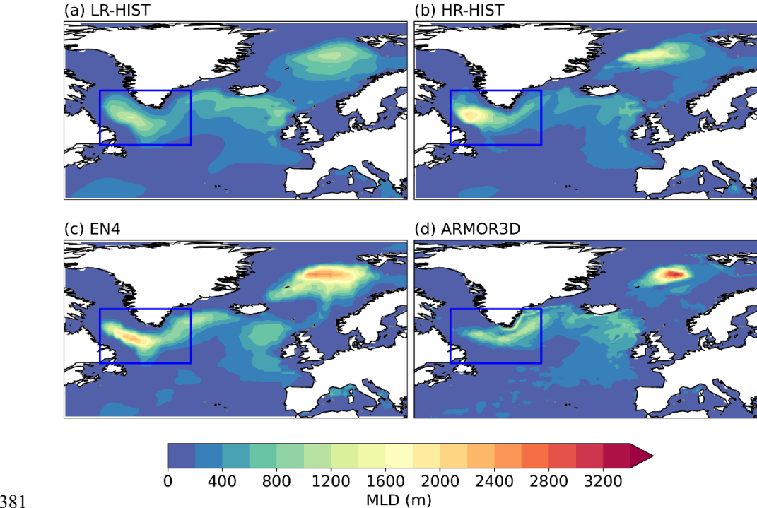
Figure 8. March MLD (in m) by groups, for (a) LR-HIST, (b) HR-HIST, (c) EN4, and (d) ARMOR3D. In all cases, MLD has been calculated from temperature and salinity fields using the density threshold method of 0.03 \text{ kg m}^{-3} described in the manuscript. The time interval covered is 1980–2014 in (a), (b), (c), and 1993–2014 in (d). Plotting details as in Fig. 7.
