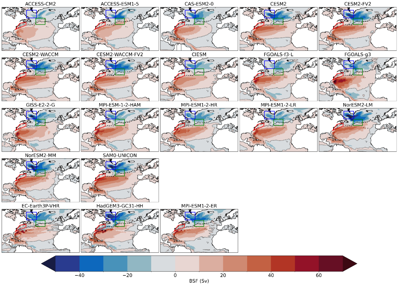
476 Figure 12. Barotropic streamfunction (BSF; in Sv) for LR-HIST (rows 1–4) and HR-HIST models (last row). Zero contour of absolute 477 dynamic topography from AVISO observations (dashed black line) corresponding to the period 1993–2014 is also shown. Boxes as in Figs. 478 2 and 4: NCH in red, CNA in green, LS in blue. Note: some models did not present a BSF output (e.g. CESM1-CAM5-SE-HR) or this 479 presented unrealistic values, hence the reason fewer models are shown in this figure. 480 481 482
