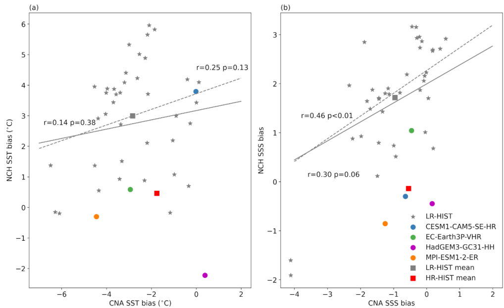
788 Figure A2. Scatterplots of (a) SST (in °C) and (b) SSS biases between the Central North Atlantic (CNA) and North Cape Hatteras (NCH) 789 regions defined in Fig. 2. Biases are calculated as spatially averaged temporal means in the model minus the corresponding EN4 values in 790 each of the selected boxes. The corresponding correlation coefficients and their p-values are shown next to the fit lines. Dashed lines are 791 regression lines obtained after removal of HR-HIST models. Note: all regression lines and values in (b) are calculated excluding the two 792 outliers at the bottom left of the figure.
