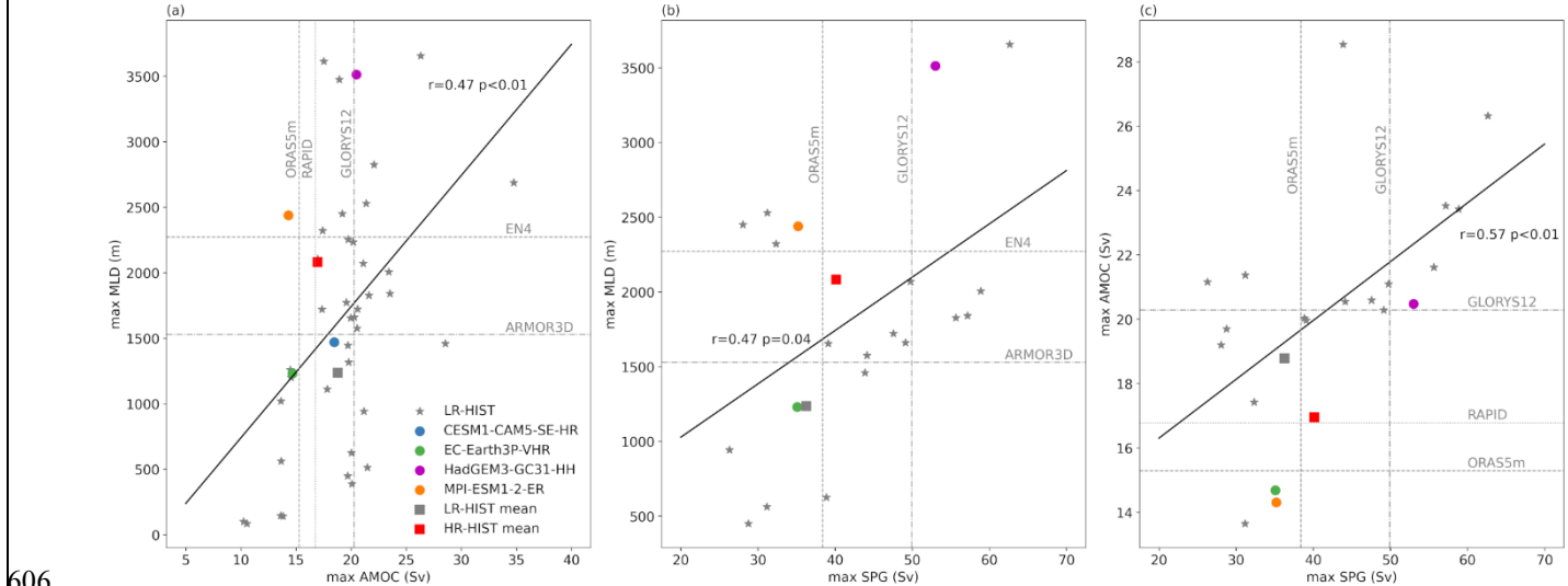
Figure 14. Scatterplots of (a) max. Atlantic overturning vs max. MLD, (b) SPG strength vs max. MLD, and (c) SPG strength vs max. overturning. The corresponding Pearson correlation coefficients and their p-values are shown next to the fit lines. Dashed/dotted vertical and horizontal lines indicate observational/reanalysis values. Units for max. MLD, overturning, and SPG strength are m, Sv, and Sv, respectively. Max. MLD is calculated in the LIS box (35°–60° W, 50°–65° N), which is shown in Figs. 7 and 8. Max. SPG strength is calculated as the absolute value of the minimum of the BSF, also in the LIS box. Max. overturning is calculated at 26.5° N. Correlation coefficients and fit lines are based on the composite of the LR-HIST and HR-HIST ensembles (LR-HIST + HR-HIST).
