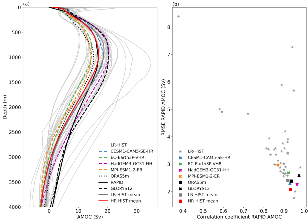
433 Figure 11. (a) Climatological Atlantic overturning profile in depth-space at 26.5° N (in Sv). (b) Pearson correlation coefficient (horizontal 434 axis) and Root Mean Square Error (RMSE; in Sv) (vertical axis) of vertical profiles in (a) against RAPID. In both subplots, models and 435 ORAS5m reanalysis data correspond to the interval 1980–2014, RAPID observations are averaged over the period April 2004–December 436 2014, and GLORYS12 reanalysis over the interval 1993–2014. 437
