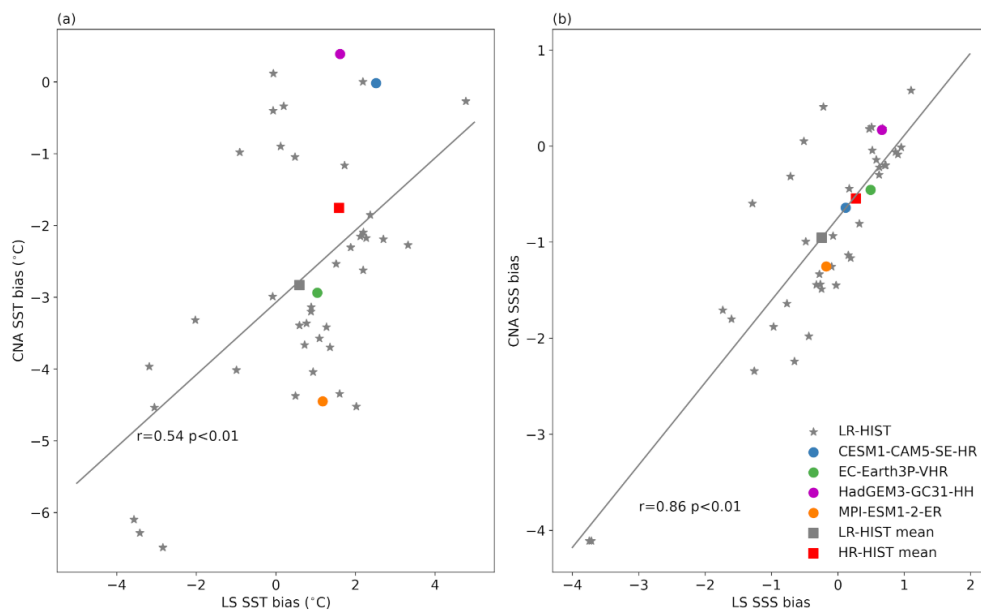
Figure A3. Scatterplots of (a) SST (in °C) and (b) SSS biases between the Labrador Sea (LS) and Central North Atlantic (CNA) regions defined in Fig. 2. The corresponding Pearson correlation coefficients and their p-values are shown next to the fit lines. Correlation coefficients and fit lines are based on the composite of the LR-HIST and HR-HIST ensembles (LR-HIST + HR-HIST).
