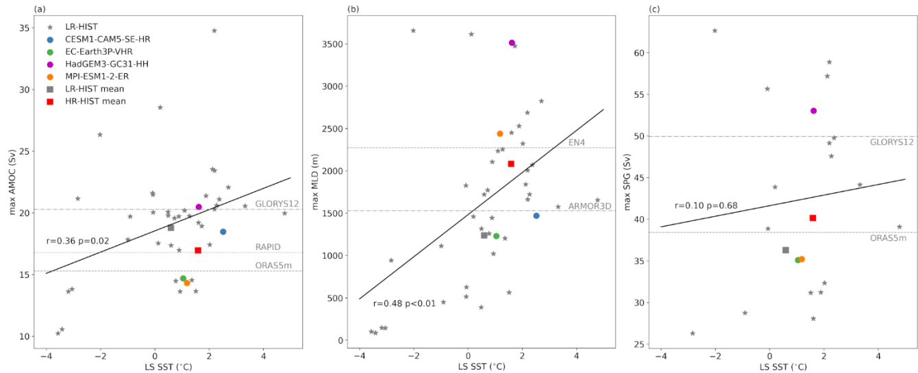
783 Figure A1. Scatterplots of LS SST vs (a) max. Atlantic overturning streamfunction at 26.5° N, (b) max. MLD, and (c) max. SPG strength. 784 LS SST biases are calculated in the LS box (44°–60° W, 52.5°–65° N), which is shown in Fig. 2. Remaining plotting details as in Fig. 14. 785
