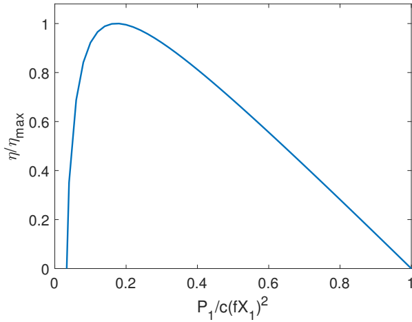
175 Figure 1. The power-yield tradeoff predicted by the modified Odum-Pinkerton model. Here, we set l = 0 and \epsilon = 0.03 , so that the model is describing the 7 th example in Odum and Pinkerton (1955), which represents an organism that captures (via J_1 ) and uses food for its maintenance (signified by \epsilon ) and growth (via J_2 ), except that we here assume that the maintenance cost is paid by X_2 (analogous to the reserve biomass in the variable internal storage models, e.g., the DEB models in this study). While we do 80 not plot negative values of \eta , it may occur resembling to a starving organism that keeps respiring at the expense of biomass under insufficient food supply.
