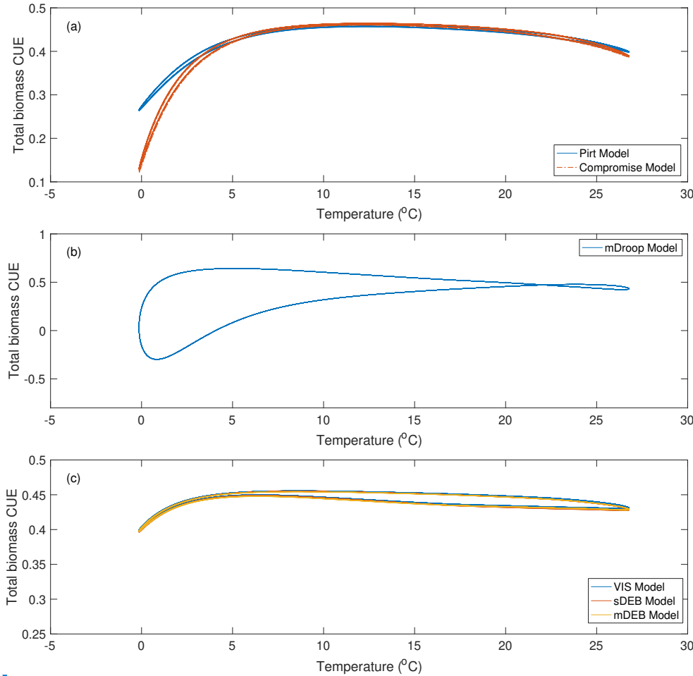
Figure 6. Variation of total biomass CUE with respect to temperature for different models. Results were plotted using the last 40 years of the 50-year simulations (shown in Figure S3).
