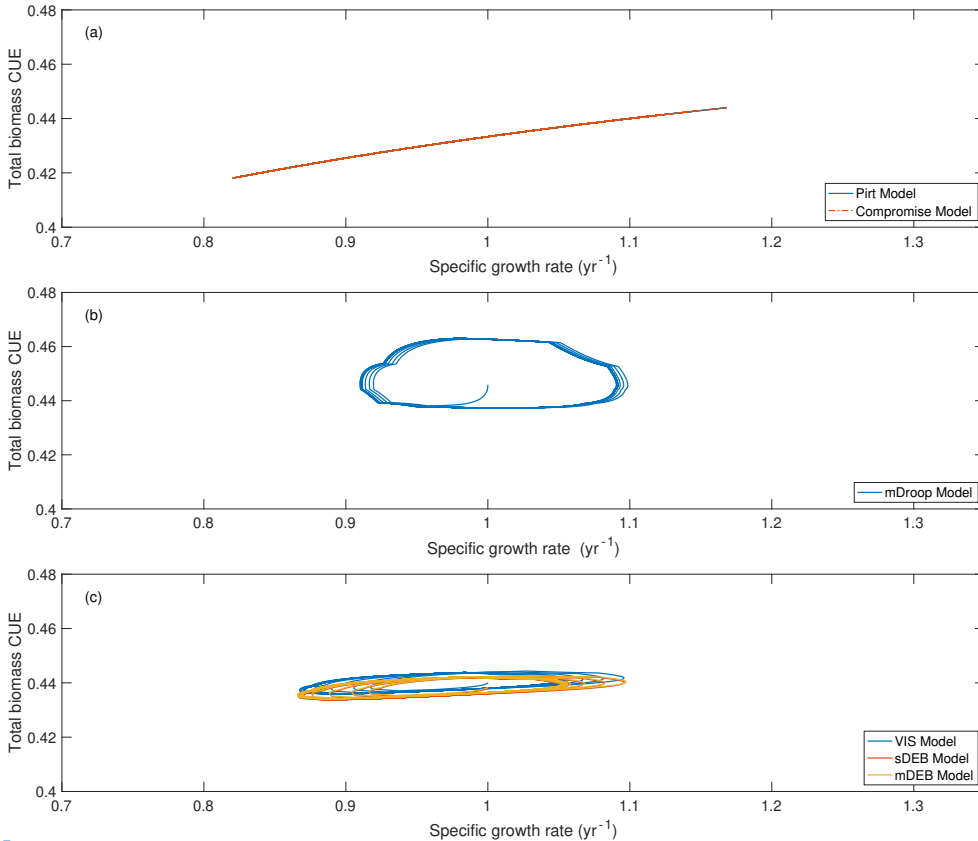
Figure 3. Relationship between total biomass CUE and specific growth rate. The evolution of different microbial carbon pools and total microbial biomass is presented in Figure S2 in the supplemental material. Note that results for the Pirt model and the Compromise model overlap each other in panel (a).
