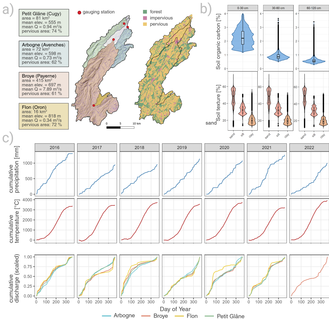
Figure 3. a: Sub-catchments and gauging station location and landcover classes . b: Soil texture and soil organic carbon for the total Broye catchment. c: cumulative temperature and precipitation sums for the whole catchment, cumulative sum of discharge for sub-catchments [scaled for easier comparison, in 2022 only data available for the Broye sub-catchment ]
