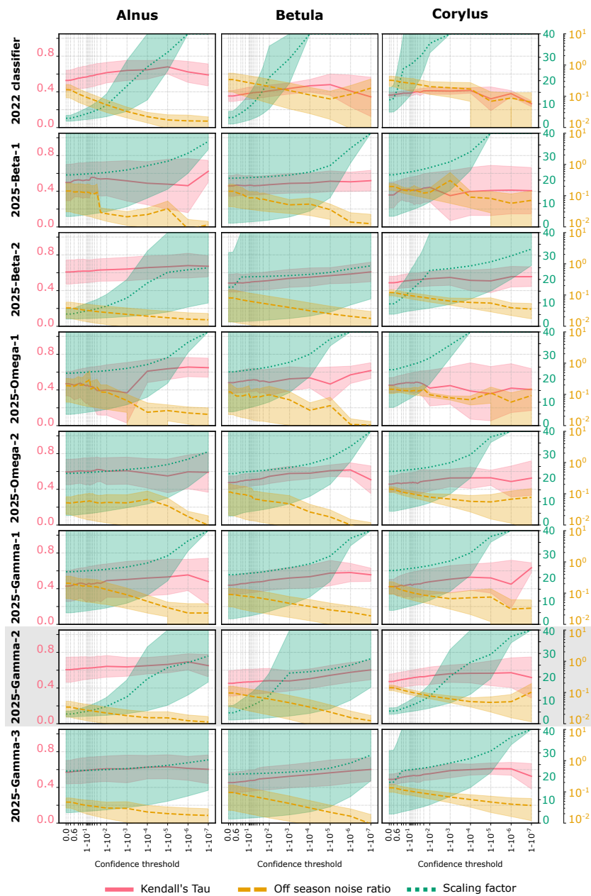
Figure 1. Kendall's Tau correlation, scaling factor and off-season noise ratio as a function of the confidence threshold for Alnus, Betula and Corylus (columns) and for each classifier (rows). The yellow, green and red areas represent the spread of values across the five sites while the thick lines show the averages. Note that the axis of the scaling factor stops at 40, while values range up to 1000. The grey frame highlights the best classifier. The 2025-Gamma-2 panel is presented in Crouzy et al. (2025) (Crouzy et al., 2025)
