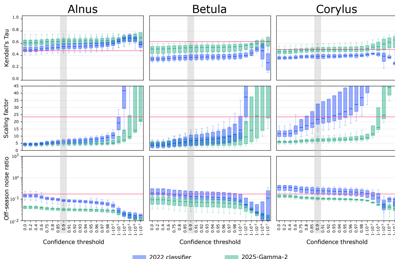
Figure 2. Kendall Tau correlation, scaling factor and off-season noise ratios as a function of confidence threshold for the five stations and for the 2022 and 2025-gamma-2 classifiers. Columns show Alnus, Betula and Corylus, from left to right. Metrics are computed at each threshold, in green for the 2025-Gamma-2 classifier, in blue for the 2022 classifier. Scaling factors higher than 45 are not shown. The boxplots illustrate the values of each metric, at each confidence threshold, for all stations. Red lines indicate the acceptability threshold values for each individual metric and taxa.
