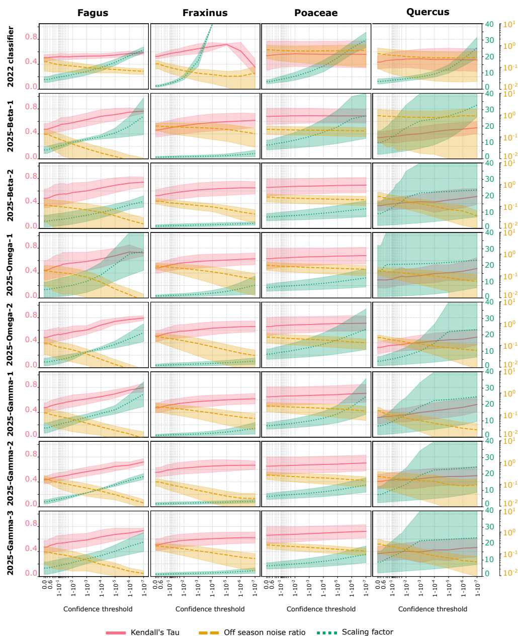
Figure A1. Kendall Tau correlation, scaling factor and Off-season noise ratio as a function of the confidence threshold for Fagus, Fraxinus, Poaceae and Quercus for the five sites and eight classifiers.
