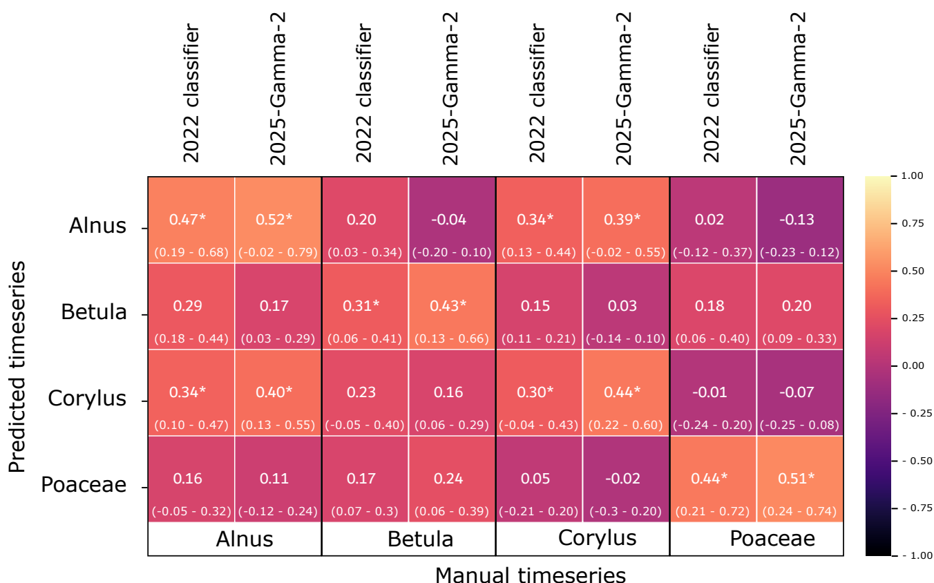
Figure 4. Heatmap of the averaged Kendall Tau correlations between the predicted and manual timeseries for the 2022 and 2025-Gamma-2 classifiers. Numbers and corresponding colours indicate the Kendall's Tau values between the predicted timeseries of the class on the y axis, and the manual observation timeseries of the class on the x axis. The minimum and maximum Kendall's Tau across stations are reported in parenthesis. * indicates that the Kendall Tau value is higher than 0.5 when calculated between the manual timeseries of the two classes, indicating an expected correlation between two classes. All predicted timeseries have been produced with the optimal confidence threshold identified for the class and algorithm.
