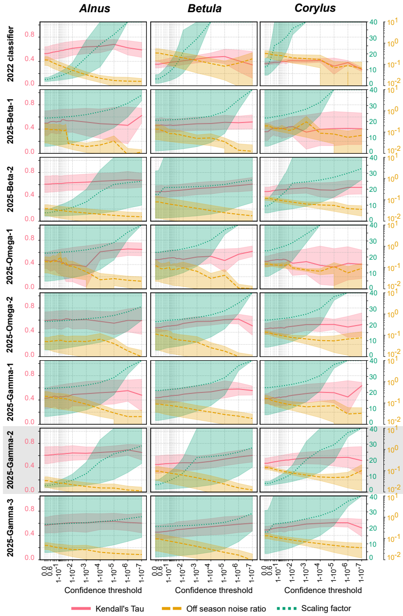
Figure 1. Kendall's Tau correlation, scaling factor and off-season noise ratio as a function of the confidence threshold for Alnus , Betula and Corylus (columns) and for each classifier (rows). The yellow, green and red areas represent the spread of values across the five sites while the thick lines show the averages. Note that the axis of the scaling factor stops at 40, while values range up to 1000. The grey frame highlights the best classifier. The 2025-Gamma-2 panel is presented in a companion short note Crouzy et al. (2025) (Crouzy et al., 2025)
