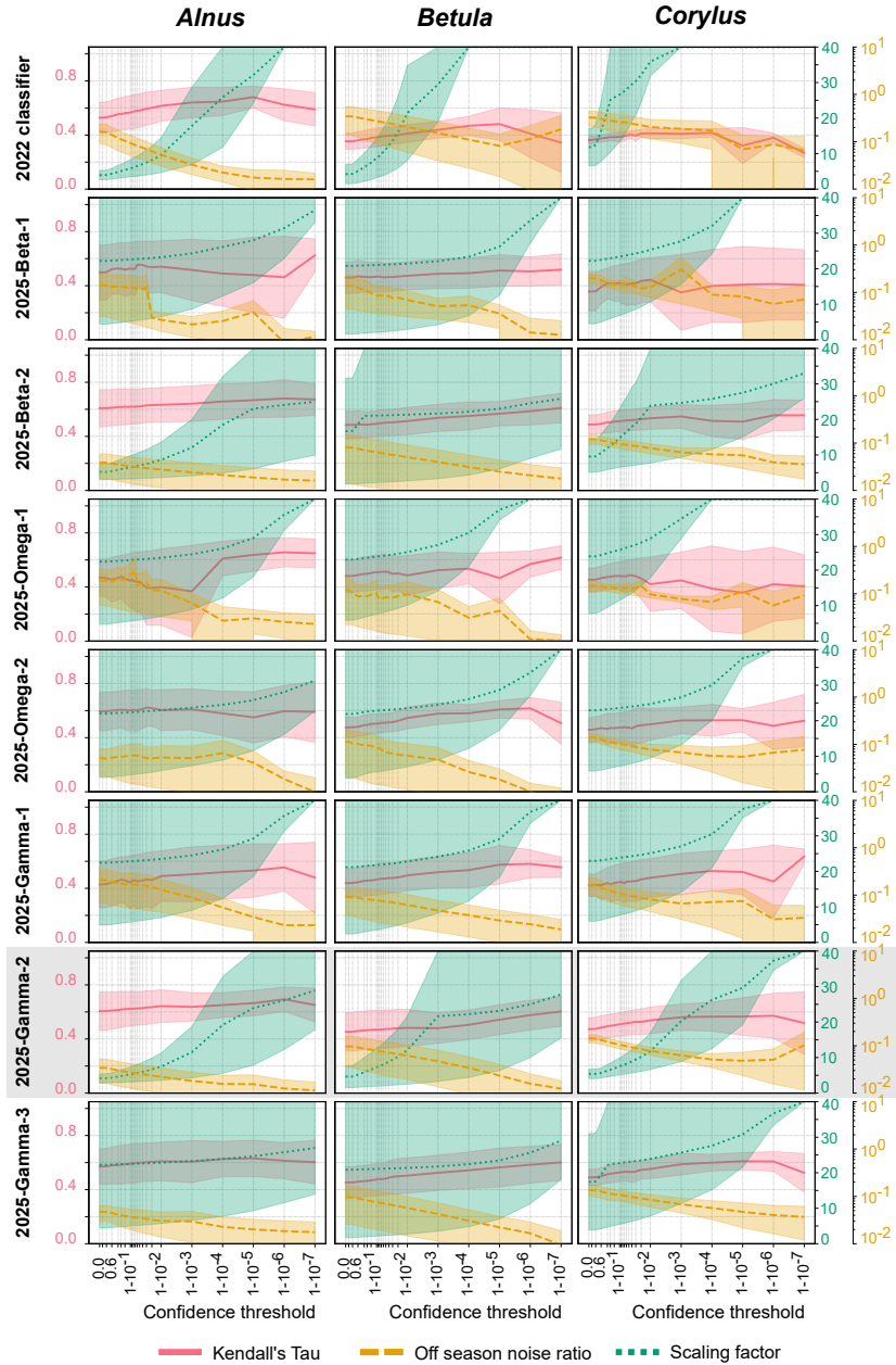
Figure 1. Kendall's Tau correlation, scaling factor and off-season noise ratio as a function of the confidence threshold for Alnus , Betula and Corylus (columns) and for each classifier (rows). Kendall's Tau correlation, scaling factor and off-season noise ratio as a function of the confidence threshold for Alnus , Betula and Corylus (columns) and for each classifier (rows). The yellow, green and red areas represent the spread of values across the five sites while the thick lines show the averages. Note that the axis of the scaling factor stops at 40, while values range up to 1000. The grey frame highlights the best classifier. The 2025-Gamma-2 panel is presented in Crouzy et al. (2025) (Crouzy et al., 2025)
