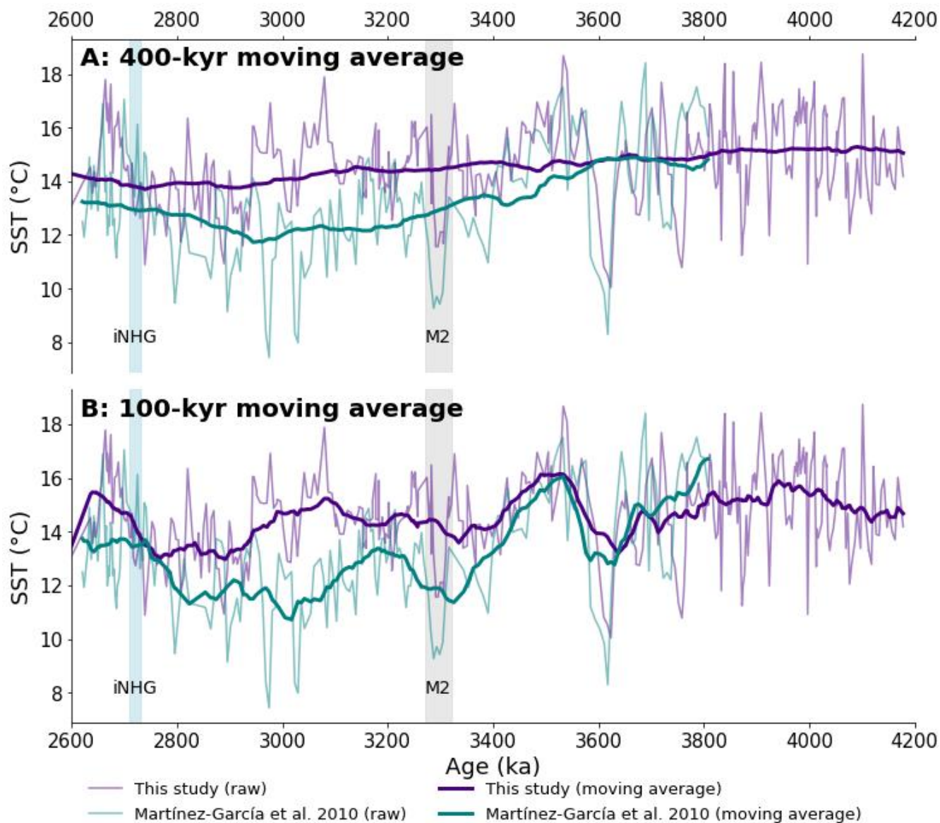
330 Figure 3: A comparison of our alkenone-based SST estimates from ODP Site 1090 and that of Martínez-García et al., (2010). The teal line denotes the original U^{k_{37}} -based SST Martínez-García et al. (2010) estimates plotted using their age-depth model (Martínez-García et al., 2011), while the SST record constructed during this study is plotted in indigo using our new age-depth model. The approximate beginning of iNHG (~2.72 Ma) is highlighted in blue, and the MIS M2 glacial event is highlighted in gray. The top panel (A) shows the full high-resolution records overlaid by a 400-kyr moving average, and the bottom panel (B) displays the same records with a 100-kyr moving average. In both cases, our new record shows elevated temperature estimates in the interval between MIS M2 and iNHG, where we noted an offset between the Martínez-García et al. (2010) data and other published records.
