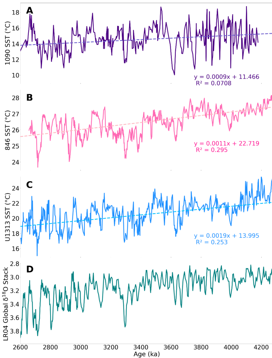
360 Figure 4: When comparing our Site 1090 record (A) to those from other regions (here, eastern equatorial Pacific [ODP 846, panel B] and the northeast Atlantic [IODP U1313, panel C]) we observe little evidence of early cooling in the high latitude southern hemisphere compared to the rest of the world. Notice the similar, slightly negative cooling trend at all three sites, indicative of cooling occurring synchronously across the globe; in fact, ODP Site 1090 displays a less negative cooling trend throughout the late Pliocene than at ODP Site 846 (eastern equatorial Pacific) or IODP Site U1313 (north Atlantic). Also displayed is the LR04 benthic oxygen isotope stack (panel D) from 2600–4280 ka.
