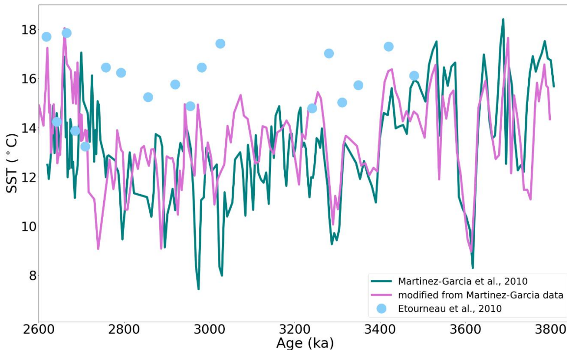
Figure 2: Previously published alkenone-based SST estimates from ODP Site 1090. The teal line denotes the original U^k_{37} -based SST Martínez-Garcia (2010) estimates plotted with their 2011 age model, while the pink line indicates our
