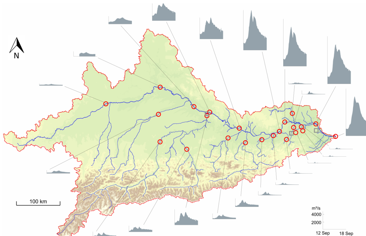
Figure 9: Overview of the Upper Danube catchment and tributary hydrographs during the September 2024 flood. The map shows the river network and key gauging stations (red circles), with stylized discharge hydrographs for the period 12 - 18 September 2024.
