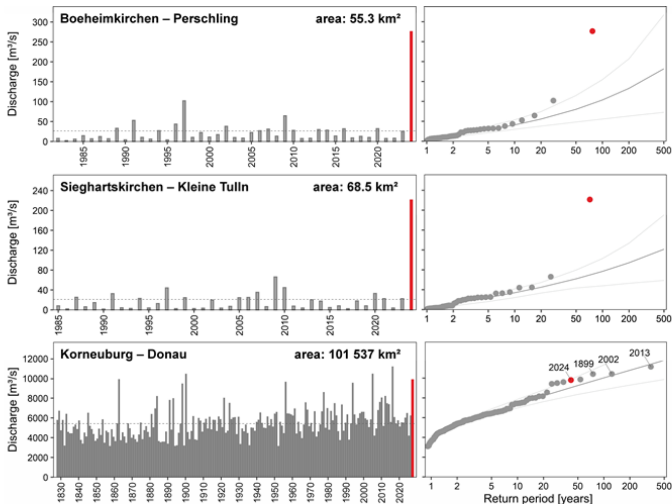
Figure 12: Annual maximum discharges and flood-frequency analyses for selected stations. Top: Perschling at Böhheimkirchen (55.3 km²). Middle: Kleine Tulln at Sieghartskirchen (68.5 km²). Bottom: Danube at Korneuburg (101 537 km²). Bars show annual peak discharges; dots and fitted curves indicate frequency distributions. The September 2024 flood is highlighted in red; historical reference events are shown for comparison.
