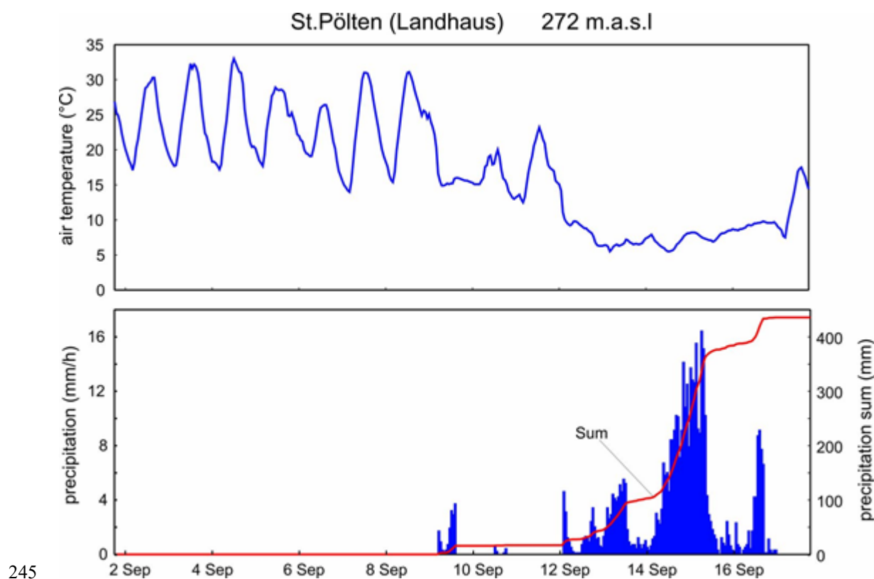
Figure 6: Hourly meteorological data recorded at St. Pölten (Landhaus station, 272 m a.s.l.) from 2 to 17 September 2024. The upper panel shows mean hourly air temperature (°C). The lower panel shows hourly precipitation sums (mm, blue bars) and cumulative precipitation sum (mm, red line).
