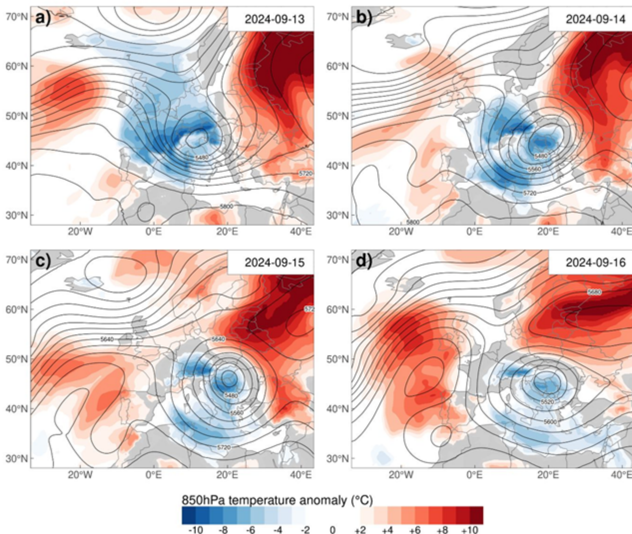
170 Figure 3: Evolution of the 850 hPa temperature anomaly (°C) and 500 hPa geopotential height (gpm) during the September 2024 flood event over Central Europe. Panels show daily snapshots from (a) 13 September, (b) 14 September, (c) 15 September, and (d) 16 September. Blue and red shading indicates negative and positive temperature anomalies, respectively, relative to the 1991–2020 climatology.
