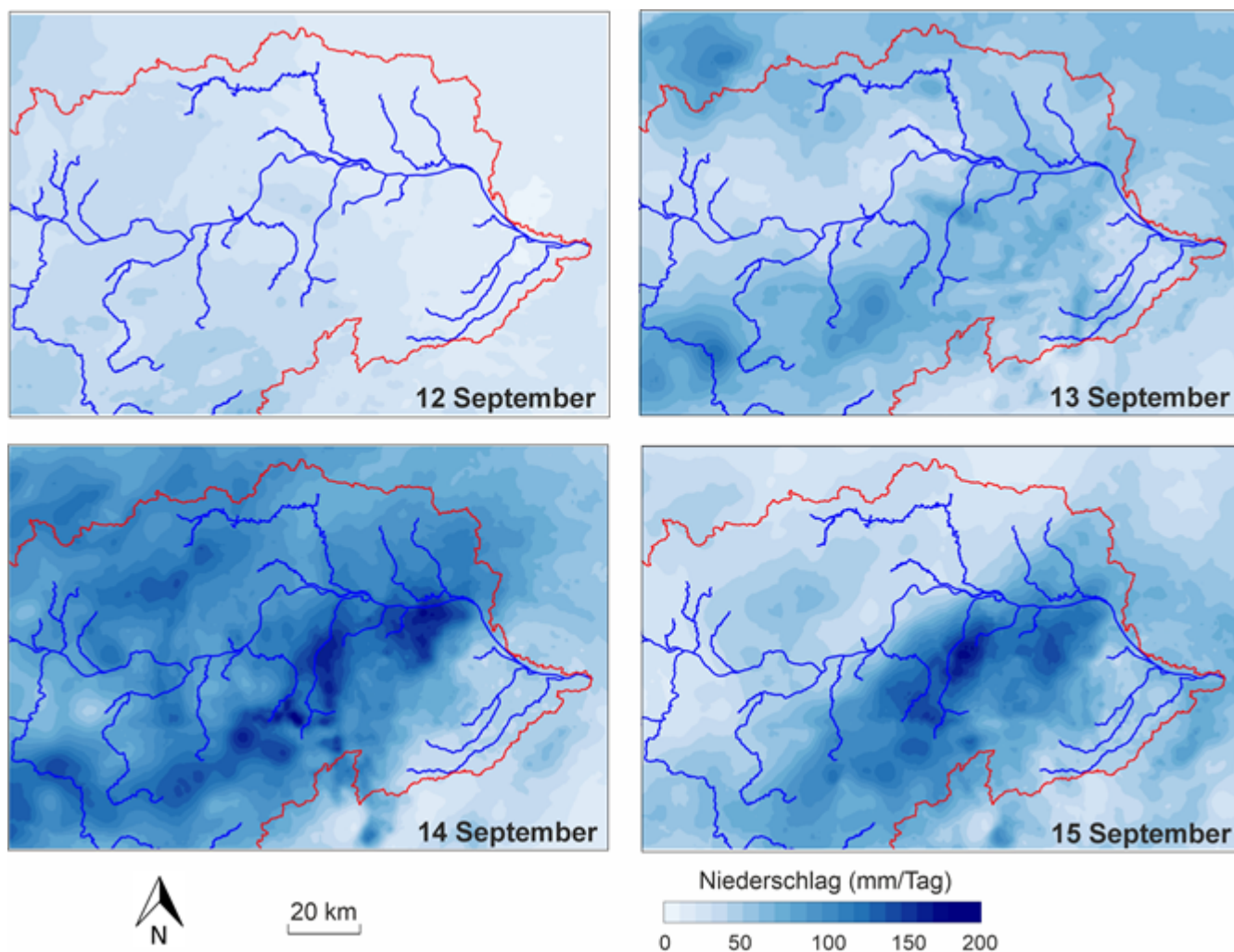
Figure 5: Observed daily precipitation (24-hour totals) in eastern Austria on (a) 12 September, (b) 13 September, (c) 14 September, and (d) 15 September 2024. Data are from the INCA gauge - radar analysis (Haiden et al., 2011). The red outline indicates the Upper Danube catchment.
