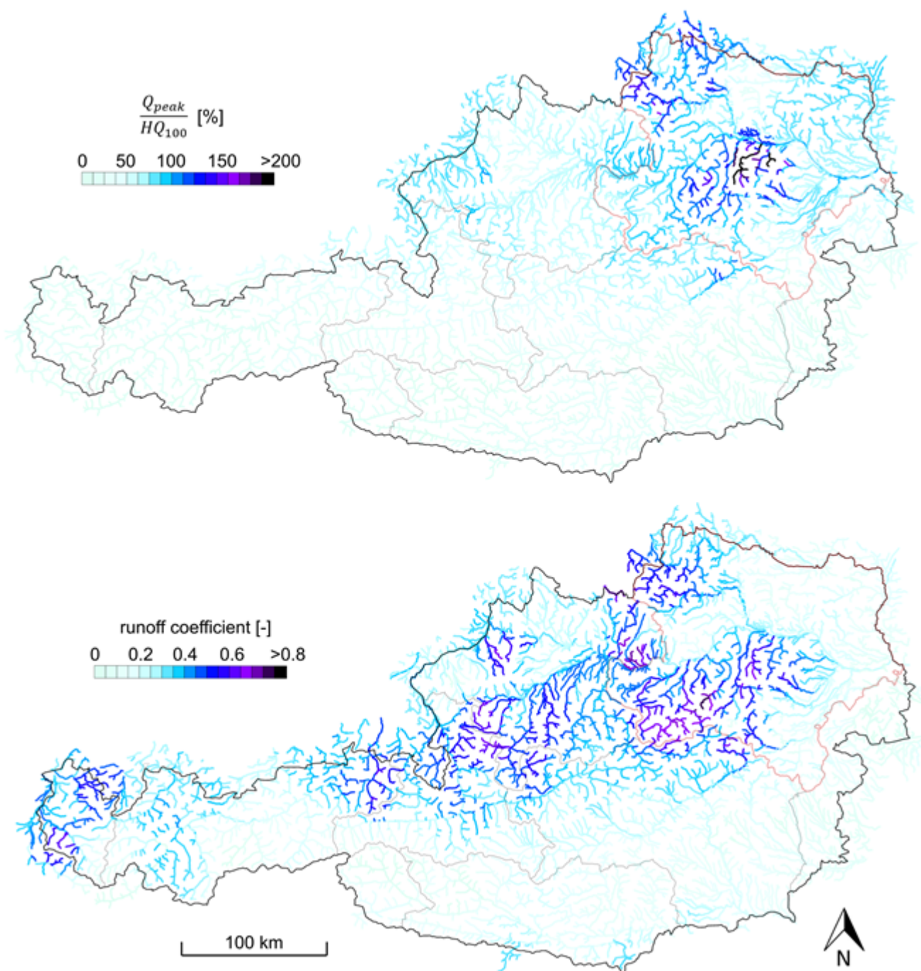
Figure 13: Characteristics of the September 2024 flood event in Austria. Upper panel: Map showing the ratio of observed peak discharge ( Q_{peak} ) to the local 100-year flood discharge ( HQ_{100} ), expressed as a percentage. Values greater than 100% (darker blue colors) indicate stations where the 2024 peak discharge exceeded the HQ_{100} threshold. Lower panel: Map of the event runoff coefficients, defined as the ratio of runoff volume to precipitation volume in each catchment (unitless).
