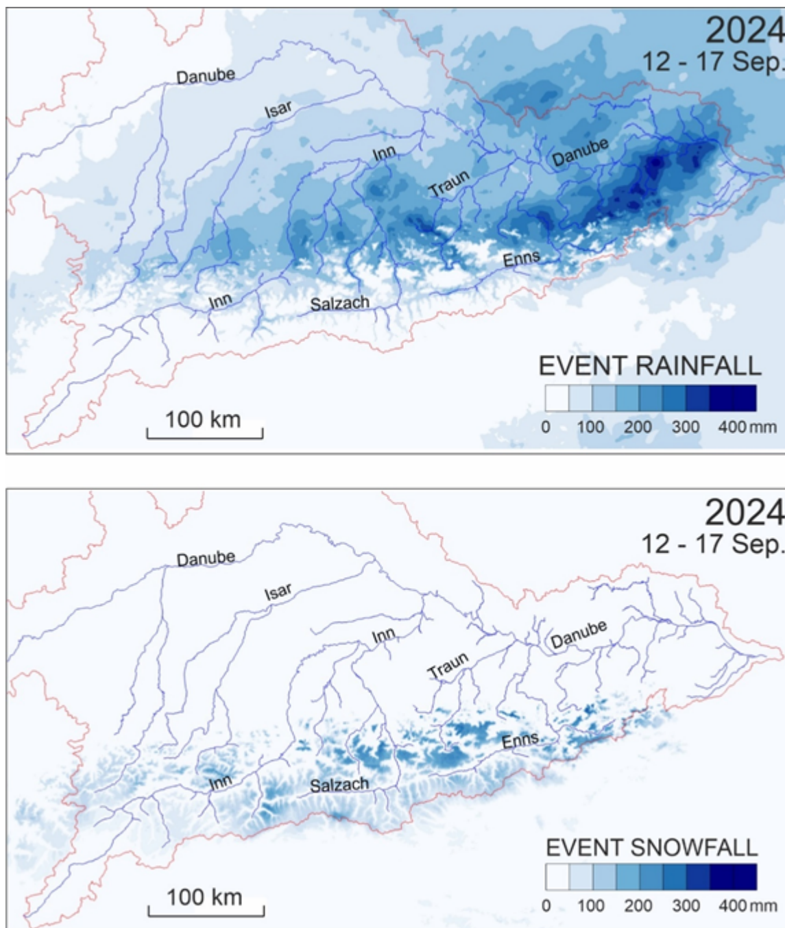
Figure 7: Precipitation phase in the Danube Basin during the September 2024 event. Top: Total rainfall (liquid precipitation) from 12 Sep 00:00 to 17 Sep 00:00, in mm. Bottom: Total snowfall (solid precipitation) over the same period, in mm water equivalent. Data are based on INCA analysis (Haiden et al., 2011). The red outline shows the Upper Danube catchment boundary.
