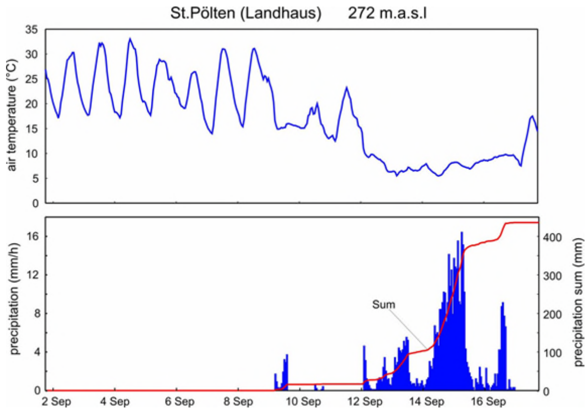
Figure 6: Hourly meteorological data recorded at St. Pölten (Landhaus station, 272 m a.s.l.) from 2 to 17 September 2024. The upper panel shows mean hourly air temperature (°C). The lower panel shows hourly precipitation sums (mm, blue bars) and cumulative precipitation sum (mm, red line).
