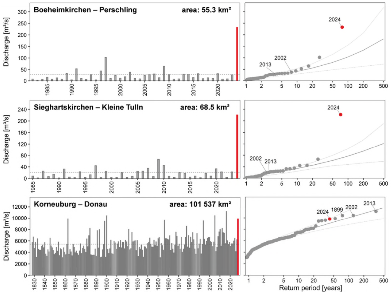
490 Figure 12: Annual maximum discharges and flood-frequency analyses for selected stations. Top: Perschling at Böhheimkirchen (55.3 km 2 ). Middle: Kleine Tulln at Sieghartskirchen (68.5 km 2 ). Bottom: Danube at Korneuburg (101 537 km 2 ). Bars show annual peak discharges; dots and fitted curves indicate frequency distributions. The September 2024 flood is highlighted in red; historical reference events are shown for comparison.
