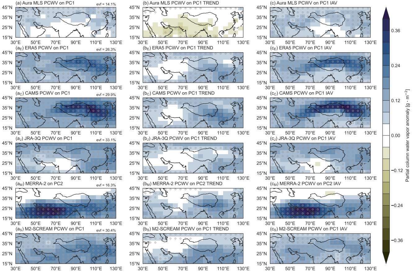
Figure 1. Deseasonalized partial-column water vapor (PCWV) anomalies (Eq. 1) regressed onto the (a) first principal component (PC1) from Aura MLS and its (b) trend ( \text{PC1}_{\text{TREND}} ) and (c) interannual variability ( \text{PC1}_{\text{IAV}} ) components. Corresponding distributions are shown for (a E )–(c E ) ERA5 PCWV on PC1 from ERA5, (a C )–(c C ) CAMS PCWV on PC1 from CAMS, (a J )–(c J ) JRA-3Q PCWV on PC1 from JRA-3Q; (a M )–(c M ) MERRA-2 PCWV on the second principal component (PC2) from MERRA-2; and (a S )–(c S ) M2-SCREAM PCWV on PC1 from M2-SCREAM. Principal components (Fig. 3a–c) are based on EOF analysis of vertical and horizontal variations in water vapor for the five Aura MLS pressure levels within 68 hPa–147 hPa, 30°E–130°E, and 15°N–45°N (Sect. 2.2). The location of the Tibetan Plateau is marked by a dark grey contour and stippling indicates that the regression is significant at the 95% confidence level based on Student’s t test. The fraction of total variance explained by each mode is listed at the upper right of panels in column (a).
