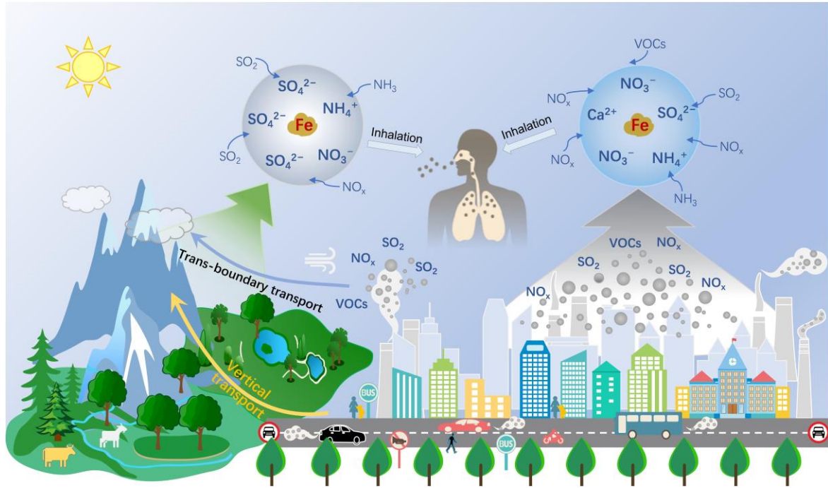
Figure 8: Schematic illustration of atmospheric iron acid dissolution processes in the upper mixing layer and at the ground-level, and their potential implications for human health.
