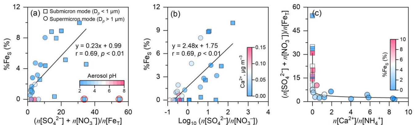
Figure 7: Scatter plots of (a) (n[\text{SO}_4^{2-}] + n[\text{NO}_3^-])/n[\text{Fe}_\text{T}] versus %Fe s , (b) \log_{10}(n[\text{SO}_4^{2-}]/n[\text{NO}_3^-]) versus %Fe s , and (c) (n[\text{Ca}^{2+}]/n[\text{NH}_4^+]) versus (n[\text{SO}_4^{2-}] + n[\text{NO}_3^-])/n[\text{Fe}_\text{T}] , respectively, in the size-resolved aerosols at Mt. Daming. Solid circles and squares are colored by aerosol pH, \text{Ca}^{2+} and %Fe s in (a), (b), and (c), respectively. In plot a, two outliers are not included in the correlation analysis due to the relatively low Fe s concentrations and are indicated by red circles.
