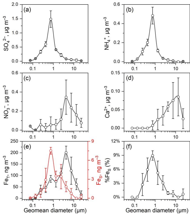
Figure 2: Size distributions of (a) \text{SO}_4^{2-} , (b) \text{NH}_4^+ , (c) \text{NO}_3^- , (d) \text{Ca}^{2+} , (e) \text{Fe}_T (black) and \text{Fe}_S (red), and (f) % \text{Fe}_S in the size-resolved aerosols at the upper mixing layer (Mt. Daming). The vertical bars represent one standard deviation for each diameter measurement ( n = 3 ).
