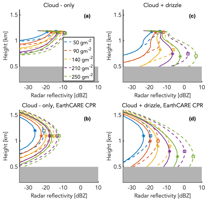
240 Fig. 3. (a) Reflectivity profiles forward calculated from the 1D microphysical model output using the cloud only hydrometeors; (b) same as (a), but with the PTR applied. (c) Reflectivity profiles forward calculated from the 1D microphysical model output using both the cloud and drizzle hydrometeors (which correspond to the actual radar signal); (d) same as in (c), but with PTR applied. Solid and dash lines indicate that total number of cloud droplets per unit of volume (200 and 50 m^{-3} , respectively). Colors indicate different cloud LWP in gm^{-2} as shown in legend. Asterisks and squares respectively represent the height of the Z_{MAX} . The gray zone indicates the region contaminated by the surface clutter. 245
