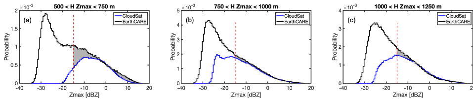
460 Fig. 9. The probability distribution Z_{MAX} values at different height ranges above the ocean surface: (a) between 500 and 750 m; (b) 465 between 750 and 1000 m; and (c) between 1000 and 1250 m. Black and blue lines respectively indicate the EC-CPR and CS-CPR observations collected in SEA and SEP. The three categories are responsible for a Sc cloud fraction of 7.5%, 14.7%, 12.4% for EC and 2.7%, 7.9%, 6.4% for CloudSat, respectively. The red dash lines mark where Z_{MAX} is -15 dBZ; precipitating Sc are identified to correspond to the region located to the right of such lines. The three categories are responsible for a precipitating Sc cloud fraction of 3%, 4.4%, 4% for EC and 2.4%, 4%, 3.8% for CloudSat, respectively. The areas shaded in gray highlight the difference where Z_{MAX} is greater than -15 dBZ.
