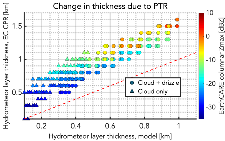
280 Fig. 4. Model hydrometeor layer thickness with EC-CPR PTR convolved vs. model hydrometeor layer thickness without the PTR applied. Colors indicate the Z_{MAX} in the column. Circles represent “cloud+drizzle” profiles and triangles represent “cloud-only” profiles.
