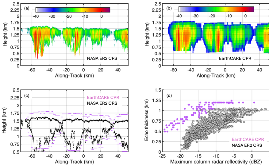
Fig. 6. EarthCARE CPR and collocated NASA ER-2 CRS observations of marine stratus collected on Oct 30 th , 2024, near 121.7° W and 26.6° N. (a) radar reflectivity [dBZ] measured by ER-2 CRS and (b) EarthCARE CPR, respectively. (c) cloud top and base height determined with radar reflectivity from the EarthCARE CPR (purple) and ER2 CRS (black). (d) Hydrometeor layer thickness based on radar echoes vs. the maximum columnar radar reflectivity.
