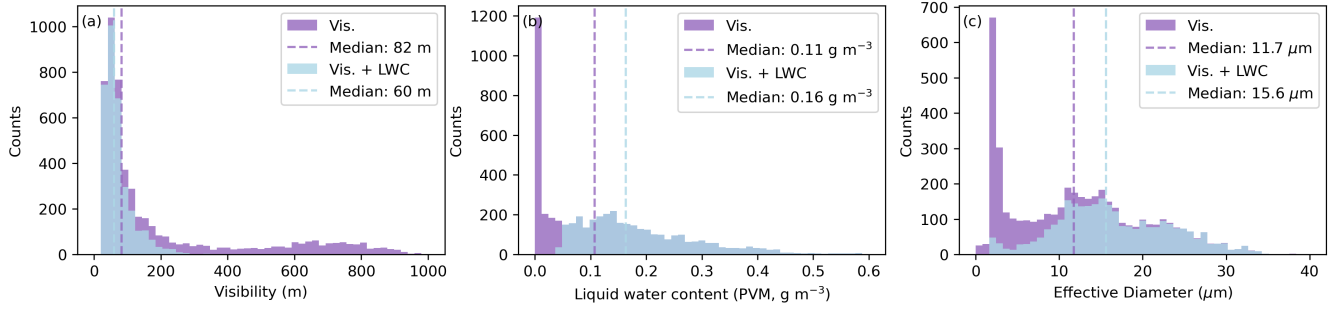
Figure 9. Effect of three different fog definitions applied on fog statistics. The commonly used fog definition ( \text{vis.} < 1 \text{ km} , purple) is compared to the combined definition ( \text{vis.} < 1 \text{ km} + \text{LWC} > 0.05 \text{ g m}^{-3} , light blue). The LWC is based on the PVM measurements.
