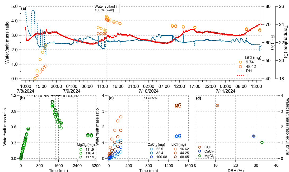
Figure 2: (a) Time series of temperature (T) and relative humidity (RH) inside the SPP reaction chamber, recorded by the Elitech probe, shown alongside water uptake by LiCl samples. (b) Water uptake by MgCl 2 at two different RH setpoints. (c) Water uptake by LiCl and CaCl 2 under constant RH conditions. (d) Equilibrium water-to-salt mass ratio as a function of the salt deliquescence RH (DRH) for the three salts at their highest RH exposure. All water uptake measurements were performed on salts placed in secondary containers within the SPP reaction chamber.
