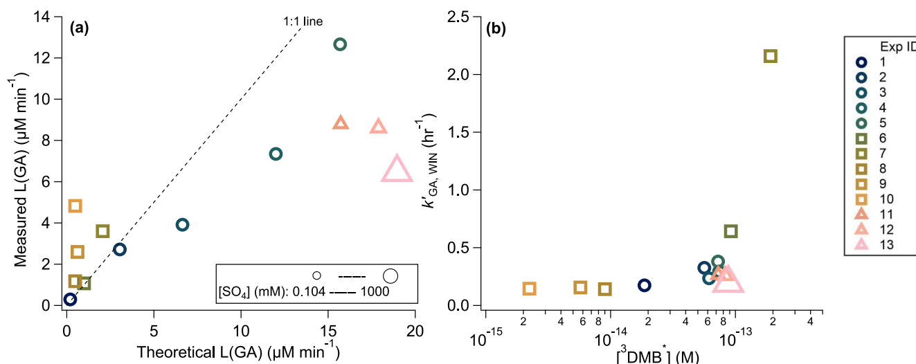
Figure 7: (a) Comparison of the measured vs. theoretical loss rates of GA under various experimental conditions. Marker size reflects the corresponding sulfate concentration, ranging from 0.104 mM to 1000 mM. (b) Pseudo-first order rate constant for GA loss plotted against the calculated steady-state ^3DMB^* concentrations. Experimental conditions are color-coded by experiment ID and shape-coded by experimental grouping (see legend). Additional details on the rate constant and [^3DMB^*] calculations can be found in Supplementary Section S1.
