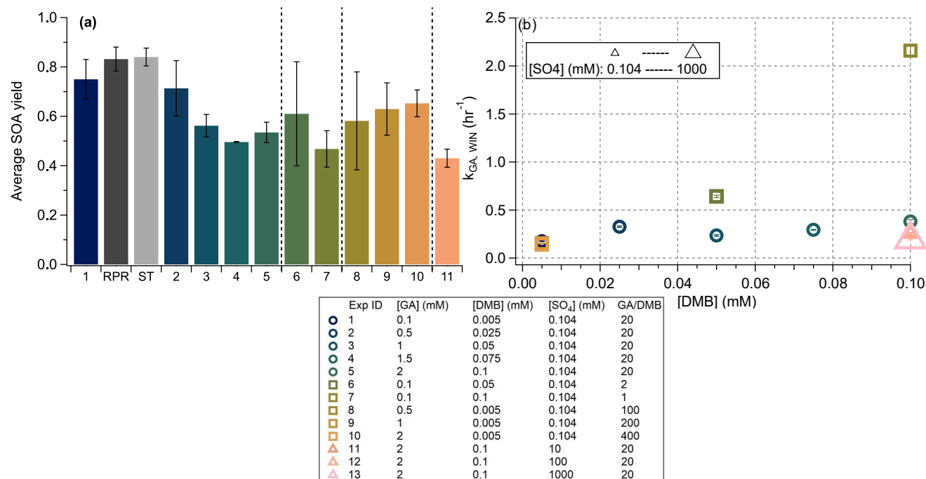
Figure 5: (a) Average SOA yields under different experimental conditions. Yields were calculated over the entire illumination period for each experiment; error bars represent standard deviations. Results from the RPR and ST experiments are displayed adjacent to Experiment 1 for comparison. Experiments 12 and 13 are excluded due to high background organic signal at high [SO 4 2- ], which precluded reliable SOA yield determination. (b) Pseudo-first-order rate constants for GA decay under Davis winter solstice conditions ( k_{GA,WIN} ) for all experiments. Abbreviated reaction conditions are provided in the figure legend with additional details available in Table 1.
