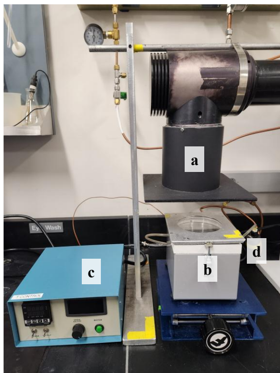
Figure 1: Photograph and schematic diagram of the photochemical experimental setup using the SPP. The photograph displays the setup used for all GA+DMB experiments while the diagram gives the generalized setup applicable to all experiments described in this study. A detailed description of the SPP system and operation is available in Section 3.1.
