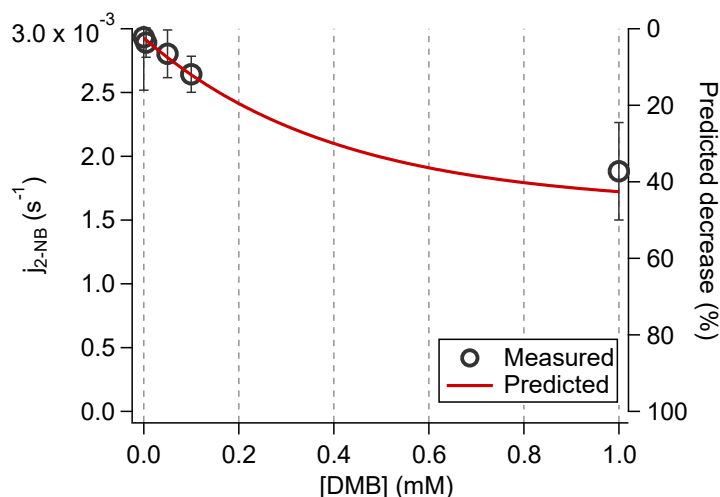
Figure 4: Expected vs. measured decreases in j_{2-NB} in solutions of DMB with a 0.3 cm pathlength. A description of the model used to predict j_{2-NB} can be found in the Supplementary Section S1.
