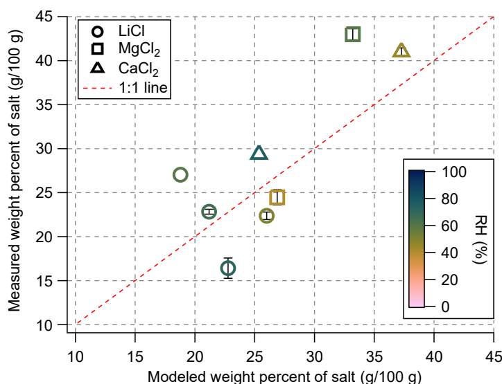
Figure 3: Comparison of measured and predicted values of the weight percent of salt (g-salt/100 g-solution) for LiCl, MgCl 2 , and CaCl 2 across a range of RH conditions. Predicted values were calculated using osmotic coefficient-based water uptake modeling. Data points are averages from replicate experiments and error bars are ± 1 standard deviation.
