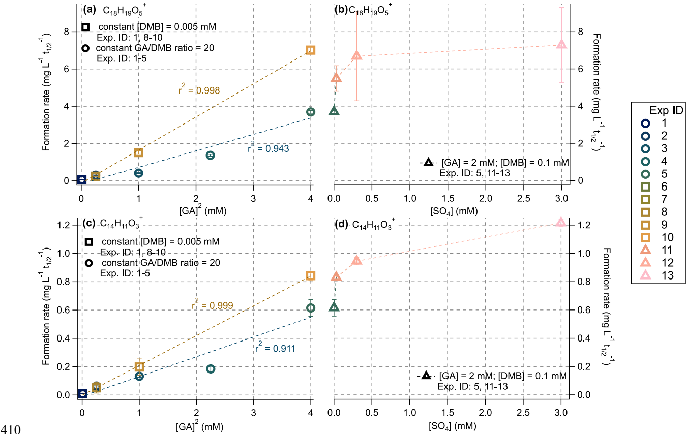
Figure 8: Formation rates of (a, b) C_{18}H_{19}O_5^+ (a major GA dimer tracer ion) and (c, d) C_{14}H_{11}O_3^+ (a likely second-generation product tracer) plotted against either [GA]^2 or ionic strength for several series of experiments (see inset text legend for experiment IDs). Error bars represent propagated uncertainties based on the standard deviations of the fitted coefficients. Reaction conditions are summarized in Table 1 and details regarding the rate-fitting procedures are provided in Section Error! Reference source not found.. All experimental data were fit using single-exponential functions, except for the C_{14}H_{11}O_3^+ in Experiments 11-13, where a linear model was used due to poor exponential fit quality. Time-resolved kinetic data used to obtain the fitted values are shown in Figure S9.
