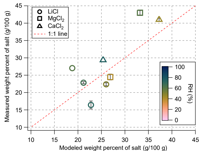
Figure 3: Comparison of measured and predicted values of the weight percent of salt (g-salt/100 g-solution) for LiCl, MgCl 2 , and CaCl 2 across a range of RH conditions. Predicted values were calculated using osmotic coefficient-based water uptake modeling. Data points are averages from replicate experiments and error bars are \pm 1 standard deviation.
