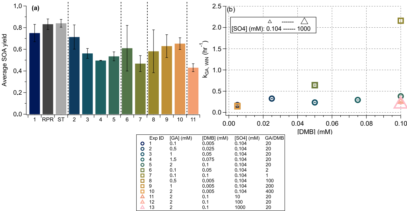
280 Figure 5: (a) Average SOA yields calculated over the entire illumination period for each experiment. Error bars indicate one standard deviation. Results from the RPR and ST experiments are displayed adjacent to Experiment 1 for comparison. Experiments 12 and 13 are excluded due to high background organic signals at high [SO 4 2- ], which precluded reliable SOA yield determination. 285 (b) Pseudo-first-order rate constants for GA decay under Davis winter solstice conditions ( k'_{GA,WIN} ) for all experiments. Abbreviated reaction conditions are summarized in the figure legend, with full details provided in Table 1. In (b), maker colors distinguish experimental conditions: circles represent the base experiments where GA and DMB concentrations varied while maintaining a fixed GA/DMB ratio of 20; squares represent experiments where the GA/DMB ratio was modified (by changing either [GA] 0 or [DMB] 0 ); triangles represent experiments where [SO 4 ] was altered while keeping GA/DMB = 20. The size of each triangle scales with [SO 4 ], allowing visual differentiation of these experiments.
