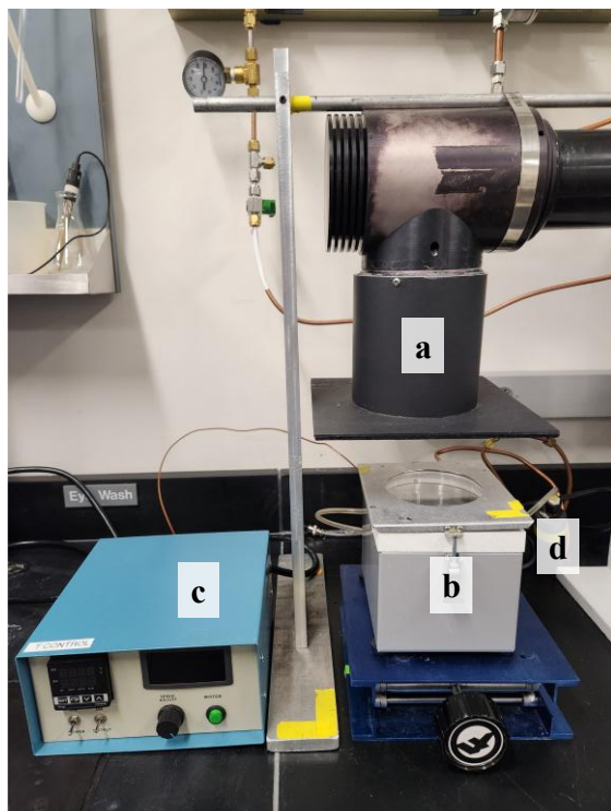
Figure 14: Photograph and schematic diagram of the photochemical experimental setup using the SPP. The photograph displays the setup used for all GA+DMB experiments while the diagram gives the generalized setup applicable to all experiments described in this study. A detailed description of the SPP system and operation is available in Section 0.
