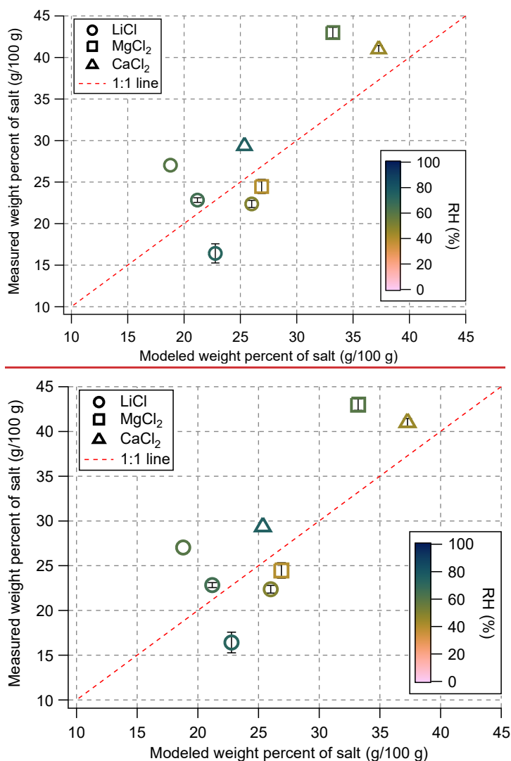
Figure 33: Comparison of measured and predicted values of the weight percent of salt (g-salt/100 g-solution) for LiCl, MgCl 2 , and CaCl 2 across a range of RH conditions. Predicted values were calculated using osmotic coefficient-based water uptake modeling. Data points are averages from replicate experiments and error bars are \pm 1 standard deviation.
