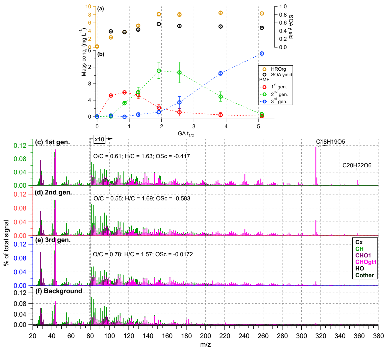
Figure 6: Time series data for Experiment 7 ( [GA]_0 = 0.1 mM, [DMB]_0 = 0.1 mM, [SO_4^{2-}]_0 = 0.104 mM), showing (a) evolution of total organic concentration and SOA yield and (b) the four-factor PMF solution, showing the evolution of distinct generations of GA-derived aqSOA. Data points are the averages from multiple samples, with error bars indicating the corresponding standard deviations. The HRMS for the PMF solution are shown in (c-f).
