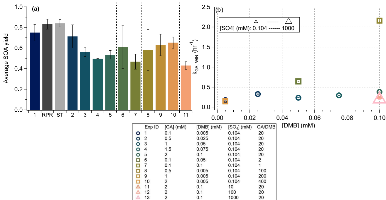
285 Figure 55: (a) Average SOA yields under different experimental conditions. Yields were calculated over the entire illumination period for each experiment; error bars indicate one standard deviation. Results from the RPR and ST experiments are displayed adjacent to Experiment 1 for comparison. Experiments 12 and 13 are excluded due to high background organic signal at high [SO 4 2- ], which precluded reliable SOA yield determination. (b) Pseudo-first-order rate constants for GA decay under Davis winter solstice conditions ( k_{GA, WIN} ) for all experiments. Abbreviated reaction conditions are
