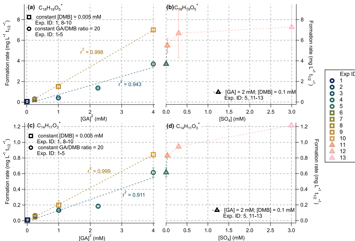
Figure 8: Formation rates of (a, b) C_{18}H_{19}O_5^+ (a major GA dimer tracer ion) and (c, d) C_{14}H_{11}O_3^+ (a likely second-generation product tracer) plotted against either [GA]^2 or ionic strength for several series of experiments (see inset text legend for experiment IDs). Error bars represent propagated uncertainties based on the standard deviations of the fitted coefficients. Reaction conditions are summarized in Table 1 and details regarding the rate-fitting procedures are provided in Section Error! Reference source not found.. All experimental data were fit using single-exponential functions, except for the C_{14}H_{11}O_3^+ in Experiments 11-13, where a linear model was used due to poor exponential fit quality. Time-resolved kinetic data used to obtain the fitted values are shown in Figure S9S8.
