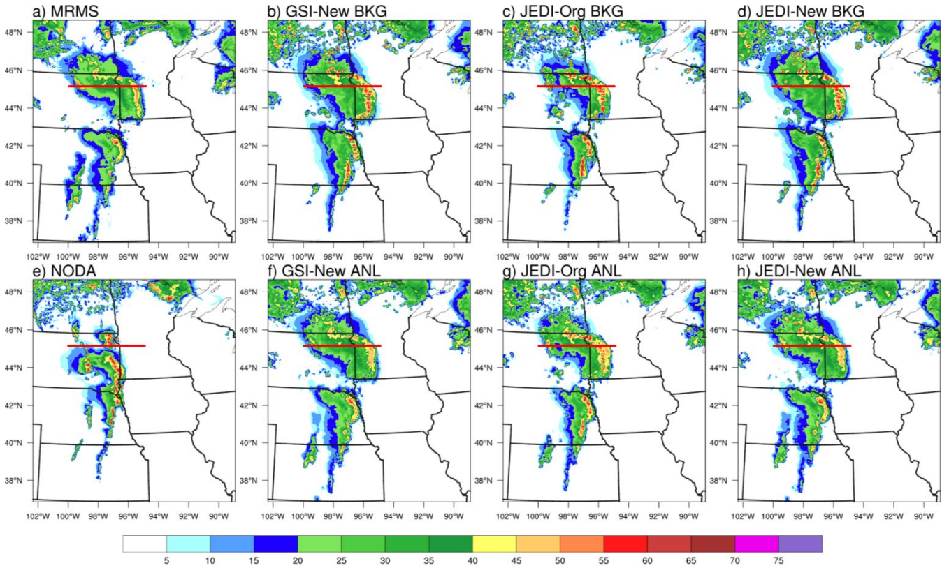
Figure 5. The composite reflectivity at final analysis time (00 UTC on May 13, 2022) from (a) MRMS observations, (b) GSI-New background, (c) JEDI-Org background, (d) JEDI-New background, (e) NODA forecast, (f) GSI-New analysis, (g) JEDI-Org analysis, and (h) JEDI-New analysis. The red line in each panel indicates the location of the vertical cross sections shown in Figs. 6 and 7. Because no data assimilation is performed in NODA, no analysis field is available for that experiment.
