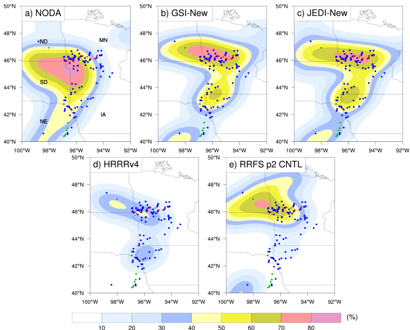
Figure 12. Neighborhood probability (%) (shaded) of 2-hr maximum updraft helicity exceeding 75 m 2 s -2 from 00 to 02 UTC on May 13, 2022 from the forecasts of a) NODA, b) GSI-New, c) JEDI-New, d) HRRRv4 and e) RRFS p2 CNTL. The red, green, and blue dots denote the SPC reports of tornado, hail, and wind, respectively.
