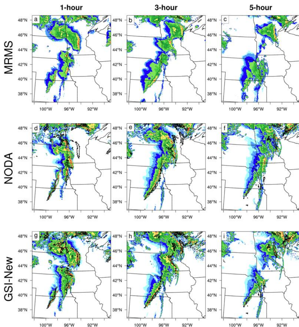
Figure 8. Composite reflectivity forecasts and observations at 1, 3, and 5 h lead times, valid at 0100, 0300, and 0500 UTC 13 May 2022, respectively. Rows show MRMS observations, NODA, GSI-New, JEDI-New, HRRRv4, and RRFS p2 CNTL, and columns show the 1-, 3-, and 5-h forecasts. In the forecast panels, the observed 40-dBZ composite reflectivity contour is overlaid in black.
