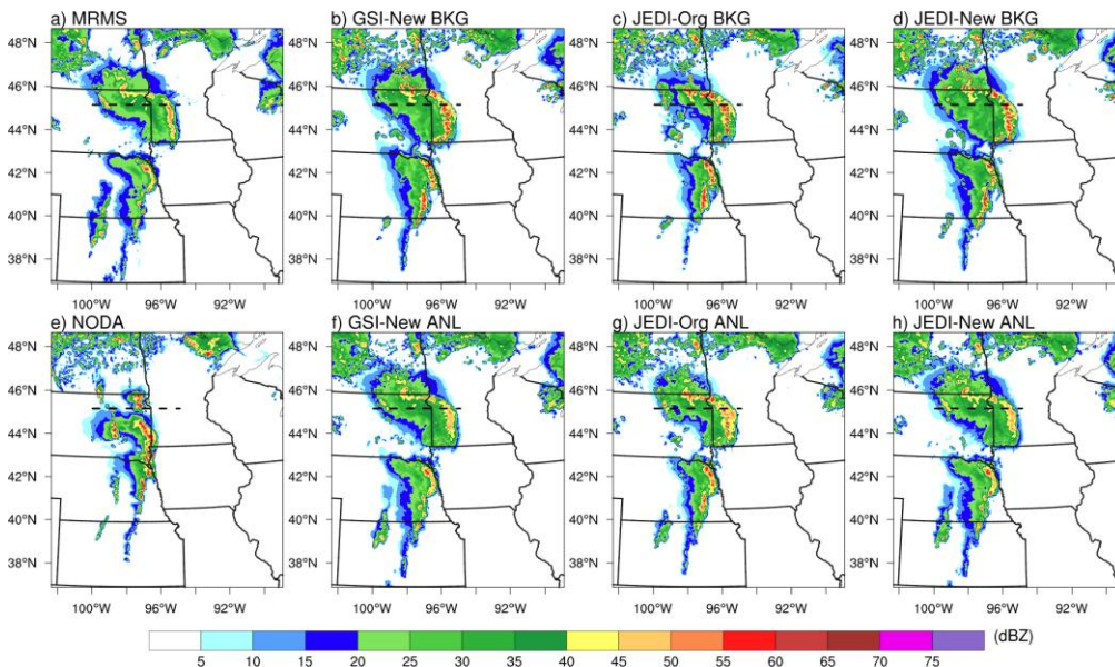
Figure 5. The composite reflectivity at final analysis time (00 UTC on May 13, 2022) from the observation and background forecasts and the analyses of the NODA, GSI En3DVar and JEDI En3DVar experiments . The dashed lines inside the panels show the locations of vertical cross sections shown in Figs. 6 and 7. (a) MRMS observations, (b) GSI-New background, (c) JEDI-Org background, (d) JEDI-New background, (e) NODA forecast, (f) GSI-New analysis, (g) JEDI-Org analysis, and (h) JEDI-New analysis. The dashed line in each panel indicates the location of the vertical cross sections shown in Figs. 6 and 7. Because no data assimilation is performed in NODA, no analysis field is available for that experiment.
