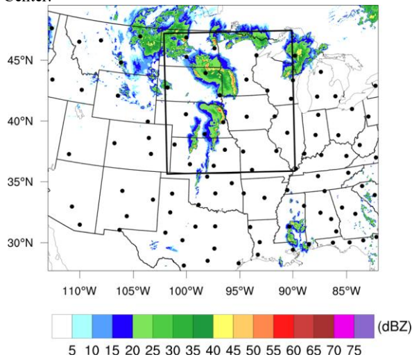
220 Figure 2. MRMS composite reflectivity (dBZ) at 0000 UTC 13 May 2022, over the FV3-LAM model domain. The bold black box marks the verification domain, and WSR-88D radar locations are indicated by black dots.
