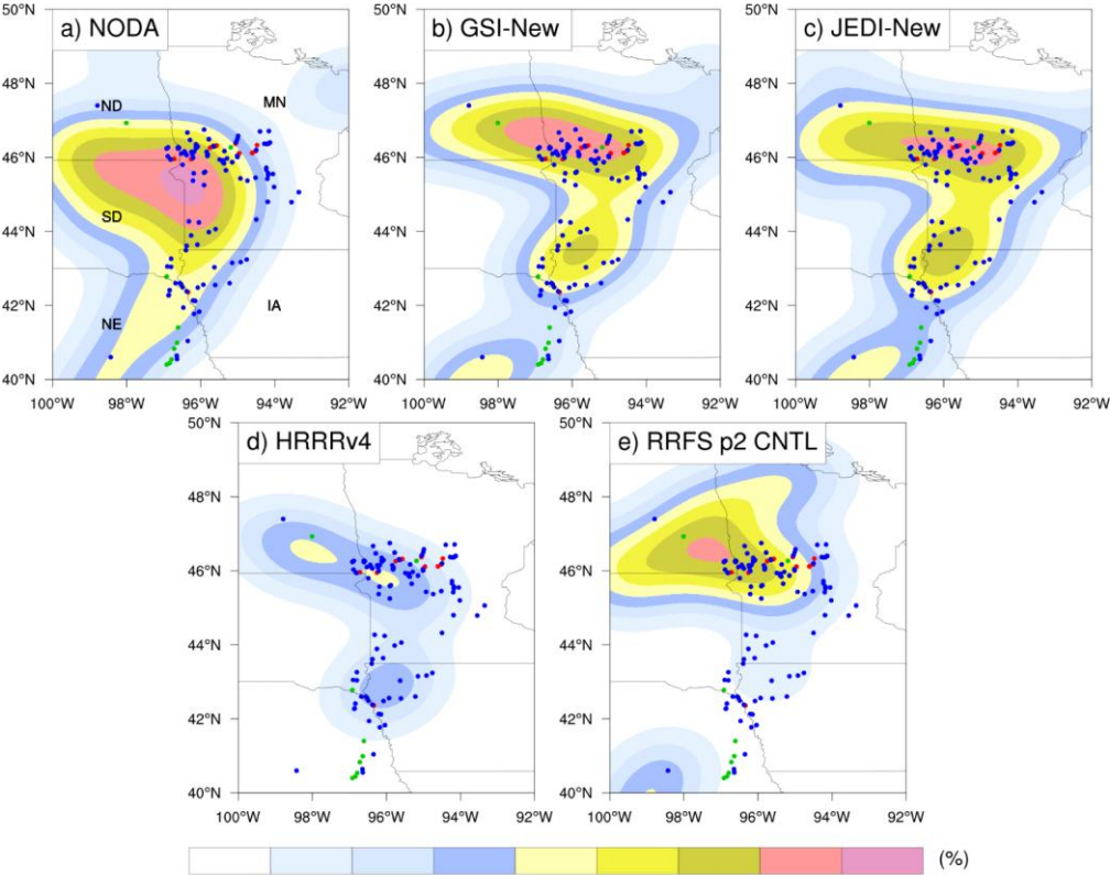
Figure 12. Neighborhood probability (%; shaded) of 2-hr maximum updraft helicity exceeding 75 m2 s-2 from 00 to 02 UTC on May 13, 2022 from the forecasts of a) NODA,
