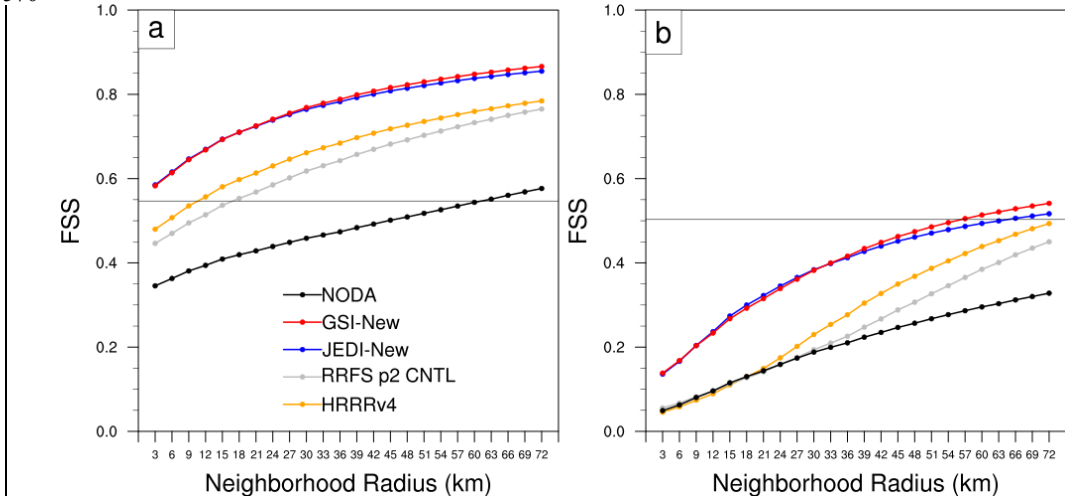
Figure 10. Fractions skill scores (FSS) of hourly composite reflectivity averaged over a 6-h verification period, shown as a function of neighborhood radius (km) for reflectivity thresholds of (a) 25 dBZ and (b) 45 dBZ. Verification is performed against MRMS
