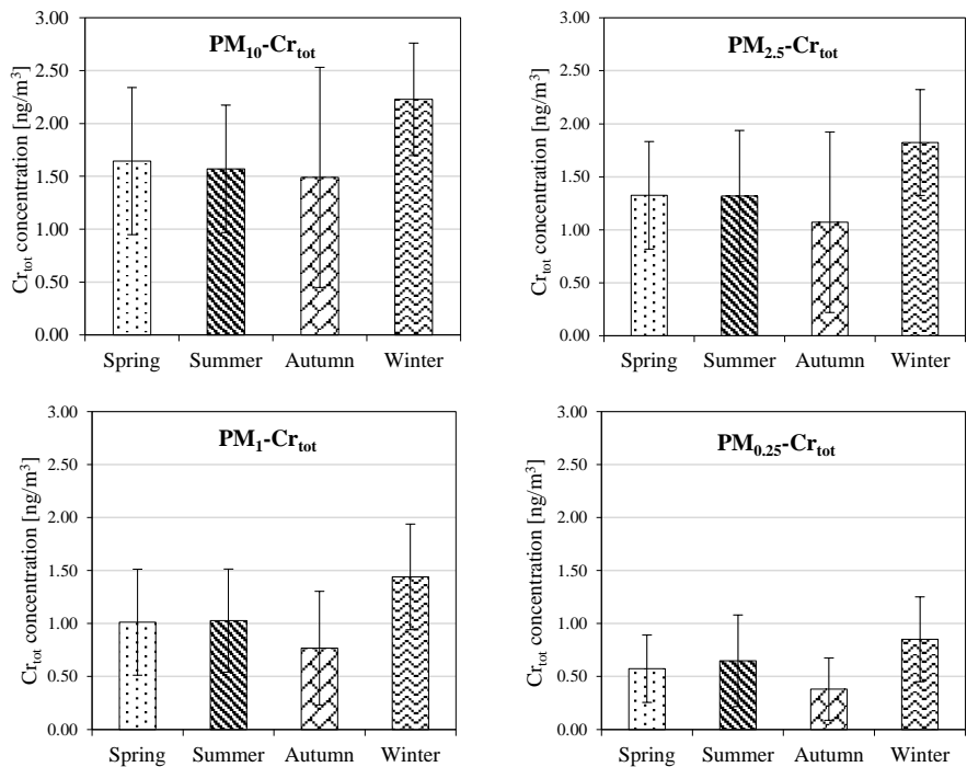
Figure 1. The concentrations of pseudo-total chromium in PM_{10} , PM_{2.5} , PM_1 and PM_{0.25} depending on the seasons.
