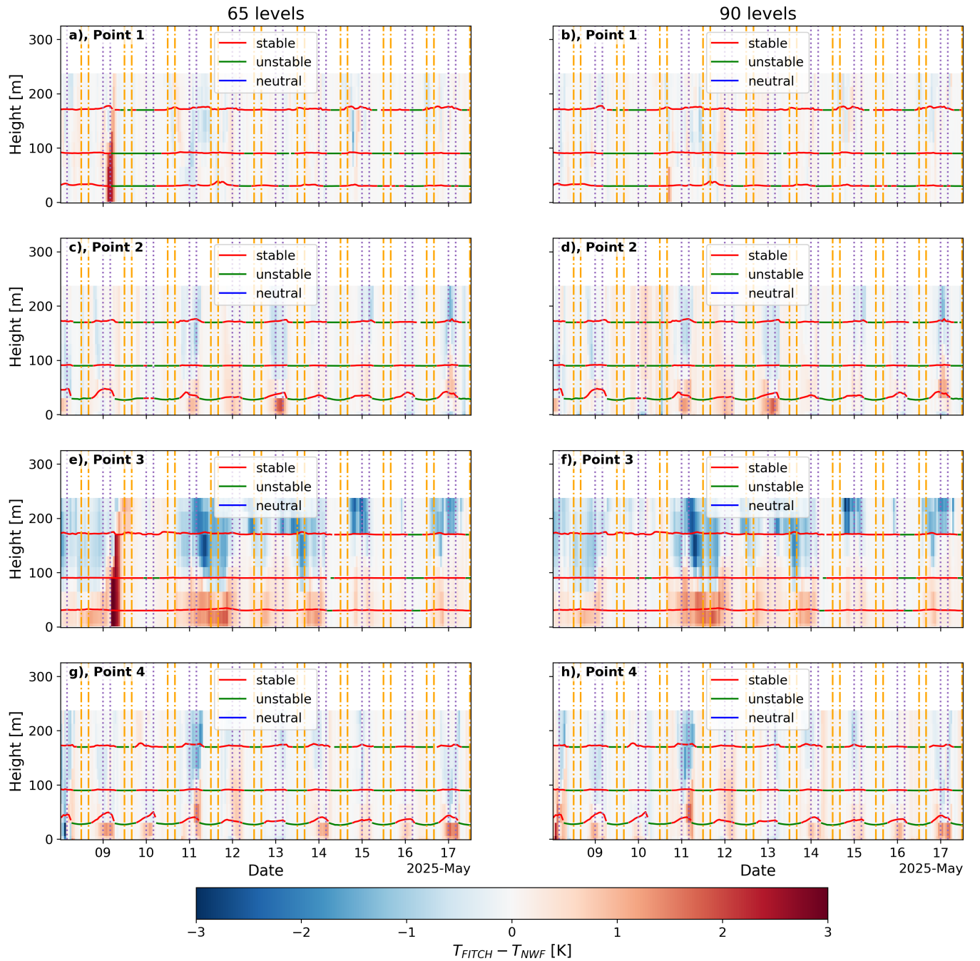
Figure 21. Timeseries of temperature profile difference of FITCH minus NWF for four points (rows) highlighted in Figure 20 for the (a,c,e,g) 65 levels and (b,d,f,h) 90 levels. The background color shows the temperature difference at each altitude and date. The horizontal lines highlight the color-coded virtual potential temperature gradient ( \gamma )-derived stability for three heights (10 m – 50 m, 80 m – 100 m and 140 m – 200 m) and shown at the center of these layers. Purple dotted vertical lines highlight periods used for night-time averages (00:00–04:00 UTC) and orange dash-dotted vertical lines highlight day-time average periods (12:00–16:00 UTC).
