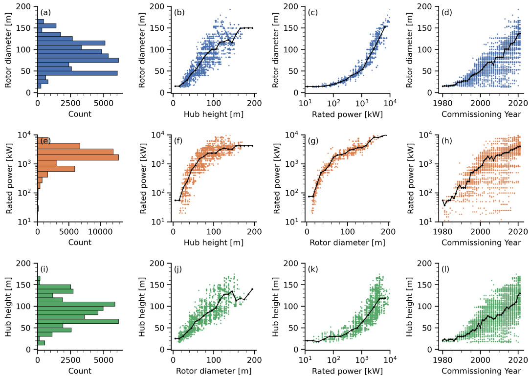
Figure 5. Rotor diameter, rated power and hub height distributions and relationships in the turbine dataset. Top, middle, and bottom rows represent each variable. First column (plots a, e, i) displays histograms; Middle plots (b, c, f, g, j, k) illustrate co-variation between variables: rotor diameter with hub height and rated power; rated power with hub height and rotor diameter; and hub height with rotor diameter and rated power. Last column (plots d, h, l) show variation over commissioning year. Black lines indicate median values within variable bins.
