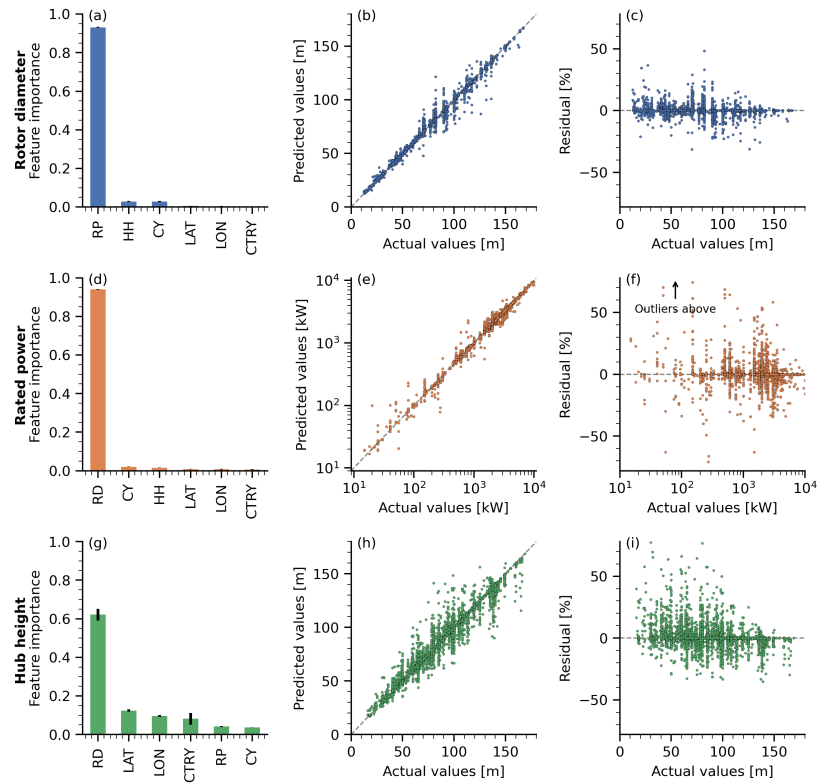
Figure 6. Feature importance and model evaluation for gap-filling models of rotor diameter, rated power, and hub height. (a, d, g): Feature importance of explanatory variables—rotor diameter (RD), hub height (HH), rated power (RP), commissioning year (CY), country (CTRY), latitude, and longitude (LAT and LON). Bars represent the mean and standard deviation of feature importance estimated by MDI across 100 random forest estimators. (b, e, h): Scatter plots of actual versus predicted values. (c, f, i): Model residuals (errors) in percent relative to actual values.
