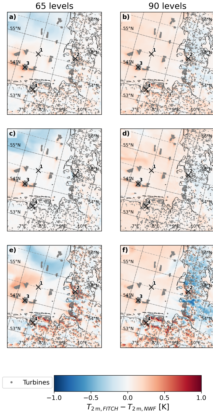
Figure 20. 2-m temperature difference for FITCH-NWF for (a,c,e) 65 levels and (b,d,f) 90 levels averaged (a,b) over the full week 08.05.–17.05.2025 and (c,d) over day-time (12:00 - 16:00 UTC) and (e,f) over night-time conditions (00:00 - 04:00 UTC) only. Turbines are shown as gray dots, and the four crosses highlight locations used in Figure 21.
