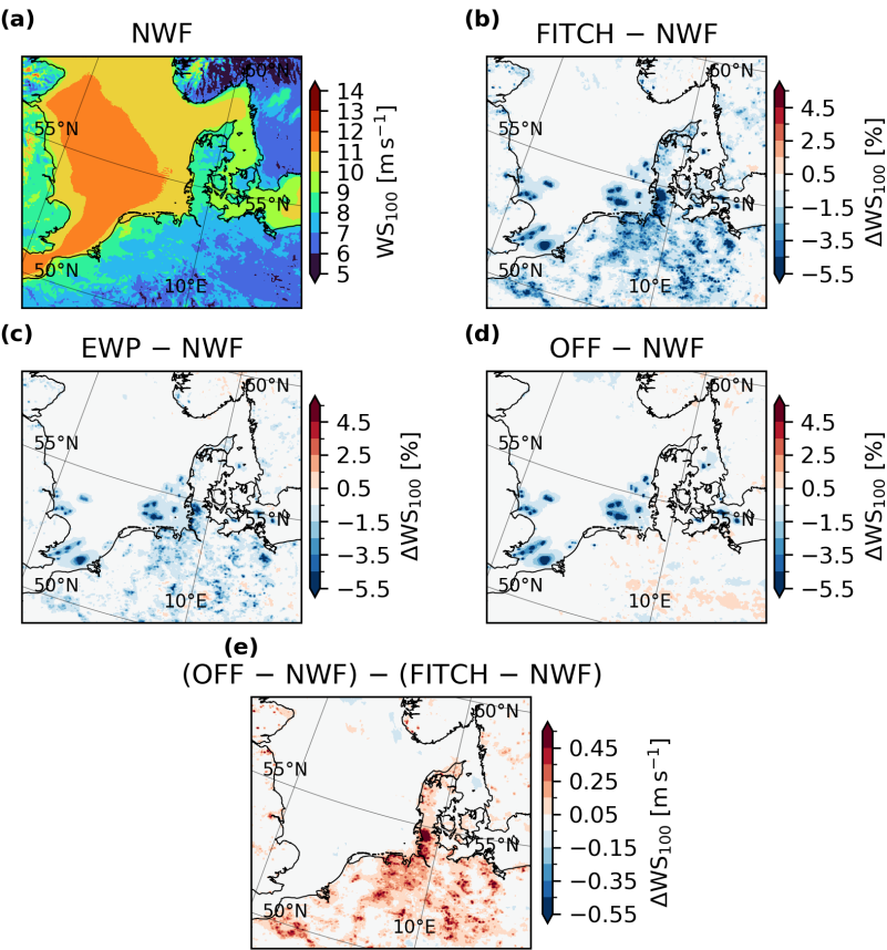
Figure 15. (a) Average wind speed at a height of 100 m height for February 2020 and August 2022 for the simulation without wind farms (NWF) and normalized difference with respect to NWF to simulations with (b) FITCH WFP, (c) EWP WFP, (d) FITCH WFP for offshore turbines only and (e) the absolute difference between (d) and (b), but shown in absolute numbers as zoom into the North Sea and Danish Baltic.
