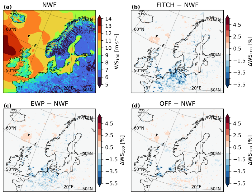
Figure 14. (a) Average wind speed at a height of 100 m height for February 2020 and August 2022 for the simulation without wind farms (NWF) and normalized difference with respect to NWF to simulations with (b) FITCH WFP, (c) EWP WFP and (d) FITCH WFP for offshore turbines only.
