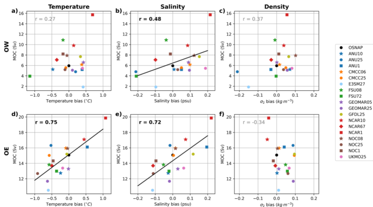
940 Figure 18. Scatter plots of the upper-ocean (0-700 m) and section average, time-mean (a, d) temperature, (b, e) salinity, and (c, f) \sigma_2 density biases against the time-mean maximum transports in \sigma_2 space at OW (top panels) and OE (bottom panels). The black dots in each panel show the OSNAP transports plotted against no bias. The LR, MR, and HR simulations are indicated by squares, circles, and stars, respectively. NCAR67 is shown as a diamond. The correlation coefficients (excluding OSNAP) are included in each panel with the bold font indicating statistical significance at the 95% confidence level, calculated using a 2-sided Student's t-test. The regression lines are also shown in panels with statistically significant 945 correlations.
