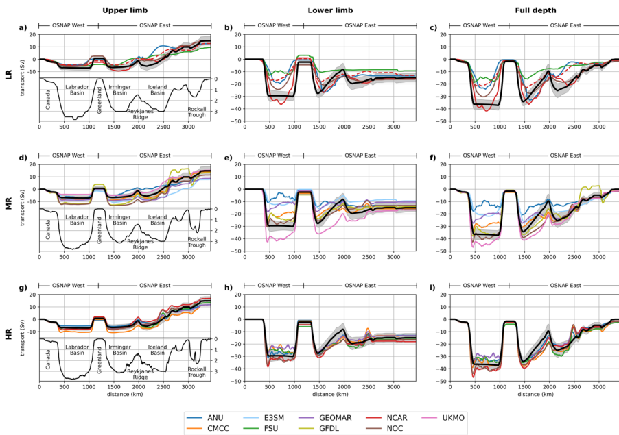
655 Figure 7. Time-mean west-to-east cumulative transports across the OSNAP sections for the (a, d, g) upper limb, (b, e, h) lower limb, and (c, f, i) full depth. The upper, middle, and bottom rows are for LR, MR, and HR, respectively. The solid black lines show the OSNAP transports with gray shading indicating \pm 1 monthly standard deviation. The positive and negative slopes indicate northward and southward transports, respectively. Typical representations of the topographic features for each grid resolution from one of the respective models are also provided in the left panels with depth given on the right y-axis in km.
