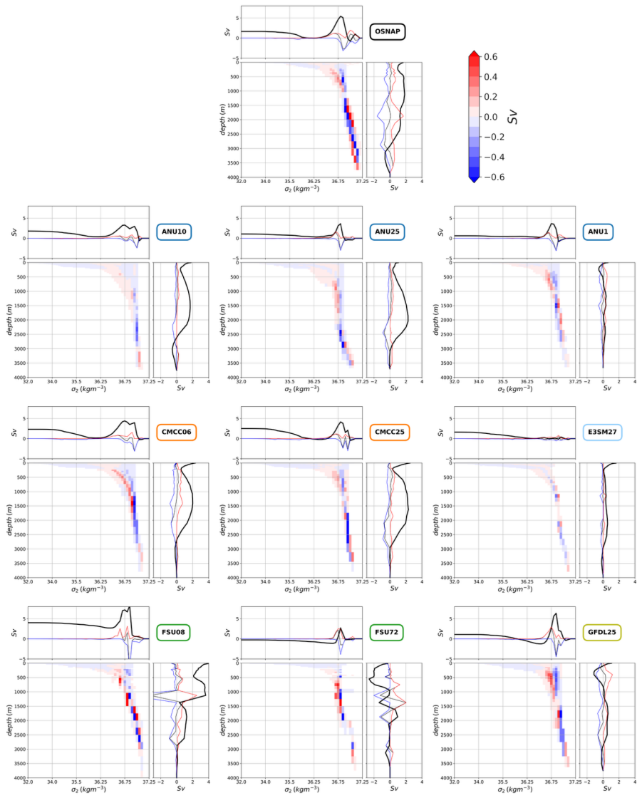
Figure 8. Time-mean transports at OW in depth and density ( \sigma_2 ) space from OSNAP and from ANU10, ANU25, ANU1, CMCC06, CMCC25, E3SM27, FSU08, FSU72, and GFDL25. In each set, the bottom left panels show southward (blue) and northward (red) transports in Sv. The
