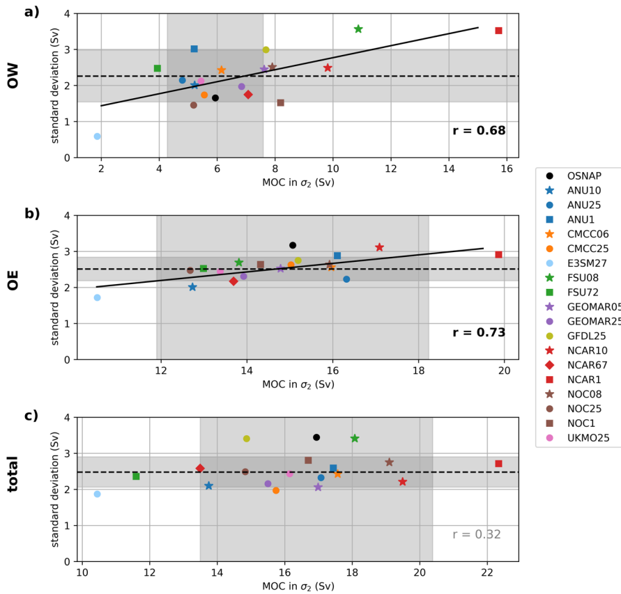
800 Figure 13. Scatter plots of time-mean maximum transports vs. their monthly standard deviations (SDs) in \sigma_2 space for (a) OW, (b) OE, and (c) total. The horizontal dashed lines show the respective ensemble mean SDs with shading indicating their \pm 1 SDs. The vertical shaded areas indicate \pm 1 SD ranges for OSNAP maximum transports. The LR, MR, and HR simulations are indicated by squares, circles, and stars, respectively. NCAR67 is shown as a diamond. The correlation coefficients (excluding OSNAP) are included in each panel with the bold font 805 indicating statistical significance at the 95% confidence level, calculated using a 2-sided Student's t-test. The regression lines are also shown for (a, b) with statistically significant correlations.
