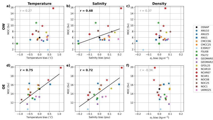
940 Figure 18. Scatter plots of the upper-ocean (0-700 m) and section average, time-mean (a, d) temperature, (b, e) salinity, and (c, f) \sigma_2 density biases against the time-mean maximum transports in \sigma_2 space at OW (top panels) and OE (bottom panels). The black dots in each panel show the OSNAP transports plotted against no bias. The LR, MR, and HR simulations are indicated by squares, circles, and stars, respectively. NCAR67 is shown as a diamond. The correlation coefficients (excluding OSNAP) are included in each panel with the bold font indicating statistical significance at the 95% confidence level, calculated using a 2-sided Student's t-test. The regression lines are also shown in panels with statistically significant correlations. 945
