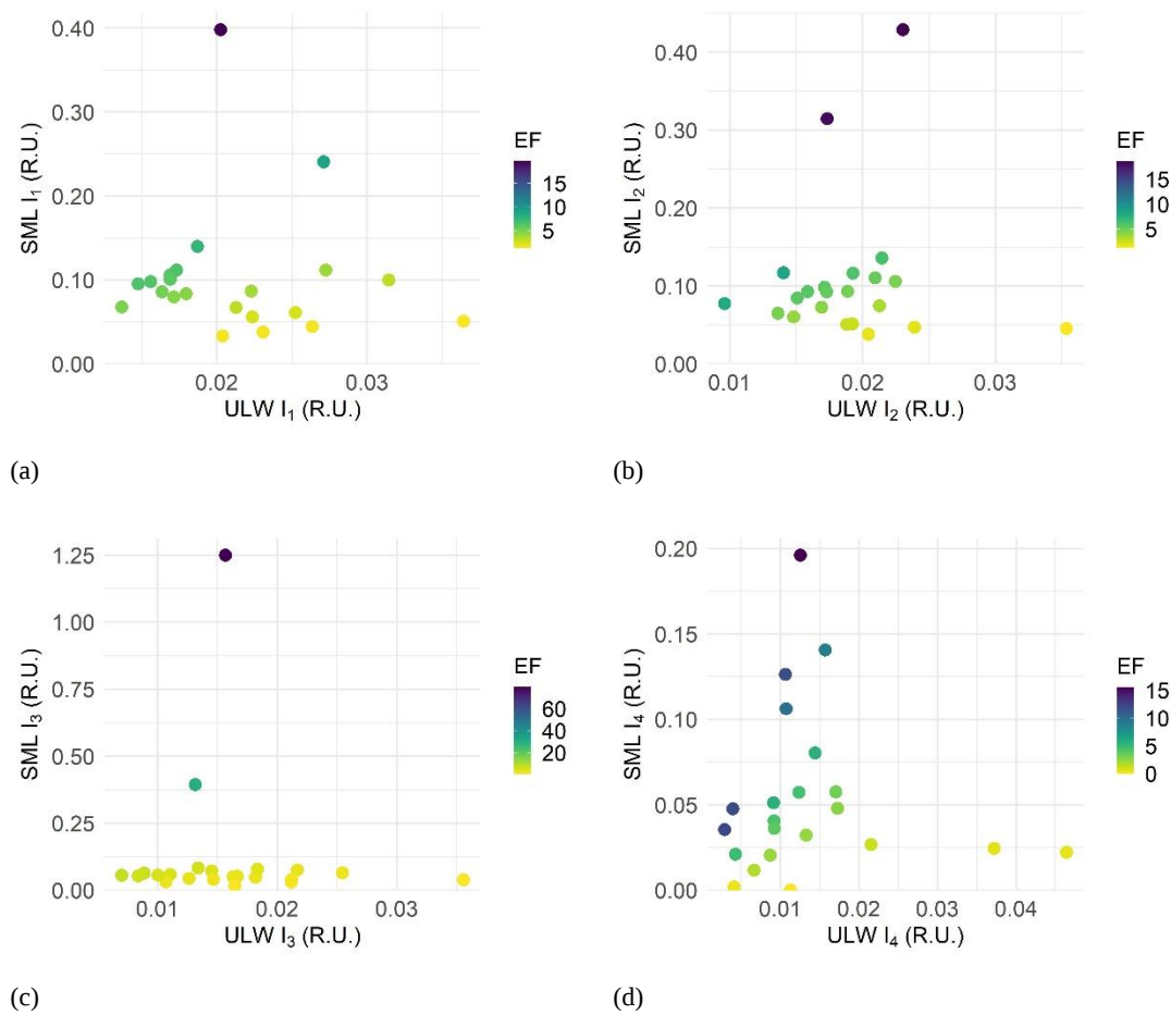
Figure 6: Correlation graphs between the SML (y axis) and ULW (x axis) of PARAFAC maximum fluorescence intensities (R.U.) of (a) I 1 ; (b) I 2 ; (c) I 3 ; (d) I 4 . The z axis illustrates the enrichment factors
