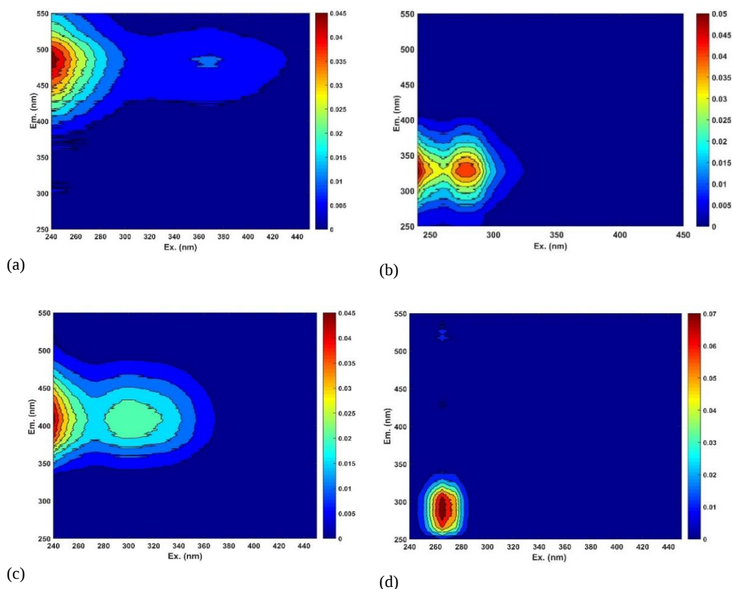
Figure 5: The four components resolved in the SML and ULW by the seawater PARAFAC model, (a) Component C1, peaks A-C, (b) Component C2, peak T, (c) Component C3, peaks A-M, (d) Component C4, peak B
