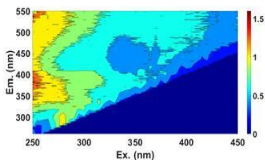
Figure 7: The FDOM/CDOM index (R.U.·m) in the (a) SML, (b) ULW, (c) the ratio (\text{FDOM/CDOM})_{\text{sml}} / (\text{FDOM/CDOM})_{\text{ulw}} . (a,b) Depletion of the fluorescence intensity excited in the UV-A / near-visible range is apparent in the SML relative to the ULW. (c) Higher contribution of FDOM excited at short wavelength (UV-C/UV-B) to CDOM is apparent in the SML
