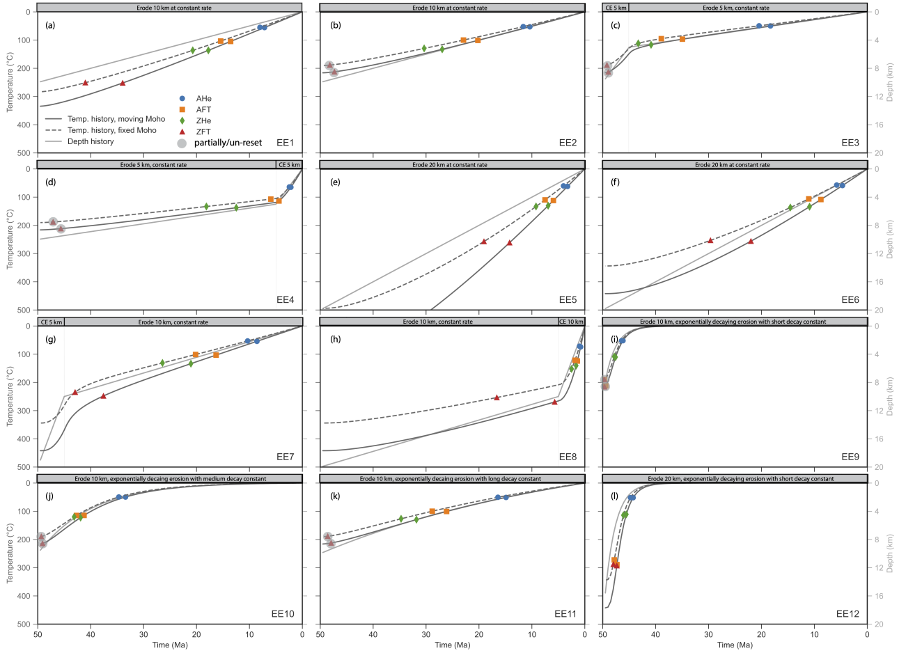
Figure 3. Erosional exhumation models—, for which volumetric heat production is set at "average", or 1 \mu\text{W} \cdot \text{m}^{-3} , unless otherwise specified: (a) —model EE1, in which 10 km is eroded at a constant rate over 50 Myr, and volumetric heat production is set at "high", or 2 \mu\text{W} \cdot \text{m}^{-3} ; (b) model EE2, same erosion as (a) but average volumetric heat production; (c) model EE3, in which 5 km is eroded in the first 5 Myr and an additional 5 km is eroded over 45 Myr; (d) model EE4, in which 5 km is eroded in the first 45 Myr, and an additional 5 km is eroded in the final 5 Myr; (e) model EE5, in which 20 km is eroded at a constant rate over 50 Myr, and volumetric heat production is "high"; (f) model EE6, same erosion as (e) but average volumetric heat production; (g) model EE7, in which 10 km is eroded in the first 5 Myr and an additional 10 km is eroded in the final 5 Myr; (h) model EE8, in which 10 km is eroded in the first 45 Myr, and an additional 10 km is eroded in the final 5 Myr; (i) model EE9, in which 10 km is eroded over 50 Myr at an exponentially-decaying rate using a short decay constant, and volumetric heat production is set to high; (j) model EE10, in which 10 km is eroded over 50 Myr at an exponentially-decaying rate using a medium decay constant; (k) model EE11, in which 10 km is eroded over 50 Myr at an exponentially-decaying rate using a long decay constant, and finally (l) show results for models EE1–EE12 model EE12, respectively in which 20 km is eroded over 50 Myr at an exponentially-decaying rate using a short decay constant. Parameters varied in each model are also described in Table 1.
