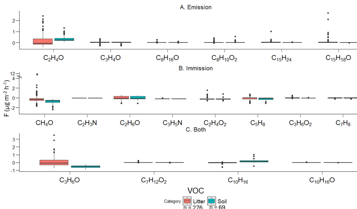
Figure 3. Measured VOC fluxes (in \mu\text{g m}^{-2} \text{h}^{-1} ) during the field campaign for A. Major emitted compounds, B. Major immitted compounds and C. Both emitted and immitted compounds for litter chambers and bare soil chambers. The line that divides the box represents the median of measured fluxes, ends of the box indicate the upper (Q3) and lower (Q1) quartiles, up and down whiskers represent max and min values and outliers are represented by dots. VOC fluxes for this figure were obtained from the 24-h measurements of 12 soil covered by litter samples (276 VOC flux measurements) and 3 bare soil samples (69 flux measurements).
