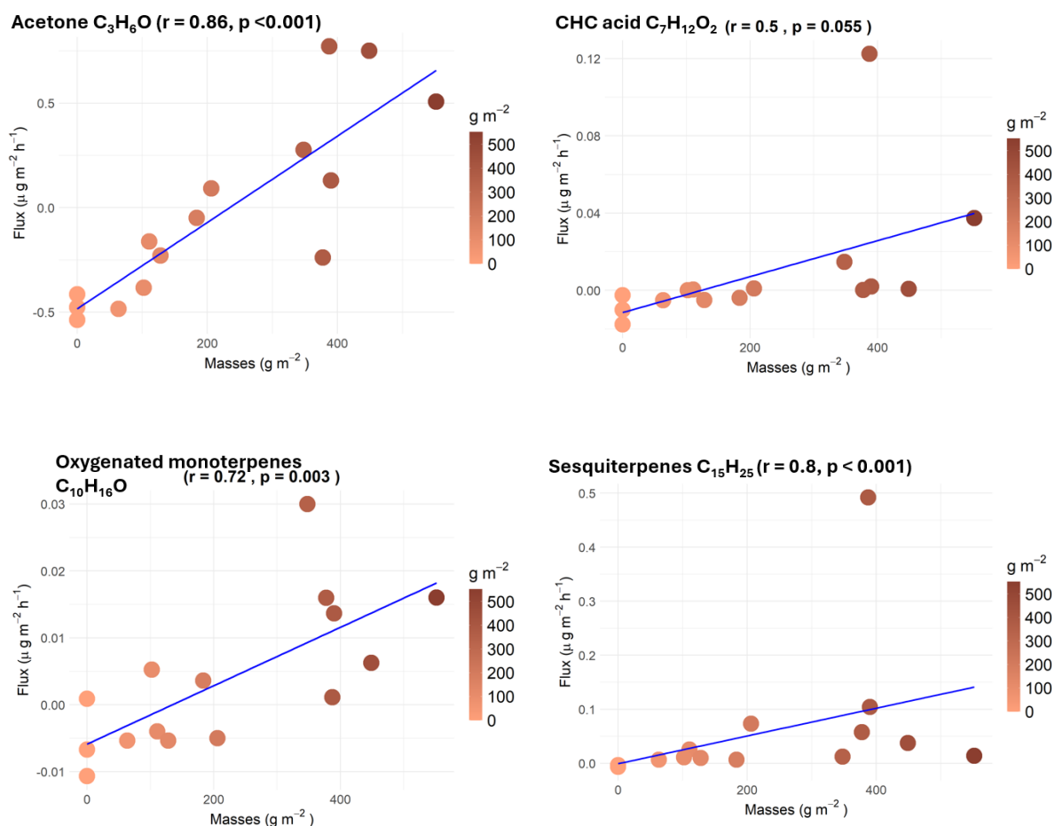
Figure 4. Correlation plots of methanol, acetaldehyde, acetone, oxygenated monoterpenes, CHC acid and sesquiterpenes fluxes ( \mu\text{g m}^{-2} \text{h}^{-1} ) with litter masses per area (0 in bare soil in \text{g m}^{-2} ).
