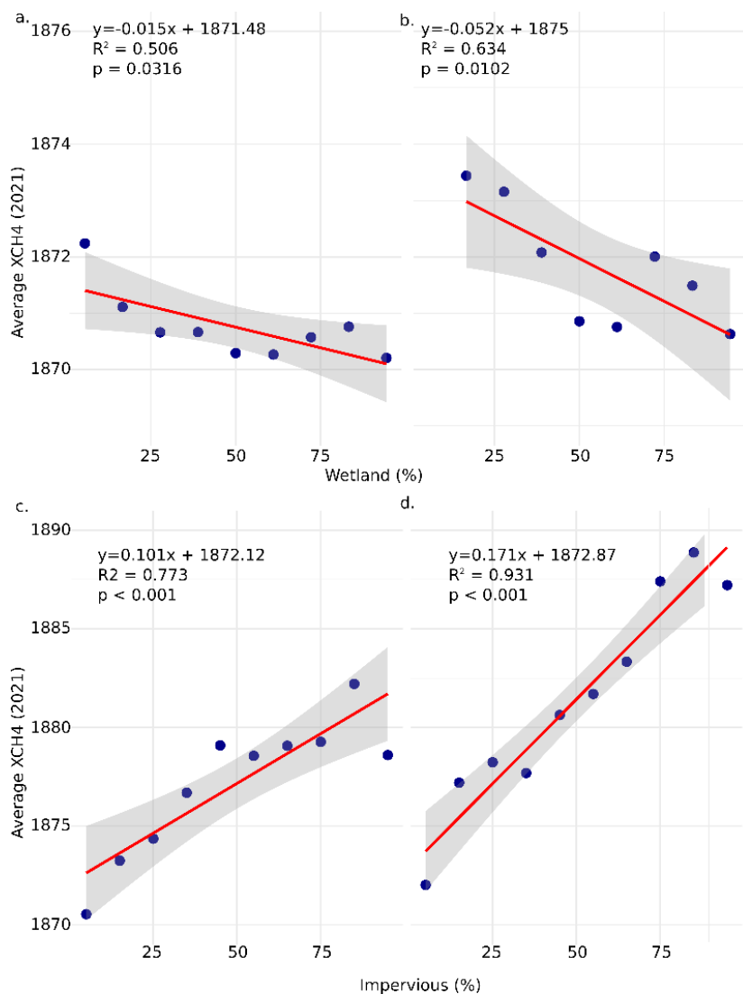
300 Figure 6: a. The linear relationship of average XCH 4 to wetland extent bins for non-gas fields. b. The linear relationship of average XCH 4 to wetland extent bins for gas fields. c. The linear relationship of average XCH 4 to impervious surface extent bins for non-gas fields. d. The linear relationship of average XCH 4 to impervious surface extent bins for gas fields.
