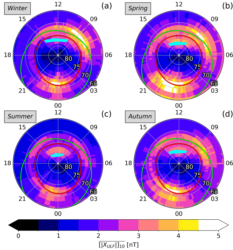
Figure 4. Polar plots of the average 10-minute [X_{ULF}]_{10} amplitudes for different seasons (a) winter (Nov–Jan), (b) spring (Feb–Apr), (c) summer (May–Jul), and (d) autumn (Aug–Oct). The Feldstein model is represented by red (polar boundary) and green (equatorward boundary) lines. The statistical location of the cusp is marked with a cyan-coloured area computed using the equations set forth by Anderson and Bukowski (2024).
