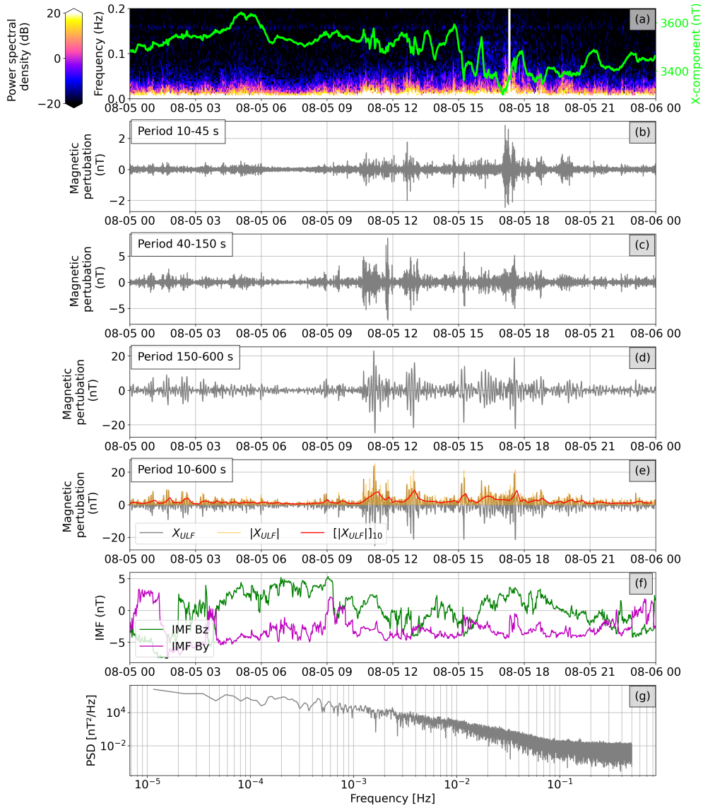
Figure 1. (a): Plot of the spectrum at TAB on the 5th of August 2022, where the green curve represents the magnetic northward component (X). (b)–(d): outputs of a bandpass filter in the period range stated in the top left corner for Pc 3 (b), Pc 4/Pi 2 (c), and Pc 5 (d). (e): The output of the bandpass filter, used in the paper ( X_{ULF} ), the absolute values ( |X_{ULF}| ), and the 10-minute smoothed signal ( [|X_{ULF}|]_{10} ). (f): IMF parameters for the given date. (g): The power spectral density w.r.t. frequency for the given day at TAB.
