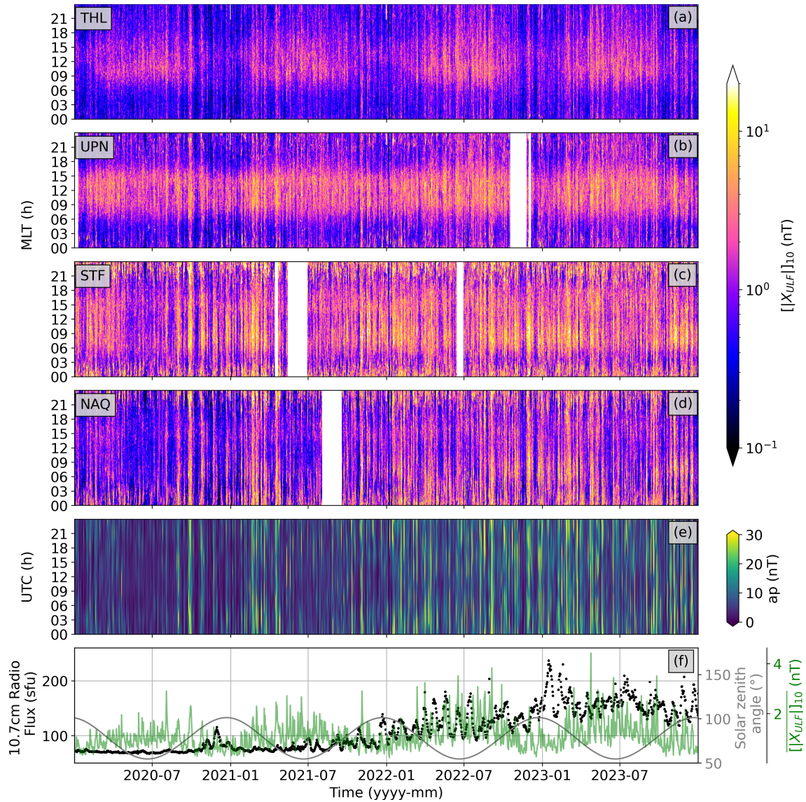
Figure 2. (a)–(d): [X_{ULF}]_{10} at the four stations THL, UPN, STF, and NAQ for four years, as a function of MLT. (e): Geomagnetic activity ap index as a function of UTC. (f): The daily average ULF signal measured at THL (green), the solar zenith angle (grey), and the daily solar flux F10.7 (black).
