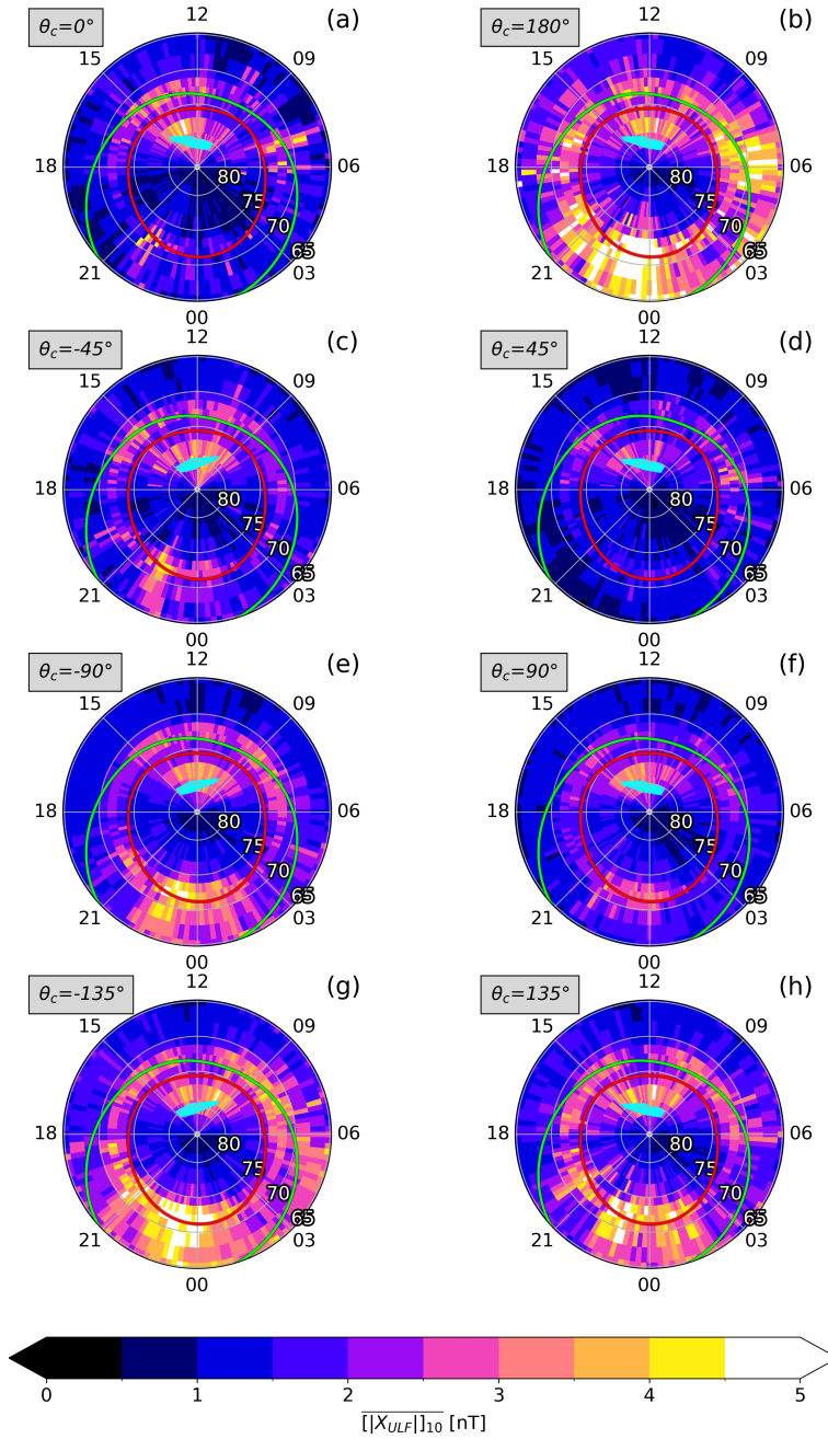
Figure 3. Average \overline{[X_{ULF}]}_{10} amplitudes during summer (May–July) in 2020–2023 for the Greenland west-coast magnetometer chain with respect to QD-latitude and MLT for different IMF clock angles ( \theta_c ). The green and red curves represent the equatorward and poleward boundaries of the auroral oval, respectively, as computed from the Feldstein model. The statistical location of the cusp is marked with a cyan-coloured area computed using the equations set forth by Anderson and Bukowski (2024).
