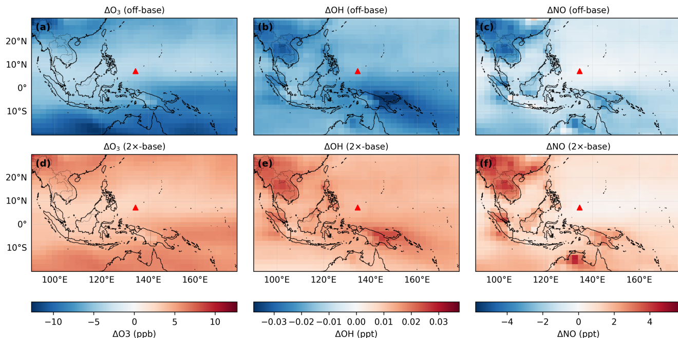
Figure 6. Tropospheric ozone Differences in tropospheric column-averaged mole fractions of O_3 , OH, and NO dry-air between LNO x sensitivity simulations and the base simulation. (a–c) the differences between the no-NO x simulation and hydroxyl radical the base simulation (OH no NO x minus base) column, and (d–f) from GEOS-Chem simulations with lightning the differences between the 2× NO x emissions included (a, d; "normal"), without lightning emissions (b, e; "control"), simulation and difference between "control" and "normal" (e and f), averaged over the study period. Panels base simulation (e) and (f) show differences (control-2× NO x minus normal) base). Columns correspond to O_3 , highlighting the impact of lightning on regional tropospheric ozone and OH distributions, and NO from left to right. The red triangle indicates marks the location of the Palau FTIR measurement site. The absolute value of the simulation results are shown in Appendix C, Fig. C1.
