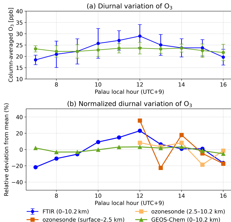
Figure 3. (a) Diurnal variation of tropospheric column of O 3 (TOC) from FTIR measurement and GEOS-Chem (smoothed with averaging kernels). Error bars denote \pm 1\sigma variability within each hourly bin. (b) Normalized diurnal variation of O 3 from FTIR TOC, GEOS-Chem, and ozonesonde volume mixing ratios from surface – 2.5 km and 2.5–10.2 km. Normalized values are calculated relative to the mean of each dataset (see Sect 2.5.1). Absolute values of ozonesonde hourly mean are shown in Appendix ??.
