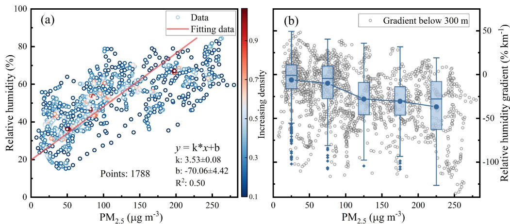
Figure 11. Relationships between PM_{2.5} concentrations and (a) relative humidity, and (b) its vertical gradient.
