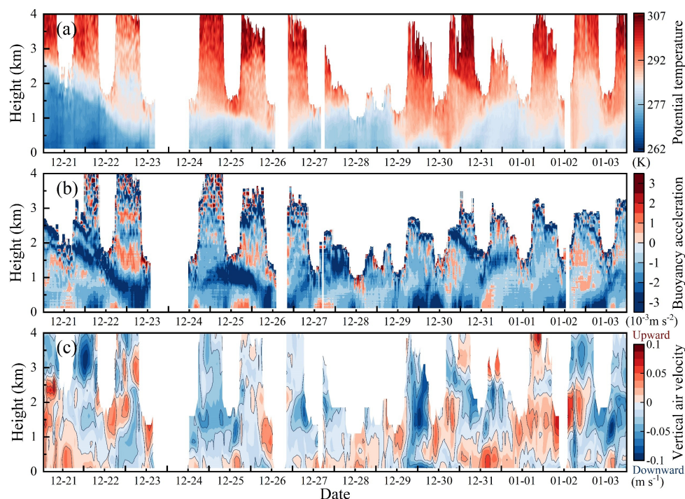
Figure 6. Spatiotemporal distributions of potential temperature, buoyancy acceleration, and vertical velocity: (a) potential temperature; (b) buoyancy acceleration; (c) vertical velocity.
