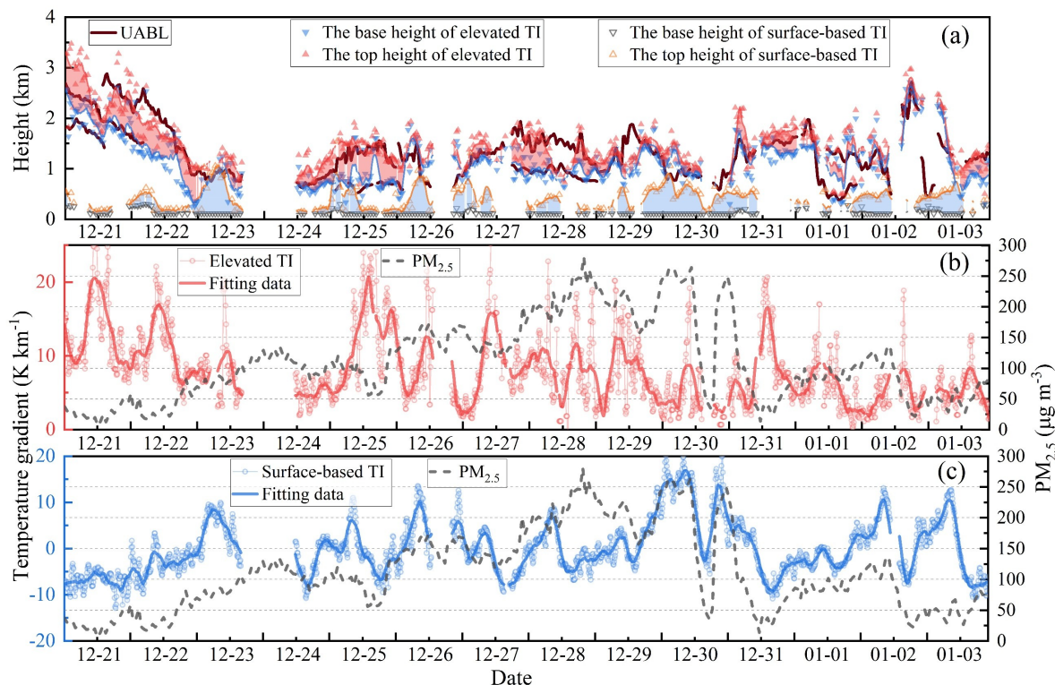
Figure 12. TI characteristics and aerosol boundary layer distribution. (a) Vertical distribution of the UABL and TIs. The black solid line indicates the UABL. The red shaded area represents the elevated TI layer, with red upward-pointing triangles and blue downward-pointing triangles indicating the top and base heights of the elevated TI, respectively. The blue shaded area represents the surface-based TI layer, with orange upward-pointing triangles and black downward-pointing triangles indicating the top and base heights of the surface-based TI, respectively. (b, c) Black dashed lines represent PM_{2.5} concentrations, while red and blue solid lines show the mean vertical temperature gradients of the elevated and surface-based TIs, respectively.
