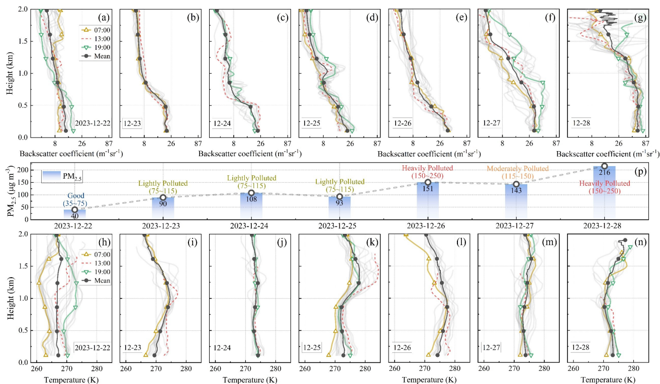
Figure 7. Vertical distributions of aerosols and temperature from 22 to 28 December. Panel (p) shows the daily mean PM 2.5 concentrations. Gray solid lines indicate hourly vertical profiles of backscatter coefficient and temperature. Yellow solid lines with upward-pointing triangles, green solid lines with downward-pointing triangles, and red dashed lines correspond to observations at 07:00, 19:00, and 13:00 local time, respectively. Black dotted lines represent daily mean values.
