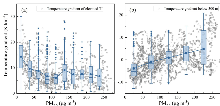
Figure 14. Relationships between PM 2.5 concentrations and the temperature gradients of (a) the elevated TI and (b) the surface-based TI.
