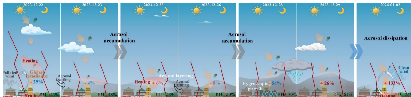
Figure 16. Aerosol accumulation and dissipation during the pollution development. The gray shading indicates the aerosol layer. Orange downward arrows represent downward radiative flux, and green upward arrows indicate the reflected component. The red solid line denotes the temperature profile.
