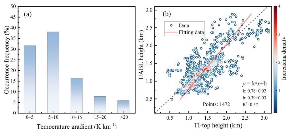
Figure 13. Characteristics of the elevated TI. (a) Frequency of temperature gradient occurrence; (b) Relationship between the UABL and the top height of the elevated TI.
