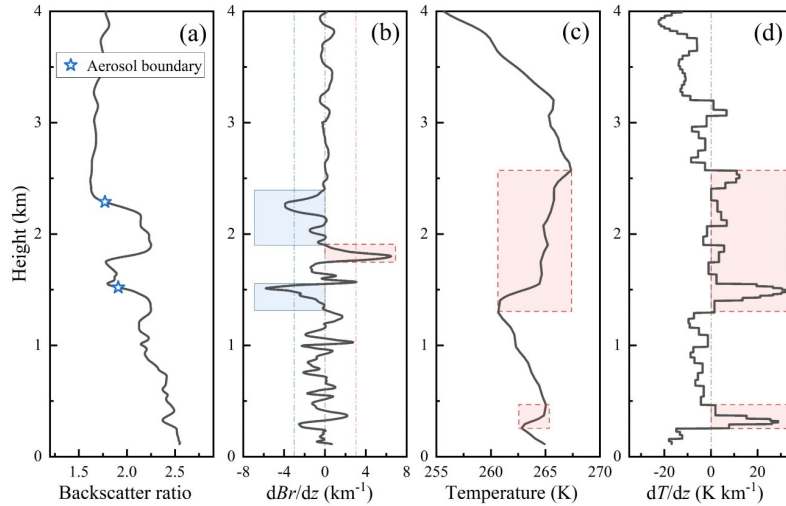
Figure 2. Extraction of UABL and TI characteristics. Panels (a)-(d) show (a) BR, (b) BR gradient, (c) temperature, and (d) temperature gradient. In panels (a)-(d), the black curves represent the BR, BR gradient, temperature, and temperature gradient, respectively. Asterisks indicate the identified aerosol layer boundaries. In panel (b), the blue solid and red dashed shaded regions denote NIBR and PIBR, respectively. In panels (c) and (d), the red dashed shaded regions highlight the TI layers.
