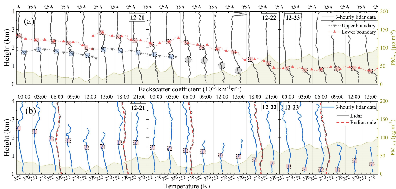
Figure 8. The early stage of aerosol accumulation. Panels (a) and (b) show the backscatter coefficient and temperature, respectively. In panel (a), black solid lines represent the backscatter coefficient, and dashed lines indicate the UABL layers, with shaded dashed boxes highlighting the UABL heights. When aerosol stratification occurs, red upward-pointing triangles and black downward-pointing triangles correspond to the upper and lower UABLs, respectively. In panel (b), the blue solid line represents the temperature, while red dashed lines and black solid lines correspond to lidar measurements and radiosonde observations, respectively. Shaded dashed boxes indicate the locations of TI layers. The yellow shaded regions represent the magnitudes of PM_{2.5} concentrations.
