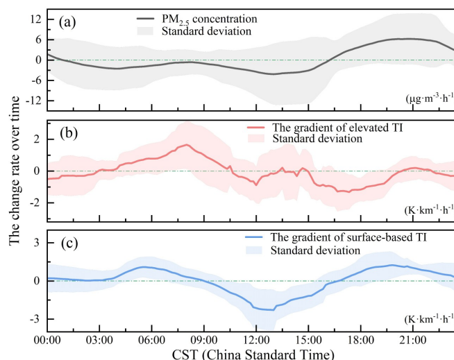
Figure 15. Diurnal rates of change for (a) \text{PM}_{2.5} concentrations, (b) elevated TI temperature gradient, and (c) surface-based TI temperature gradient.
