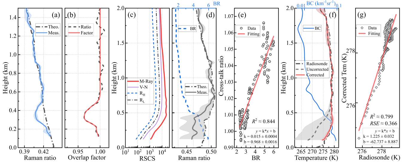
Figure 2. Aerosol backscatter coefficient–Atmospheric temperature correction. (BC) (a) Measured (blue solid) and temperature retrieval theoretical (black dash-dotted) rotational Raman ratios. Panels (ab) Overlap-related quantities, including the measured ratio (black dashed) \tau , and the overlap function (red solid) \omega . (c) Range-square-corrected signals from the elastic (Mie–Rayleigh; thick red solid), while-nitrogen vibrational Raman (thin purple solid), and high- and low-quantum-number rotational Raman (black dash-dotted and blue dashed) channels. (d) \tau -Backscatter ratio (blue dash-dotted) and rotational Raman ratios (measured ratio, black solid; theoretical ratio, black dash-dotted). (e) show Linear regression between the backscatter ratio (BR) and the cross-talk ratio. (f) Backscatter coefficient (BC) and temperature profiles derived from lidar measurements and radiosonde observations. The black solid-dash-dotted line represents BC, and denotes the blue-dashed radiosonde temperature, while the red solid \tau - and black-dash-dotted-blue dashed lines correspond to represent the uncorrected temperature profile, the corrected temperature profile, and the radiosonde-uncorrected lidar temperature profiles, respectively. Shaded areas indicate the corresponding uncertainties. (g) Linear regression between radiosonde and lidar temperatures.
