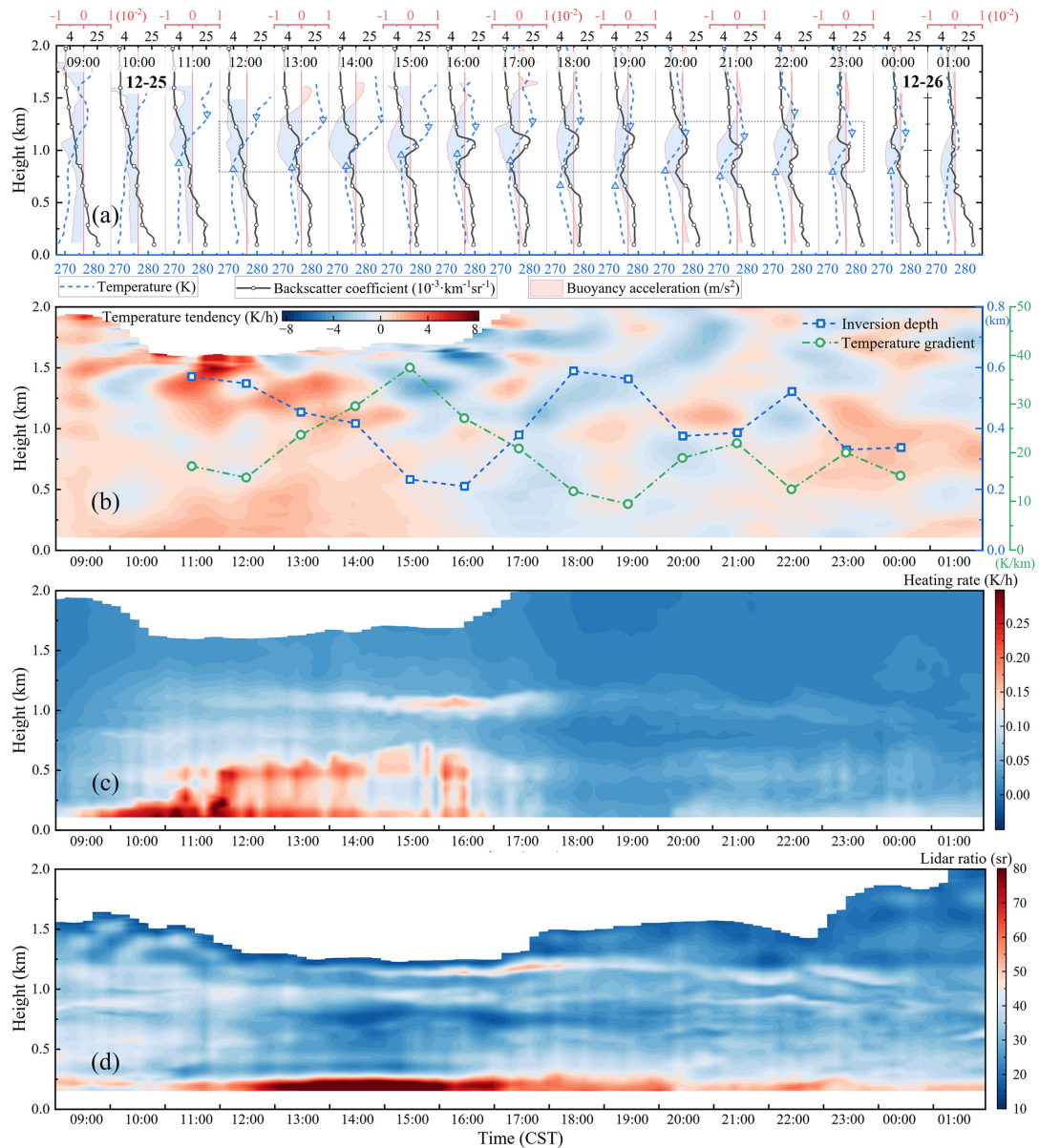
Figure 10. Vertical evolution of the vertical structure and atmospheric buoyancy on 25 December. Panels (a)–(d) show the vertical structures of aerosol and temperature structure, buoyancy acceleration, aerosol heating rate, and lidar ratio (b355 nm) presents the buoyancy acceleration, respectively. In panel (a), the black circular line with circle markers represents the aerosol backscatter coefficient, while the blue dashed line and shaded areas represent the temperature profile and buoyancy acceleration, respectively. The blue (red) shading indicates corresponding to negative (positive) buoyancy acceleration, corresponding to values and downward (upward) buoyant motion. Upward- and downward-pointing triangles are used to indicate the TI layer. In panel (b), the green dotted line shows the variation in temperature gradient, and while the blue square-dotted-dash-dotted line with square markers represents the TI depth.
