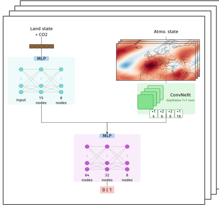
Figure 3. Diagram of the Combined Model. Includes a simple MLP for the Land-State plus a ConvNeXt model for the Atmosphere state, which are then combined using a final MLP that does the binary classification. An ensemble of 20 members is used during training to add robustness and treat the model’s epistemic uncertainty.
