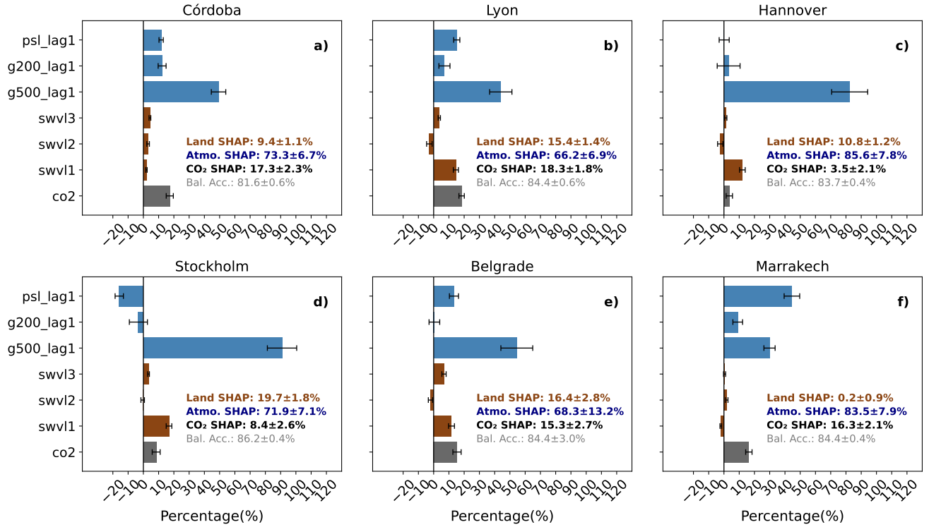
Figure 5. Extreme class prediction mean SHAP value percentage for all locations using the CombinedModel taking the 50% most confident predictions. The x-axis represents the percentage contribution of each feature relative to the total sum of mean absolute SHAP values. Error bars indicate the Standard Error of the Mean (SEM) derived from the 20-member ensemble, representing the uncertainty across different model initializations. The colored text box provides the aggregated percentage contributions for Land and Atmospheric components, as well as the CO 2 contribution, with associated ensemble uncertainties ( \pm SEM). The box also includes the balanced accuracy of the model is also indicated .
