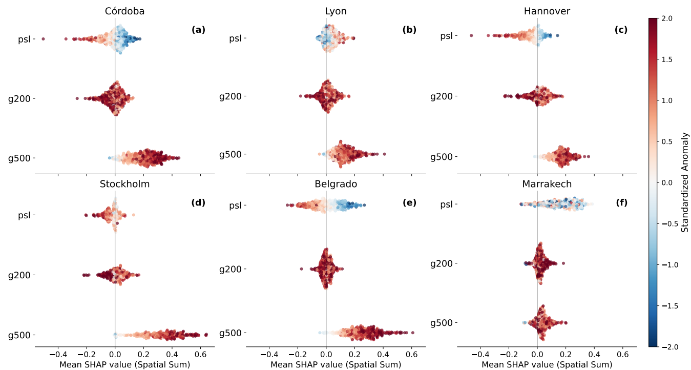
Figure D1. Same plot as in Fig. 6 but for the atmospheric circulation features. We sum up the SHAP values and averaged the standardized anomalies of the circulation variables in a 400km by 400km region surrounding the target location.
