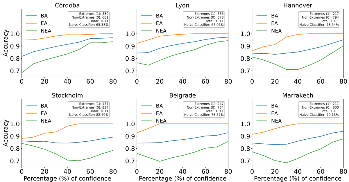
Figure B2. Change in accuracies for the Combined Model for different percentages of confidence using the 90th percentile extreme definition. In the x-axis the percentage of confidence taken, and in the y-axis the accuracies. EA, NEA and BA in the legend stand for extreme accuracy, non-extreme accuracy and balanced accuracy respectively. The text box shows the sample size and the random chance of the naive classifier.
