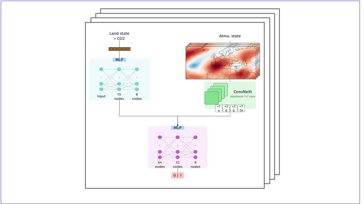
Figure 3. Diagram of the Combined Model. Includes a simple MLP for the Land-State plus a ConvNeXt model for the Atmosphere state, which are then combined using a final MLP that does the binary classification. An ensemble of 20 members is used during training to add robustness and treat the model’s epistemic uncertainty.
