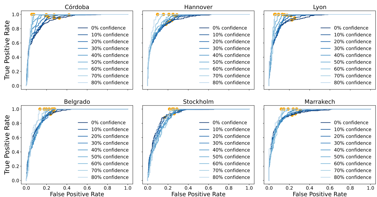
Figure B3. Change in ROC curves for the Combined Model for different percentages of confidence using the 90th percentile extreme definition. In the x-axis the false positive rate and in the y-axis the true positive rate. The legend shows the different percentages of confidence taken.
